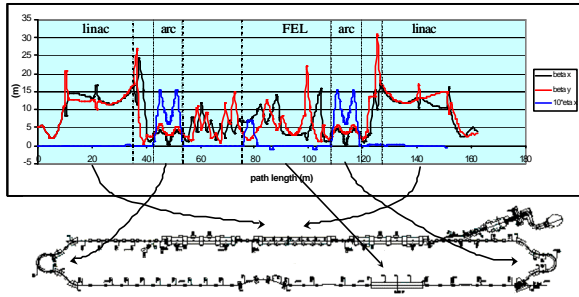
Figure 2: Lattice Functions in IR Upgrade
