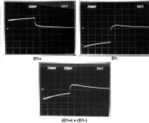
Fig 5. Oscillograms showing bug signals generated from a 1 cm offset of the center conductor of the test fixture.
