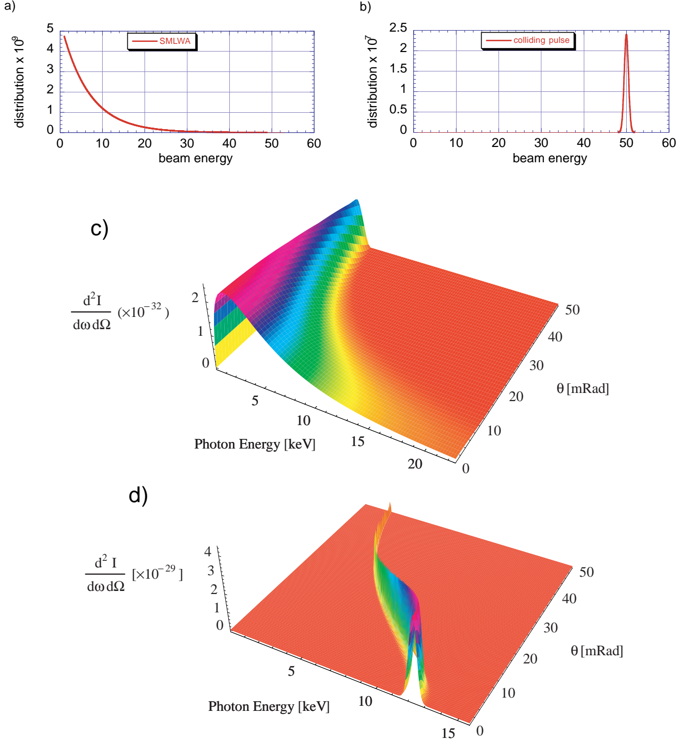
FIG. 2. Energy distribution (a) and spectral flux density (c) for SMLWA; energy distribution (b) and spectral flux density (d) for colliding pulse for the parameters in Table 1. The integral of the distributions are 3 \times 10^{10} and 3 \times 10^7 electrons per bunch for SMLWA and colliding pulse, respectively. The intensity distributions illustrate the contrast between the two injection schemes in scattered X-ray bandwidth and spatial collimation at a fixed observation frequency.
