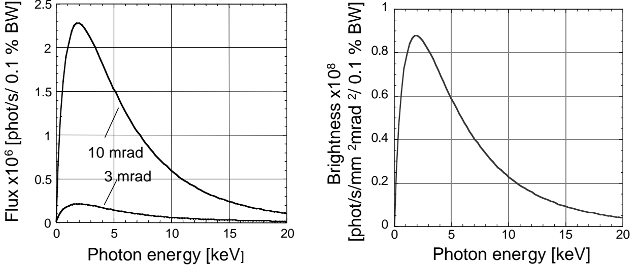
FIG. 1. The average flux into 3 and 10 mrad collection angles and average brightness for the SMLWA-based TS design (see Table 2, col. 2 for parameters) shows the influence of the high charge per bunch ( \sim 5 nC) and broad energy distribution.
