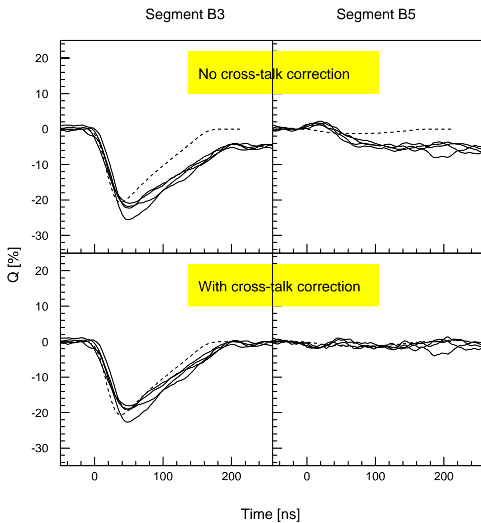
Fig. 10. Signals of segments B3 and B5 as in fig. 6 before (top) and after (bottom) correcting for cross-talk.
