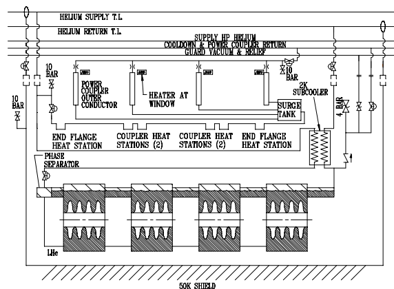
Figure 2: Flow Schematic
