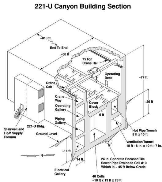
Figure 4 Cross Section of the 221 U-Plant.
