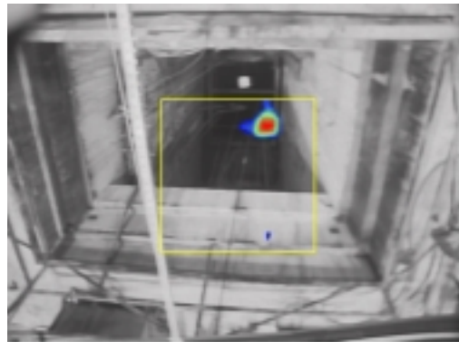
Figure 14 Image of Sources under Shield Cover
