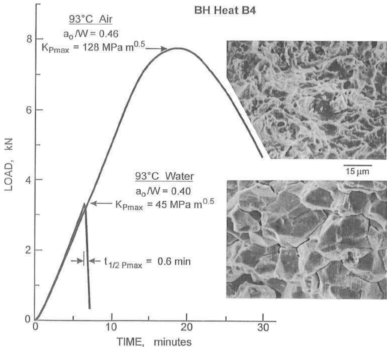
Figure 2. Rising load test results for BH Heat B4 in 93°C air and argon-sparged water. Tests were performed on three-point-bend specimens at a displacement rate of 0.05 mm/min. SEM fractographs show dimple rupture mechanism operative in air and intergranular cracking mechanism operative in water.
