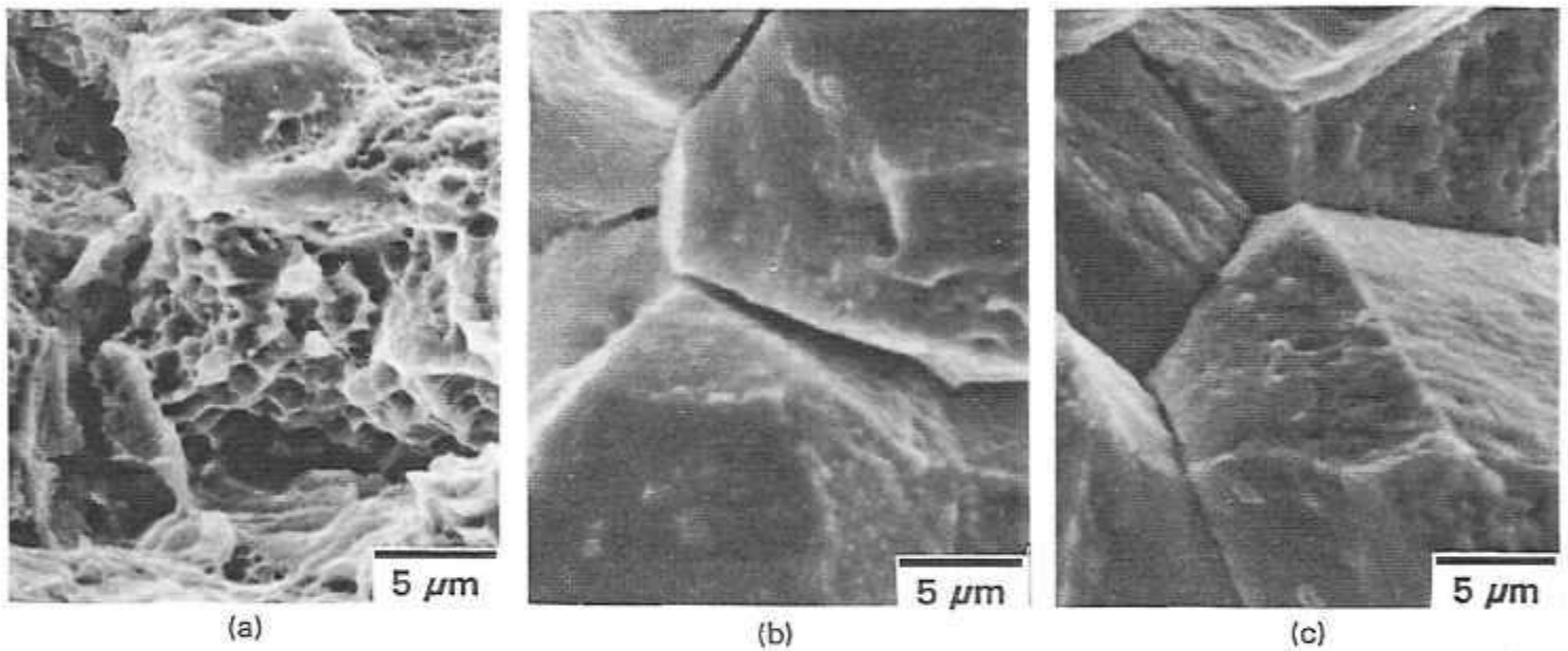
Figure 9. Typical fracture surface morphologies observed in the low temperature regime. (a) Non-precharged specimen tested in air showing ductile microvoid coalescence. (b) Non-precharged specimen tested in water showing intergranular cracking. (c) Hydrogen-precharged specimen tested in air showing intergranular appearance that is indistinguishable from LTCP fracture surface morphology shown in (b).
