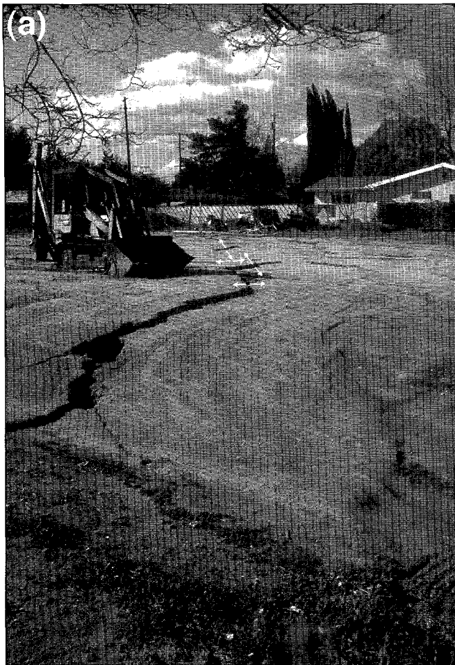
Figure 4. (a) Photograph of rift just south of Malden, and east of Tampa Ave. This large rift went across two vacant lots. View is to the southwest. The trend of the rift is about N40^{\circ}E , and it is made up of biconjugate faults. (b) Details of the east side of the rift. The scarp is almost a decimeter high.
