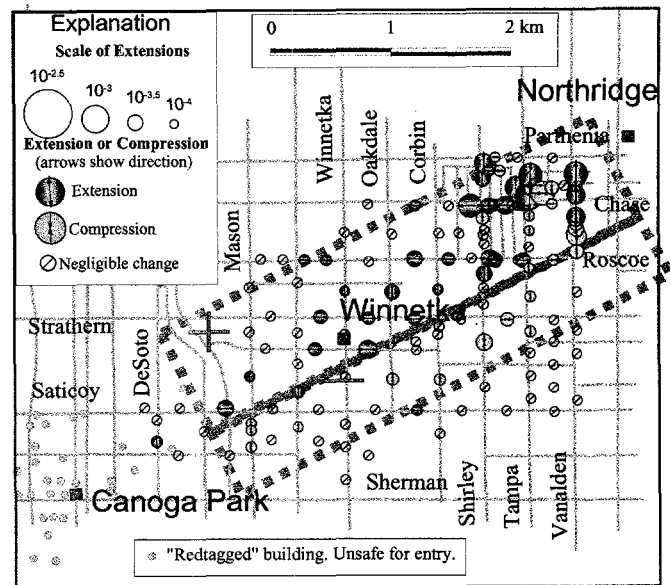
Figure 8. Computed extension of streets in Canoga Park-Winnetka-Northridge area between the 1950's and 1970's and 1985, and after the Northridge earthquake sequence. Magnitude of the largest extension (regardless of sign) indicated by radius of heavy circle. Where extensions were smaller than error, measurement indicated with circle with diagonal line. Significant strains form a deformed zone trending northeast-southwest, about 1 km wide and 4.5 km long. Extension predominates in northwest part (area shown with a "+") and compression in the southeast part (area shown with a "-"). The deformation zone may continue to southeast, as indicated in figure 1, into areas with many red-tagged buildings. More details are shown in Plate 2.
