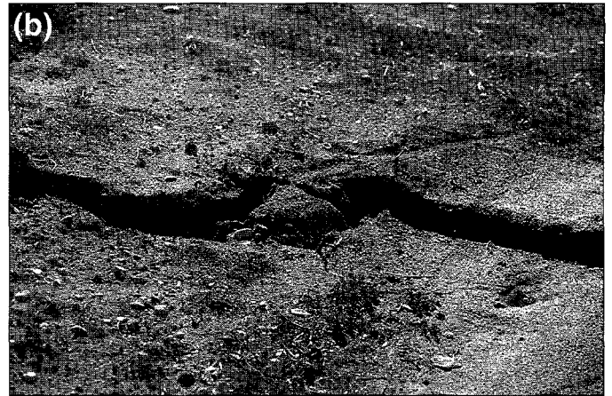
Figure 4. (a) Photograph of rift just south of Malden, and east of Tampa Ave. This large rift went across two vacant lots. View is to the southwest. The trend of the rift is about N40^{\circ}E , and it is made up of biconjugate faults. (b) Details of the east side of the rift. The scarp is almost a decimeter high.
