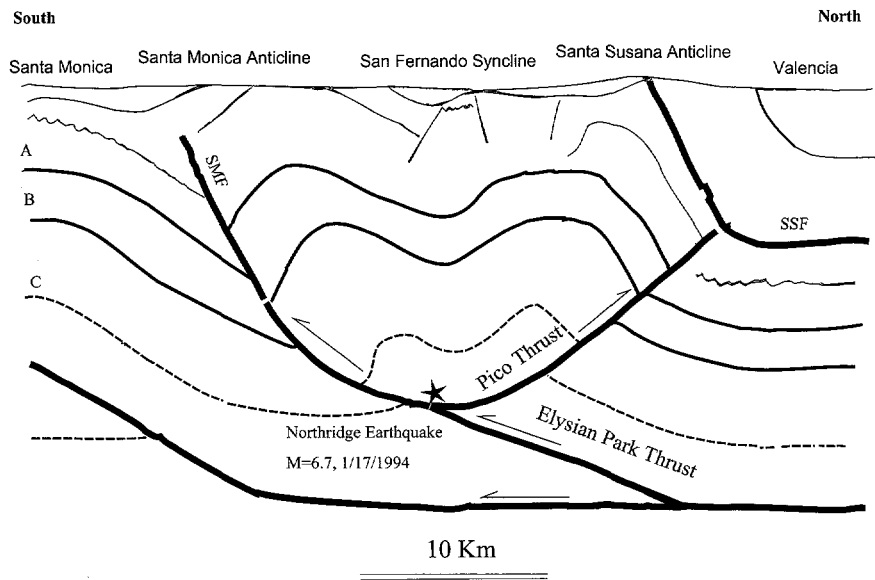
Figure 10. Interpretative structural cross-section of San Fernando Valley area, showing a dish-shaped fault that underlies the center of the valley and that ends beneath the Santa Monica Mountains to the south and the Santa Susana Mountains to the north. (Map modified after Davis and Namson, 1994). The epicenter of the Northridge earthquake was at about 19 km depth, apparently along the Pico thrust fault. The Pico thrust fault is interpreted to be listric in order to explain the tilting of the San Fernando Valley toward the south.
