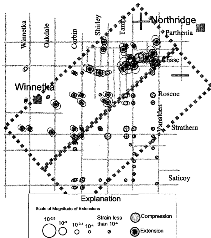
Figure 9. Computed strain figures (shmoos and nerds) of streets in Winnetka/Northridge area between the 1950's to 1970's and 1985, and after the Northridge earthquake sequence. The strain figures show that the belt of extension in the Winnetka deformation zone is dominated by principal extensions in the northwest and southeast direction, and that the belt of compression is dominated by a principal compression in the same direction. The pattern indicates that the Winnetka deformation zone would not be a strike-slip fault, but rather a reverse or normal fault. See Plate 3 for details.
