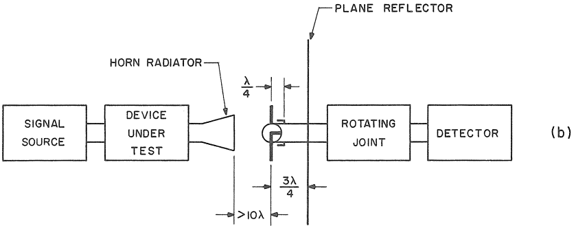
FIGURE 14. Standard attenuators for direct substitution attenuation measurements.
