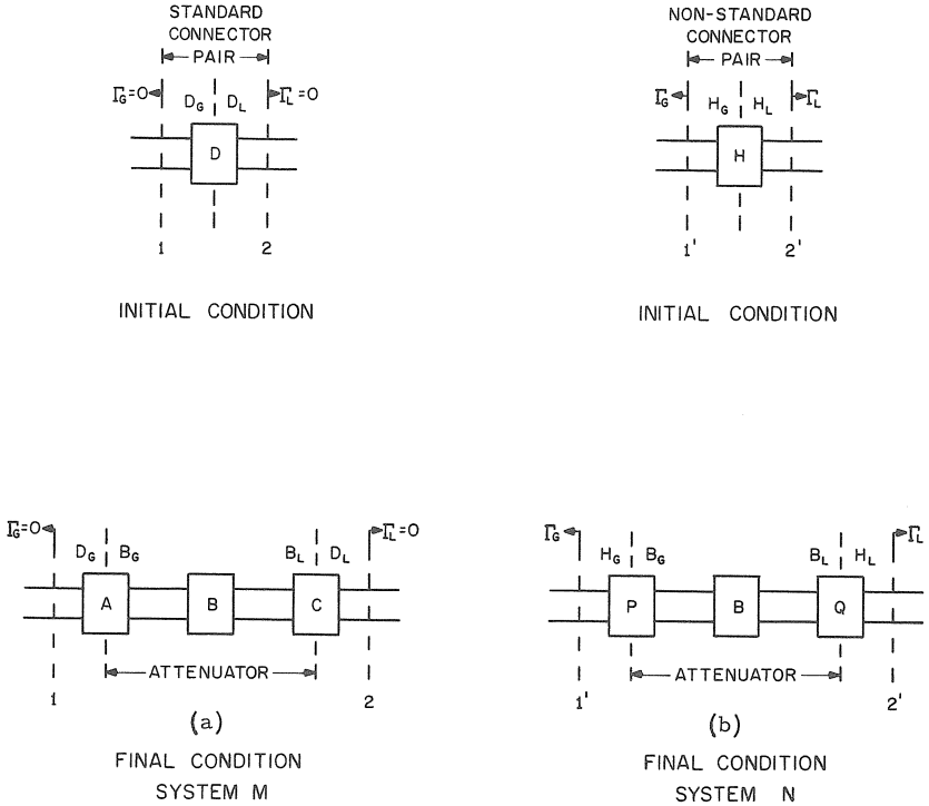
FIGURE 7. Representation of same attenuator installed alternately in two systems. (a) System M nonreflecting and joined with a standard connector pair. (b) System N has reflections and is joined with a nonstandard connector pair.
