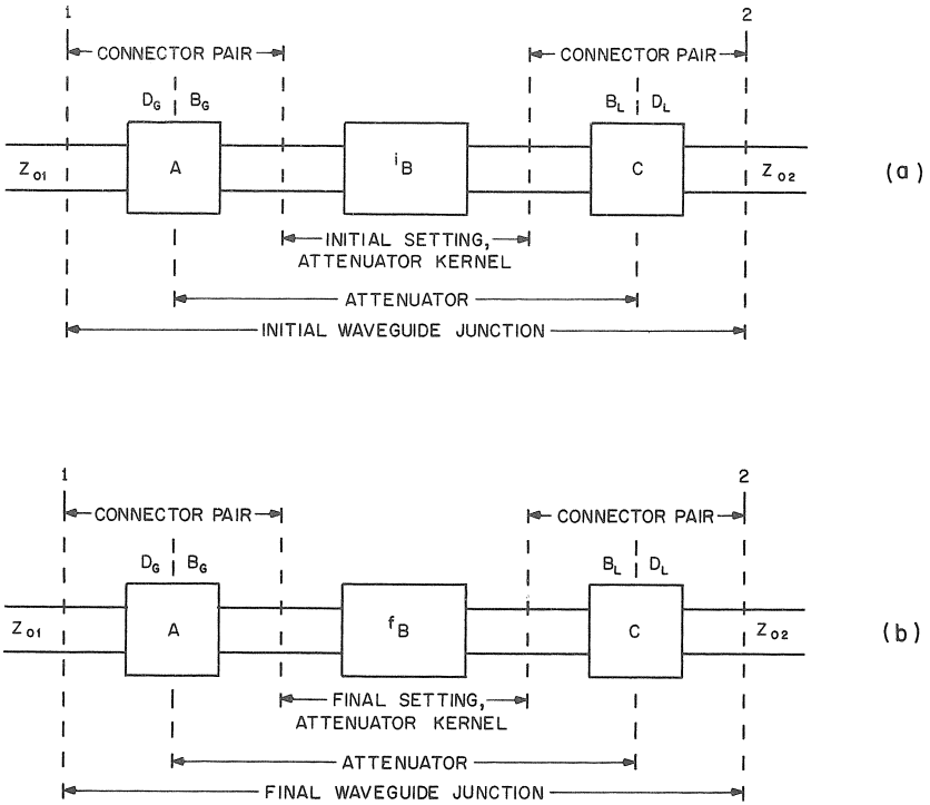
FIGURE 5. Representation of a continuously variable attenuator installed in a waveguide system.
