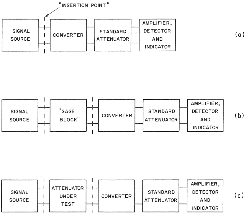
* FIGURE 11. Basic IF substitution attenuation measurement systems.
