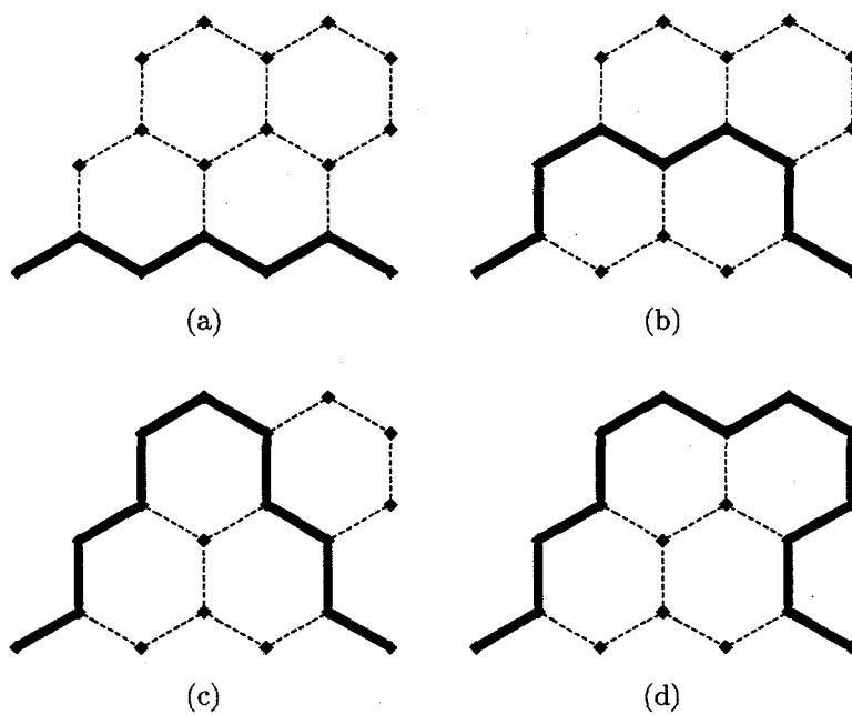
Figure 8: Illustration of the embedding of extensible paths from \hat{L}_0^H into the hexagonal lattice. Figure (a) shows the initial path that is extended by two in (b), (c) and (d).
