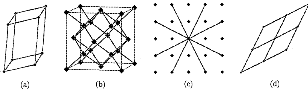
Figure 7: Bipartite crystal lattices: (a) triclinic, (b) fluorite, (c) the "210 lattice", and (d) the embedding of L into the "210 lattice".
