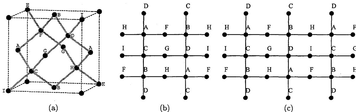
Figure 4: Embedding the \hat{L}_0^2 latticoid into a diamond lattice: (a) labeled unit cell, (b) embedding onto plane of unit cells with embedded latticoid, and (c) extending this embedding.
