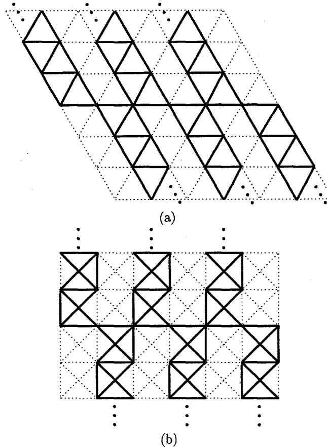
Figure 9: Illustration of (a) the nonbipartite latticoid used by the nonbipartite master approximation algorithm in L' , the triangular lattice. This latticoid can be embedded in the face centered cubic lattice as shown in (b).
