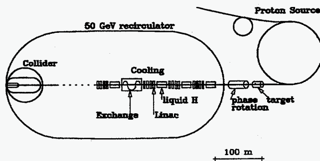
Figure 2: Plan of a 100 GeV CoM Muon Collider.
