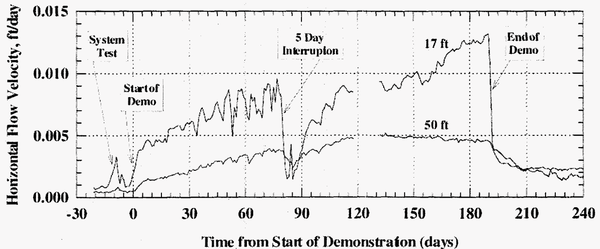
Figure 6. Horizontal flow velocity, relative to background, recorded by the near and far flow sensors during a demonstration at Edwards Air Force Base.
