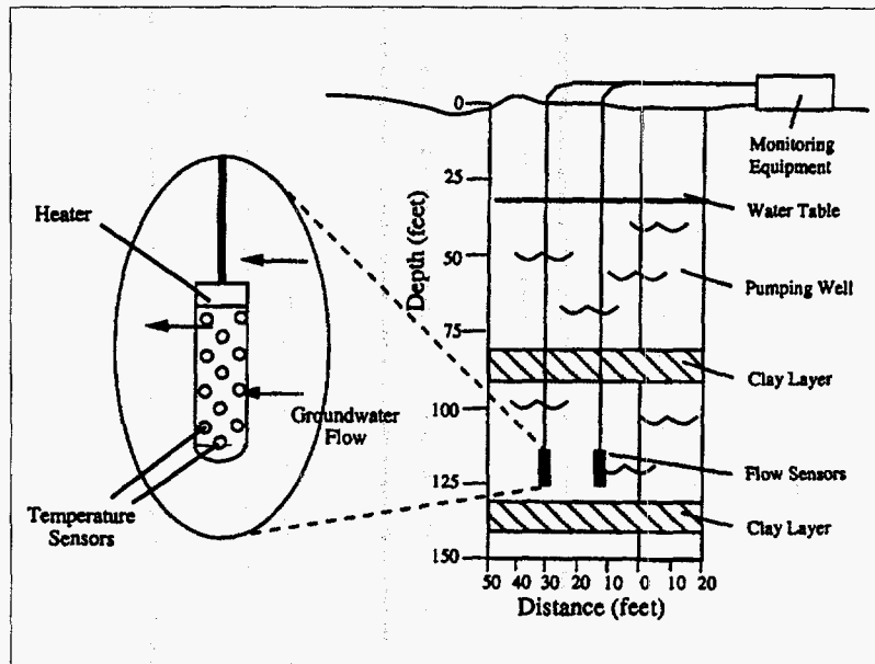
Figure 2. In Situ Permeable Flow Sensor Schematic Diagram showing installation of two flow sensors adjacent to a pumping well.
