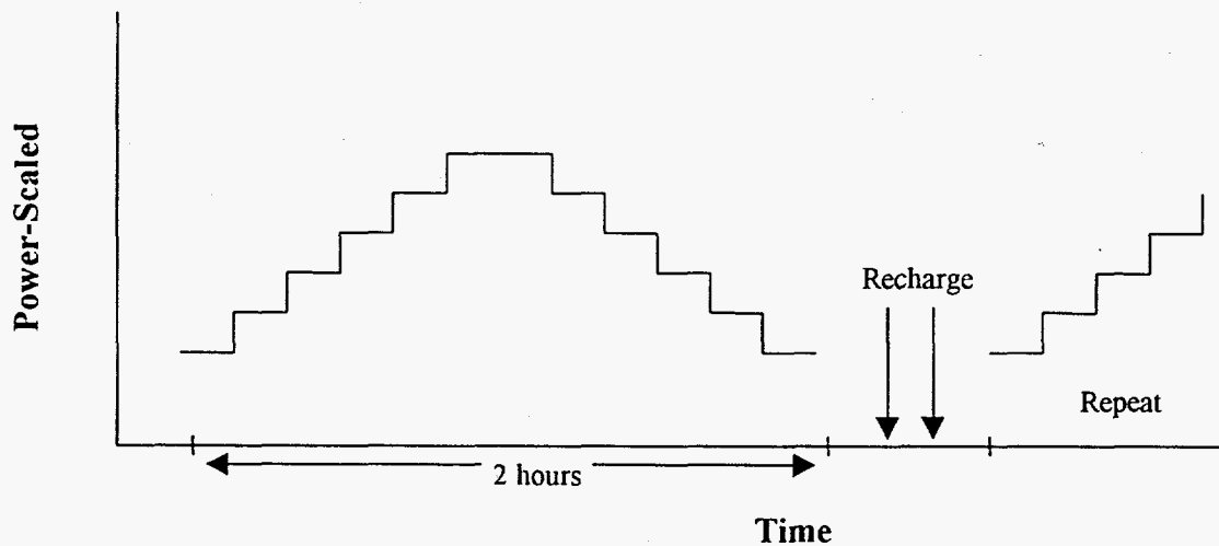
Figure 4 - Peak Shaving Test Profile
