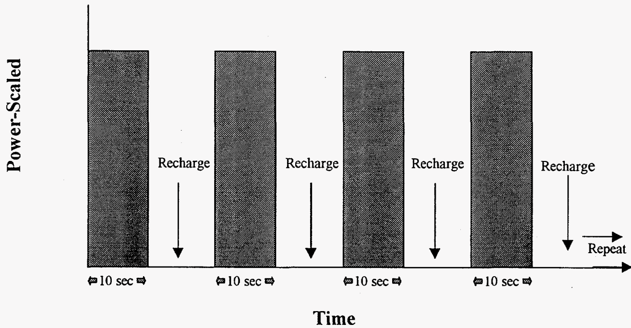
Figure 2 - Power Quality Test Profile
