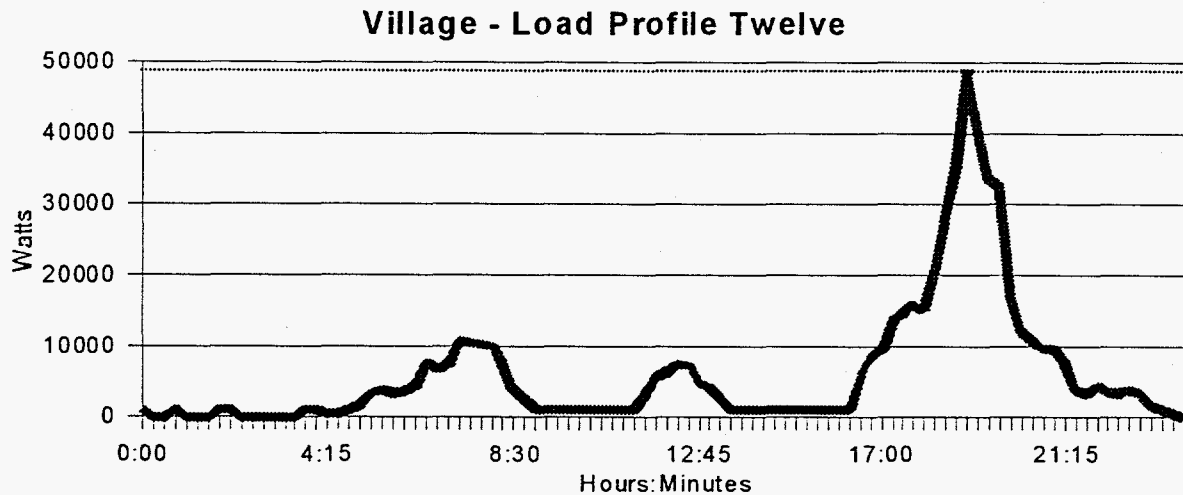
Figure 3. Example RAPS test profile
