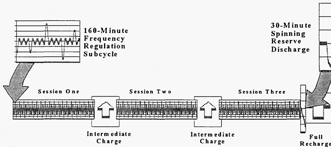
Figure 1B. Frequency Regulation & Spinning Reserve Test Profile
