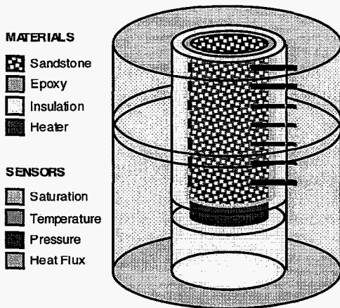
Figure 2. Schematic of experimental setup for boiling experiment.
