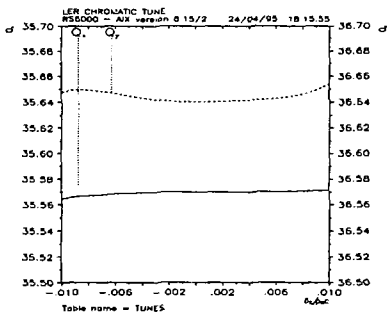
Figure 2. Tune versus relative momentum deviation.
