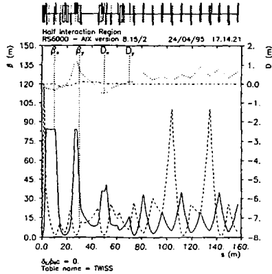
Figure 1. Optical functions for the one half IR.
