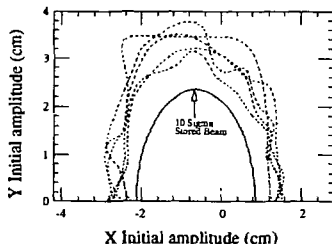
Figure 3. Dynamic aperture for non-interleaved sextupoles and 90^\circ cells, 5 seeds with full alignment and multipole errors, 10\sigma_E offset.
