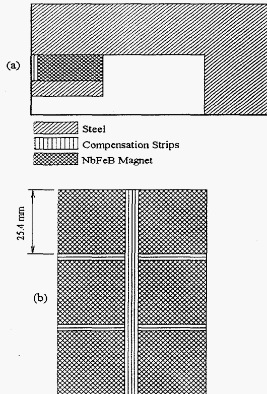
Figure 1: (a) Symmetrical cross section of a quadrant of a dipole magnet with a soft-steel pole and flux-return yoke. The NdFeB block is magnetized in the vertical direction. (b) Top view for the arrangement of the permanent magnet blocks and the temperature compensation strips inserted between the blocks.
