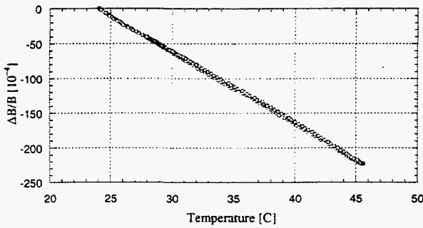
Figure 2: Magnetic field data under a slow thermal cycle for a NdFeB permanent dipole magnet. Temperature coefficient for the relative magnetic field in the air gap was (\Delta B/B)/\Delta T = -1.1 \times 10^{-3}/^\circ\text{C} in the temperature range of 25-35°C.
