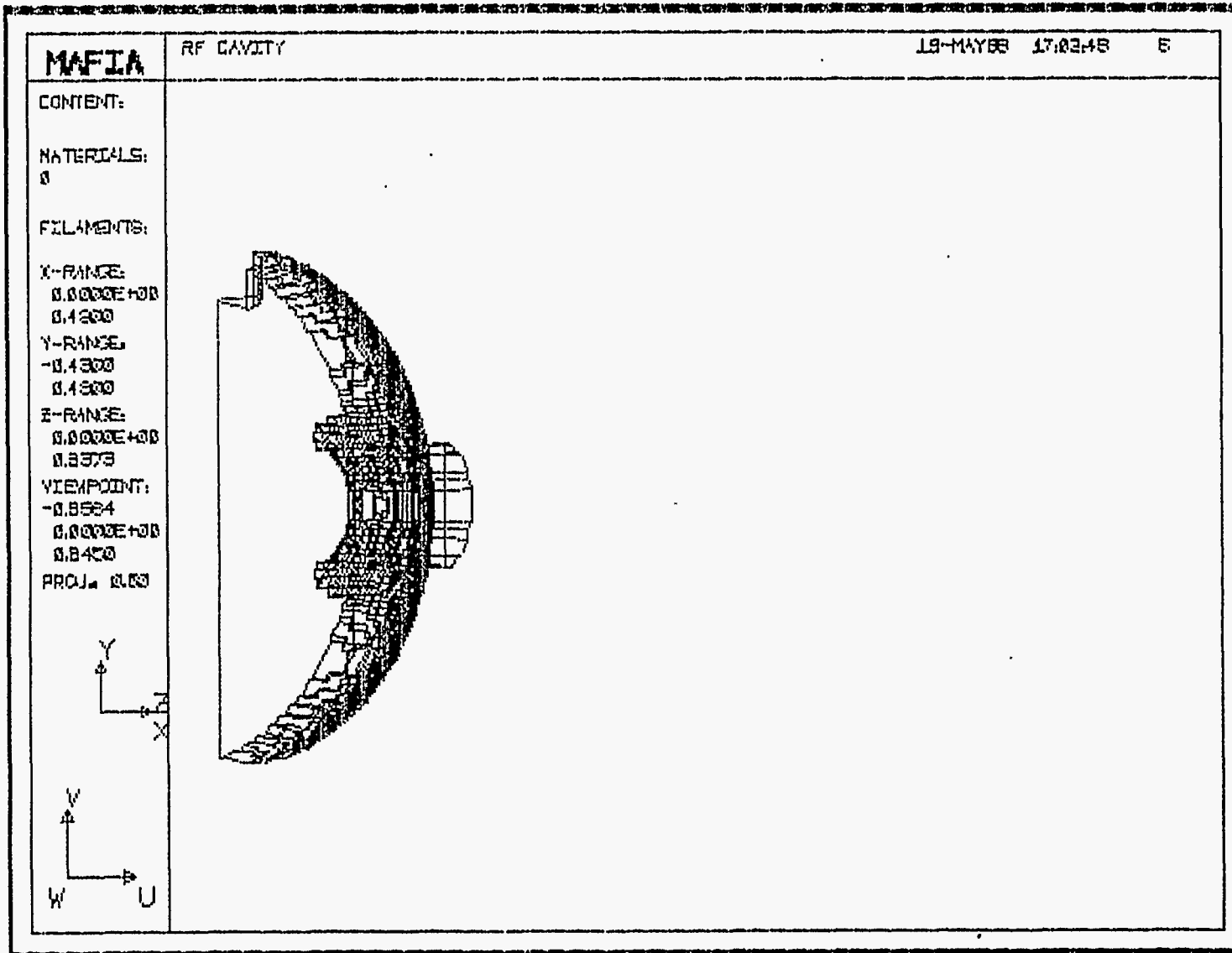
Fig. 4. One-fourth structure of the cavity, used for calculating tuner range.
