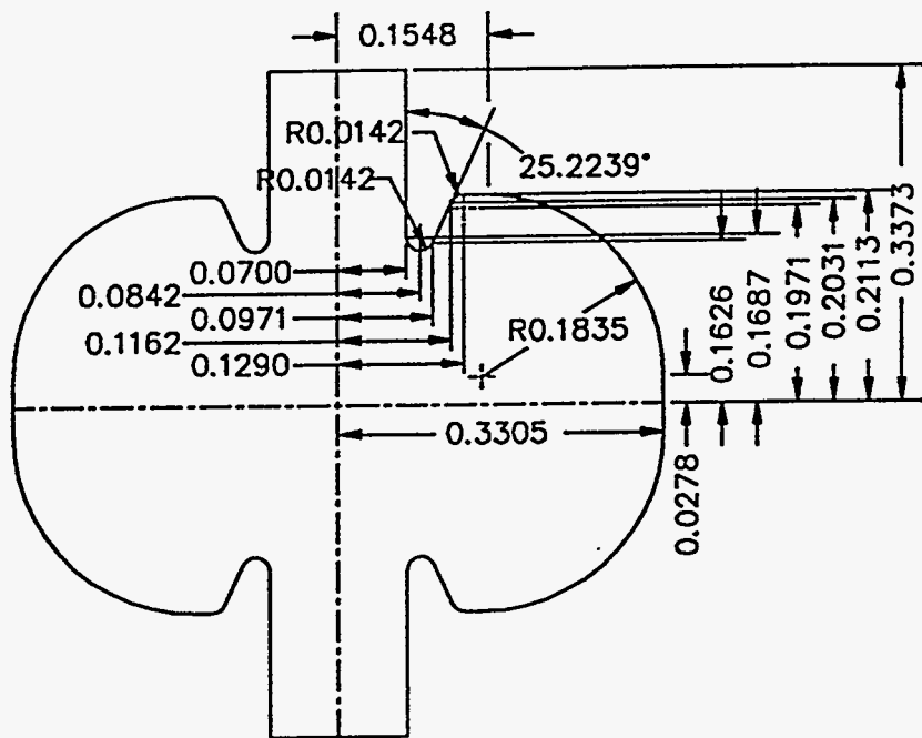
Fig. 1a. The basic shape and dimensions of the cavity.
