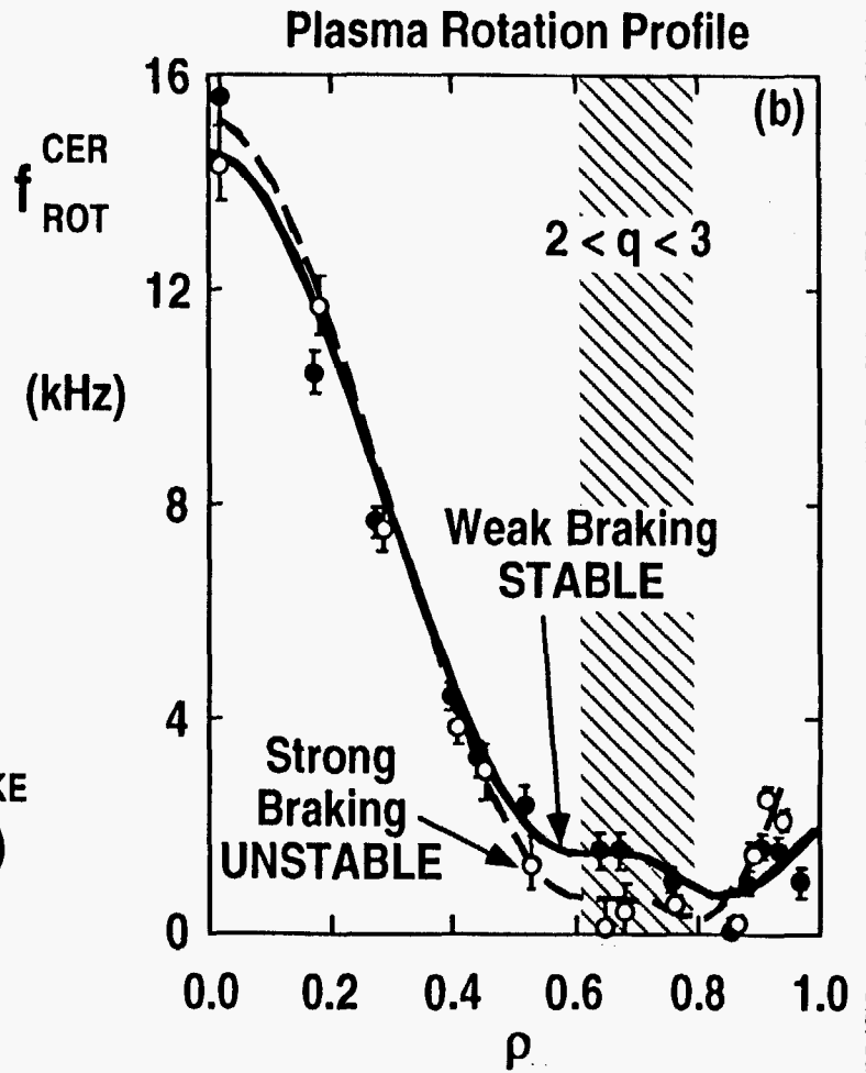
Fig. 5. (a) Temporal evolution of two similar discharges, one with large C-coil current, and one with smaller C-coil current, (b) toroidal rotation profile of the two discharges shown at the time of the arrow in (a).
