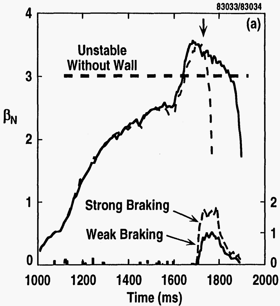
Fig. 5. (a) Temporal evolution of two similar discharges, one with large C-coil current, and one with smaller C-coil current, (b) toroidal rotation profile of the two discharges shown at the time of the arrow in (a).
