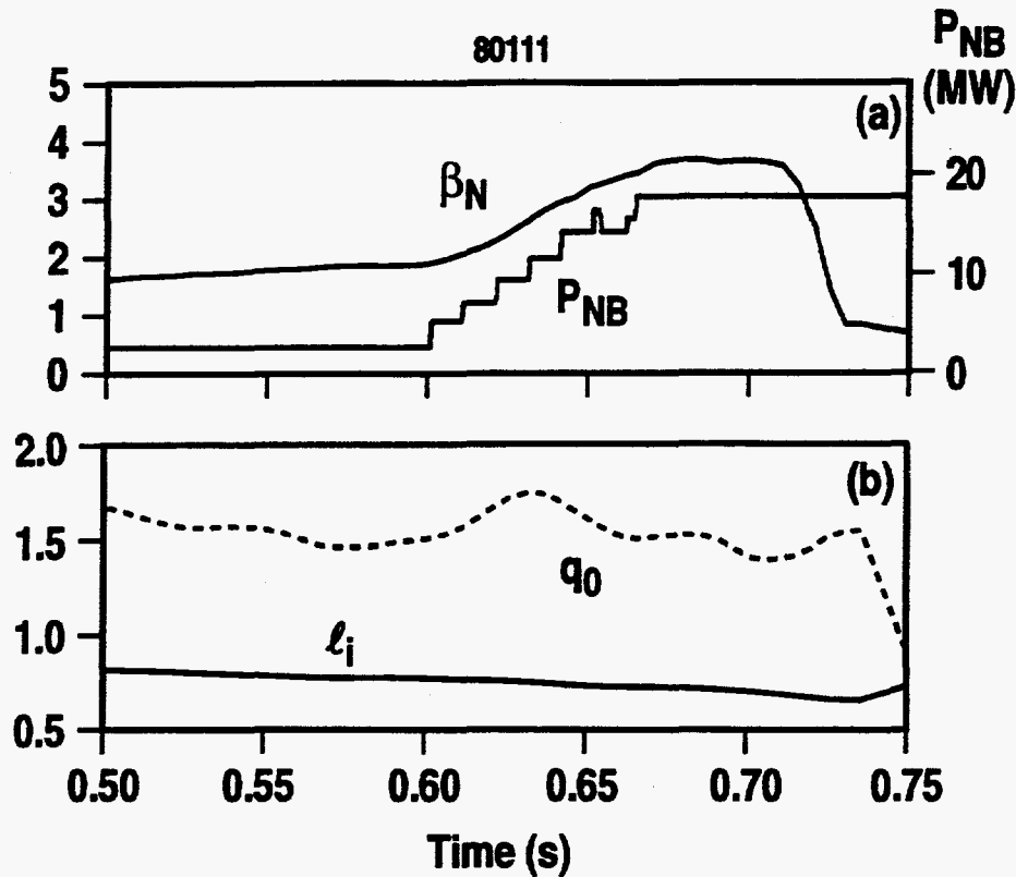
Fig.1. Temporal evolution of wall stabilized discharge. (a) normalized plasma beta, \beta_N = \beta_T / (I/aB) \% \text{-m-T/MA} , and injected neutral beam power, P_{NB} (b) calculated internal inductance l_i and measured central safety factor, q(0)
