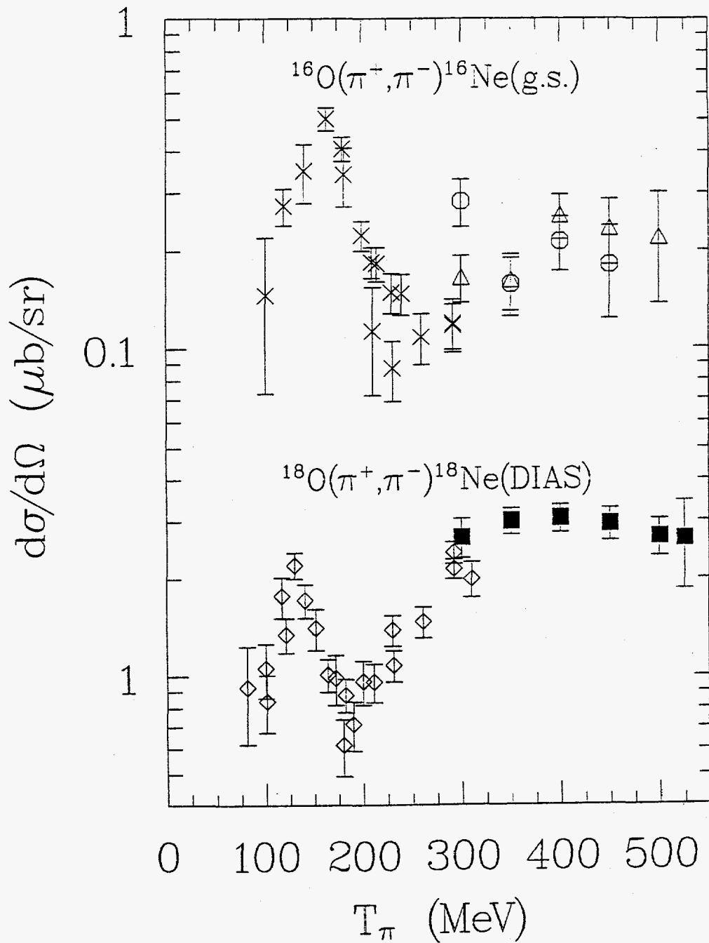
Figure 2: Forward-angle differential cross sections for ^{16}\text{O}(\pi^+, \pi^-)^{16}\text{Ne}(\text{g.s.}) and ^{18}\text{O}(\pi^+, \pi^-)^{18}\text{Ne}(\text{DIAS}) . Shown are two data sets from this experiment, as open circles and triangles. Results from previous experiments[8, 9] are indicated by crosses. The ^{18}\text{O} results at lower energies (diamonds) are from ref.[10], and those at higher energies (filled squares) are from ref.[1].
