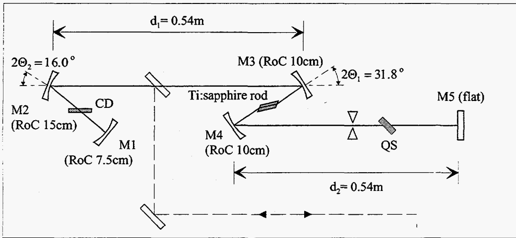
Figure II.6: Diagram of the final amplifier cavity. The path of the injected and cavity dumped pulses is drawn dashed. CD=cavity dumper, QS=Q-switch, M1-M5=mirrors. The distance between the \text{Ti:Al}_2\text{O}_3 rod and M3, M4 is 4.7cm
