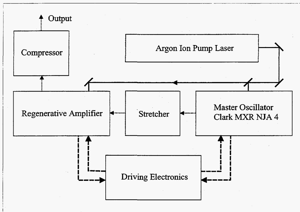
Figure I.1: Schematic setup of a Ti:sapphire oscillator-amplifier system.
