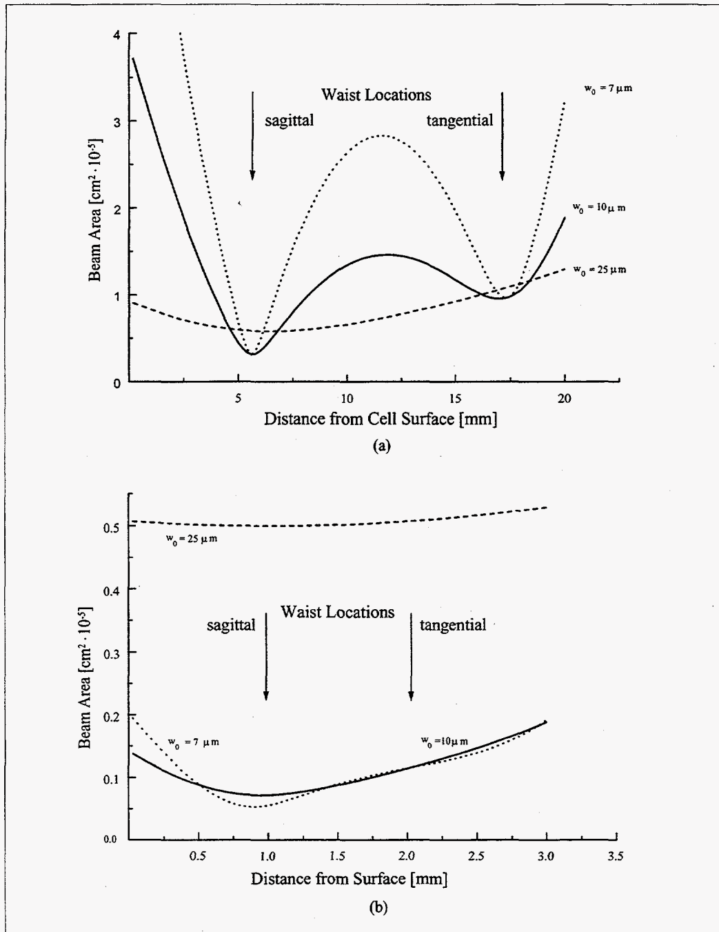
Figure II.3: Gaussian beam propagation through a Brewster plate. \lambda = 820\text{nm} , n = 1.76 . (a) t = 20\text{mm} . (b) t = 3\text{mm} . The indicated waist sizes are values for assumed focusing in air.
