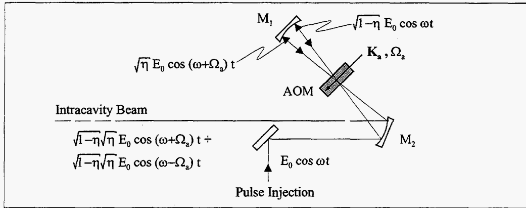
Figure V.3: Pulse injection using a double pass configuration and interferometric superimposition. For dumping out of the cavity, the two frequency components of the intracavity beam have to be considered.
