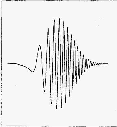
Figure IV.1: Linearly chirped pulse with Gaussian envelope function
