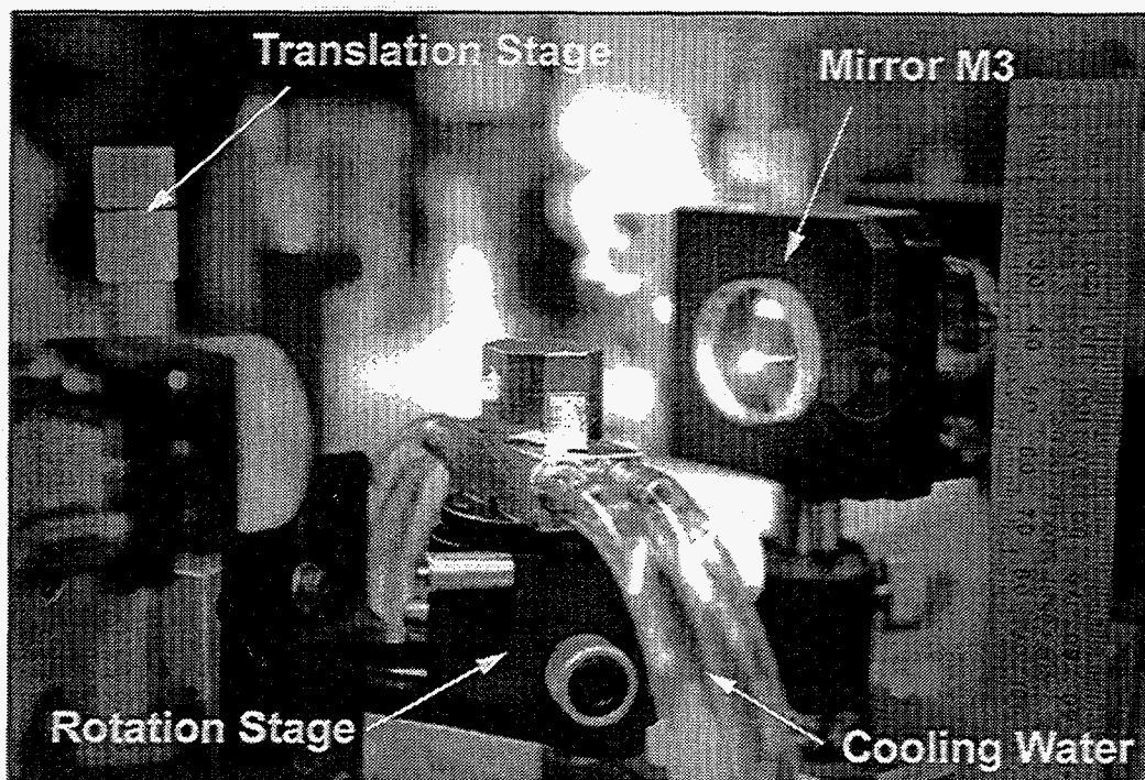
Figure III.3: Ti:sapphire crystal and mount (in final setup)
