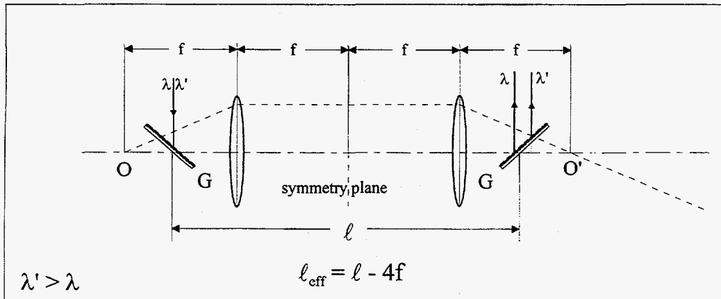
Figure IV.3: Effect of a 1:1 telescope in a grating stretcher: The distance between O and O' (focal points) must be subtracted from l , because the optical paths for propagation at different angles are identical. If the gratings G are located inside the focal planes, the effective distance between the gratings is negative. The beams \lambda and \lambda' are shown schematically
