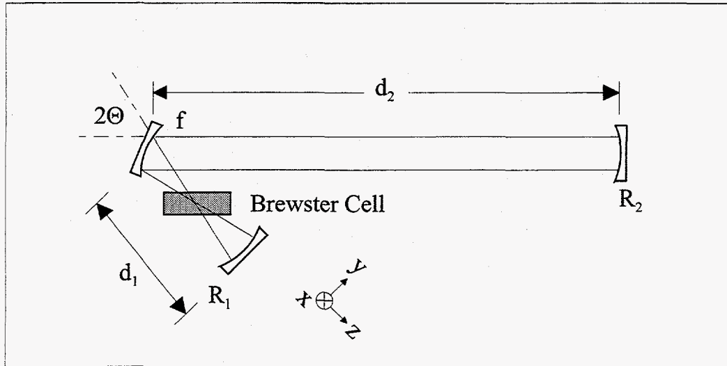
Figure II.4: Folded 3-mirror cavity with internal Brewster-angle cell of thickness t . d_2 \gg d_1 and d_1 \approx R_1 + f
