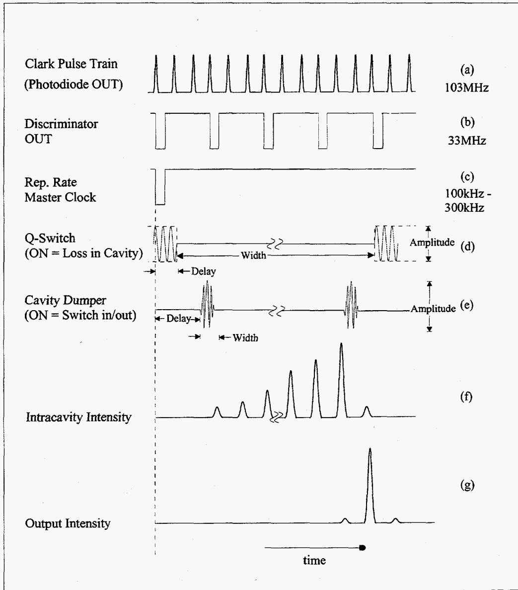
Figure V.4: Timing Scheme for the Amplifier System.
