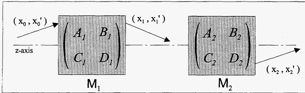
Figure II.1: Ray transformation through optical elements
