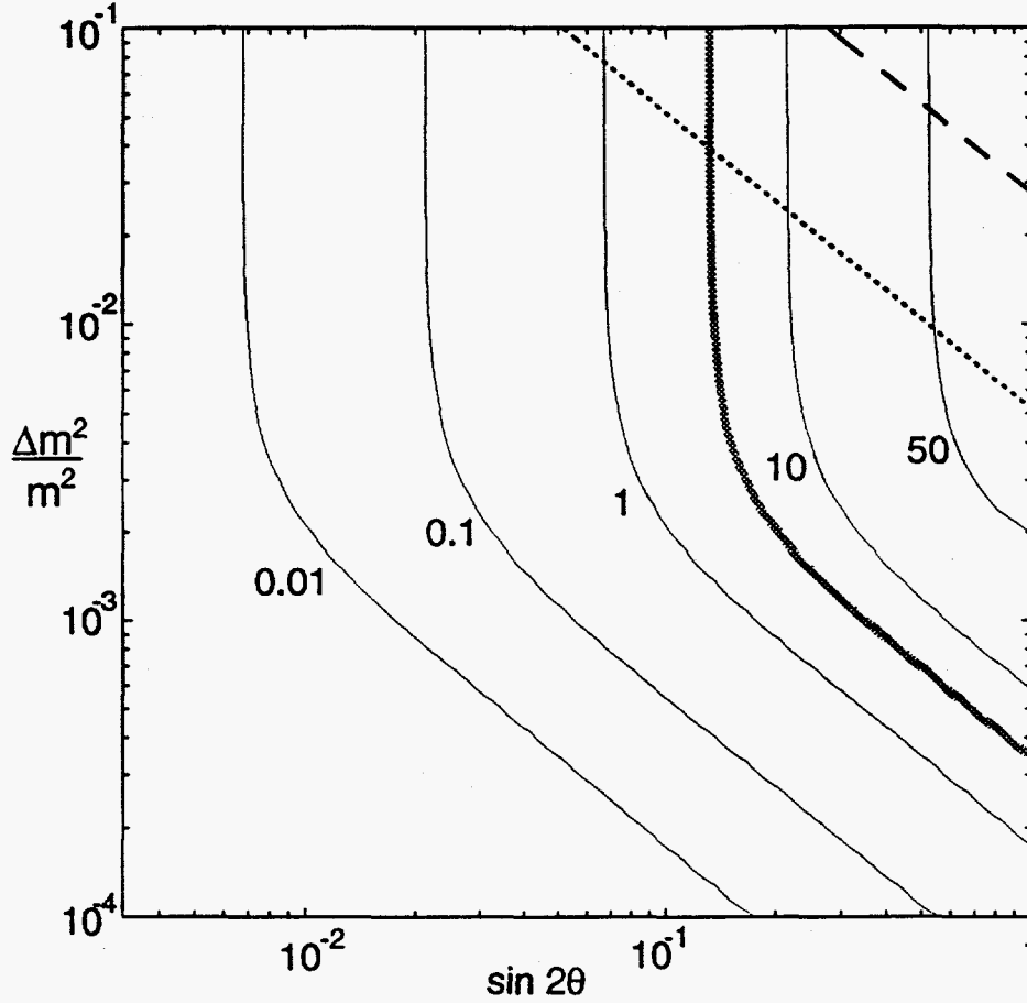
Figure 1: Contours of constant \sigma(e^+e^- \rightarrow e^\pm\mu^\mp\tilde{\chi}^0\tilde{\chi}^0) (solid) in fb for NLC, with m_{\tilde{e}_R}, m_{\tilde{\mu}_R} \simeq 200\text{GeV} , M_1 = 150\text{GeV} , \mu = -400\text{GeV} , M_2 = 300\text{GeV} , and \tan\beta = 2 . The thick gray contour represents the experimental reach for one year's integrated luminosity. The dashed (dotted) contour is the current experimental bound from B(\mu \rightarrow e\gamma) = 4.9 \times 10^{-11} for the same parameters and \tan\beta = 2(50) , m_{\tilde{e}_L}, m_{\tilde{\mu}_L} = 350\text{GeV} . (The cross section contours are basically unchanged for \tan\beta = 50 .)
