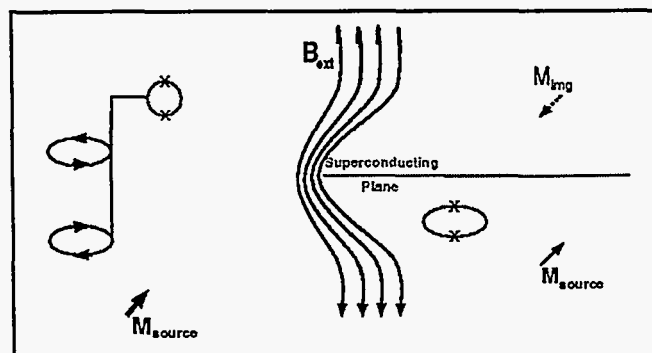
Figure 1a. (left) Depiction of conventional wire-wound gradiometer connected to a SQUID and responding to a magnetic source. Figure 1b. (right) Superconducting image-plane gradiometer concept showing a “real” magnetic source, M_{source} , and an “image” source, M_{img} . See text for detailed description.
