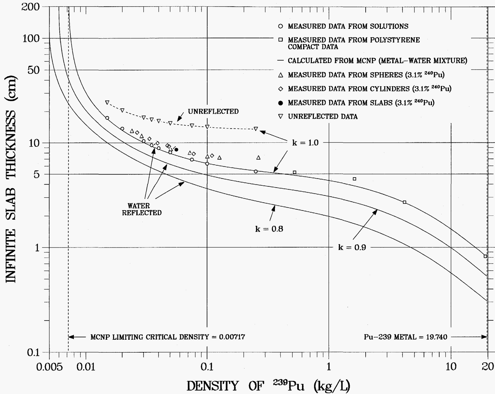
Fig. 13. Thicknesses of infinite slabs of homogeneous water-moderated 239 Pu as functions of 239 Pu density.
