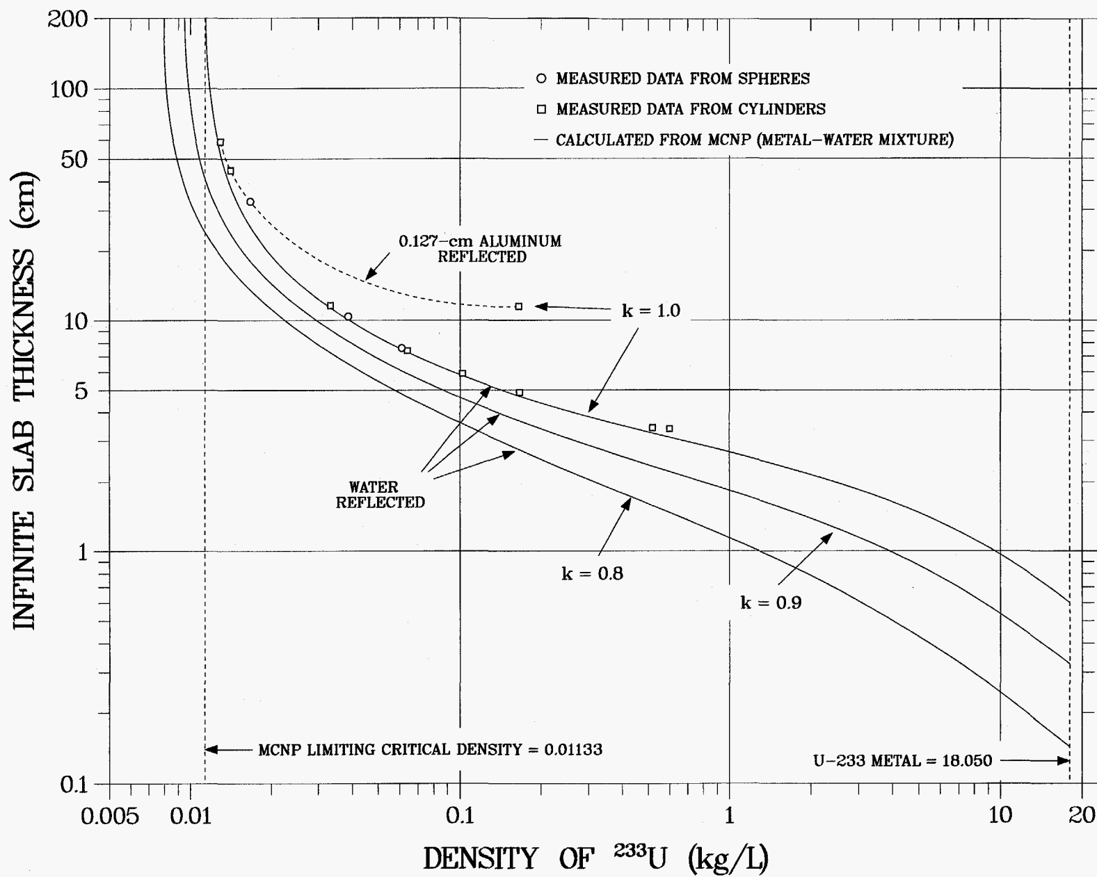
Fig. 5. Thicknesses of infinite slabs of homogeneous water-moderated ^{233}\text{U} as functions of ^{233}\text{U} density.
