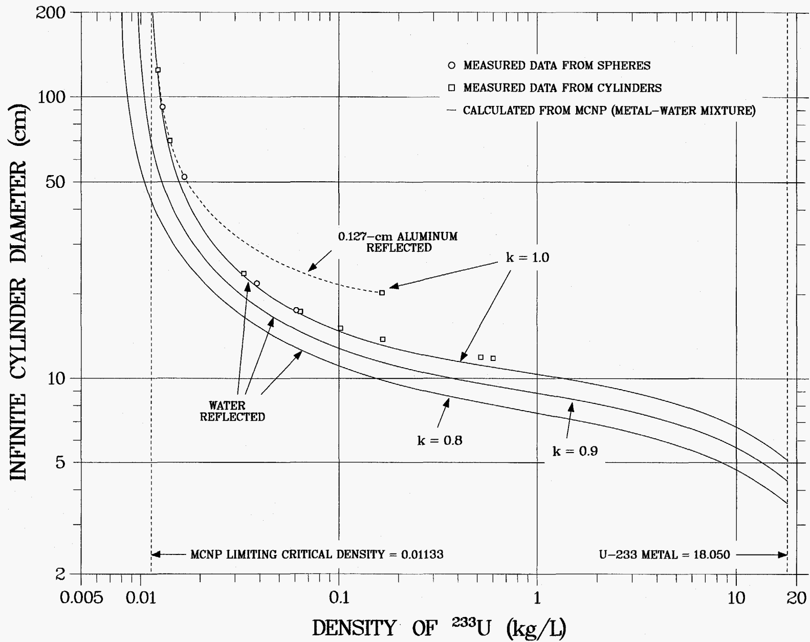
Fig. 4. Diameters of infinite cylinders of homogeneous water-moderated ^{233}\text{U} as functions of ^{233}\text{U} density.
