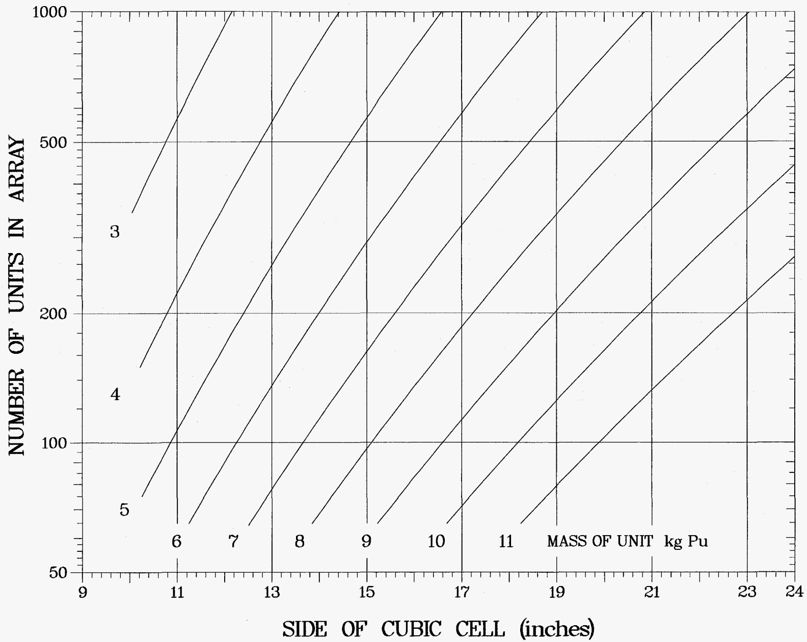
Fig. 23. Subcritical reflected arrays of spherical units of Pu(94.8) oxide at H/Pu \leq 0.40 .
