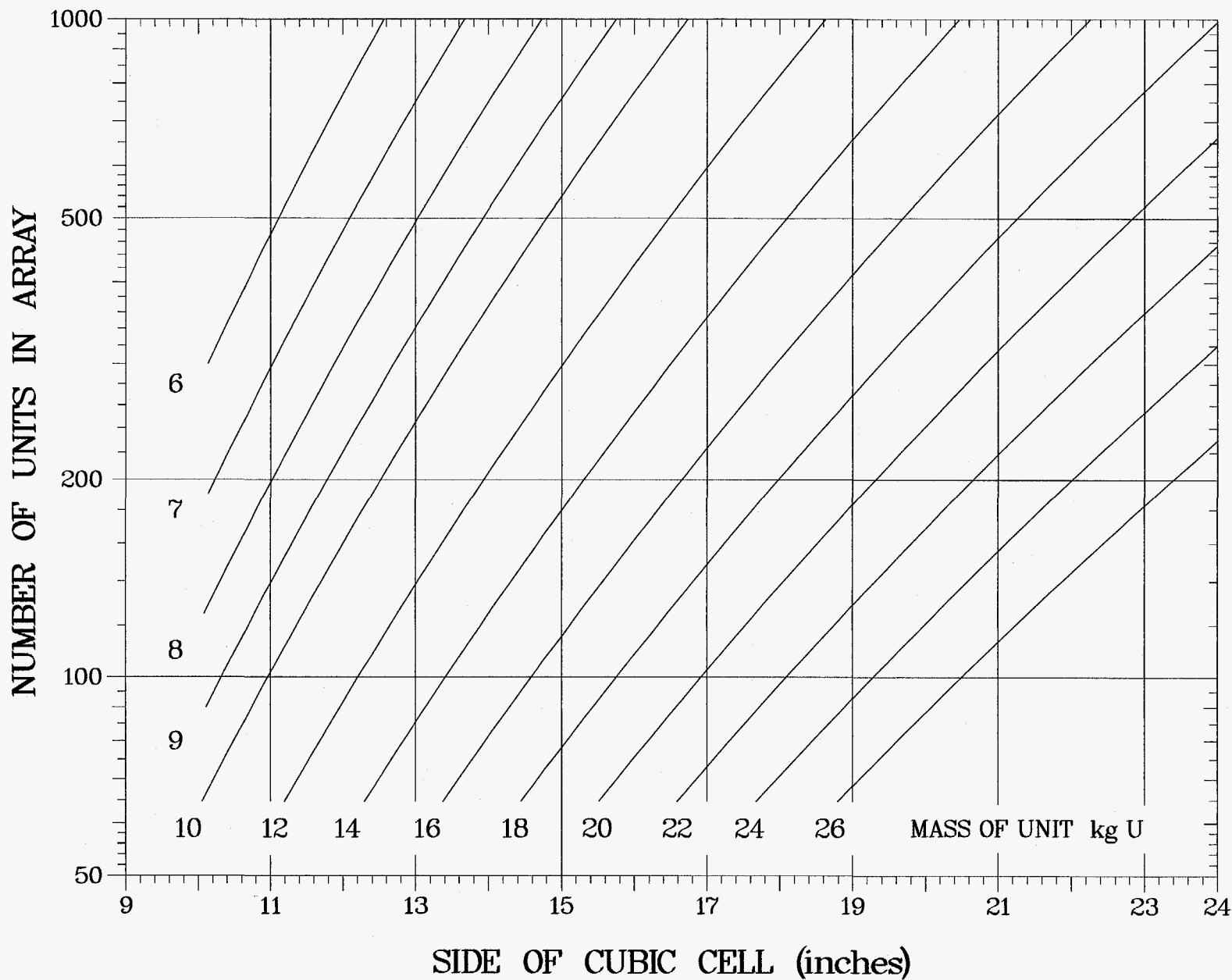
Fig. 20. Subcritical reflected arrays of spherical units of U(93.2) oxide at H/U \leq 0.40 .
