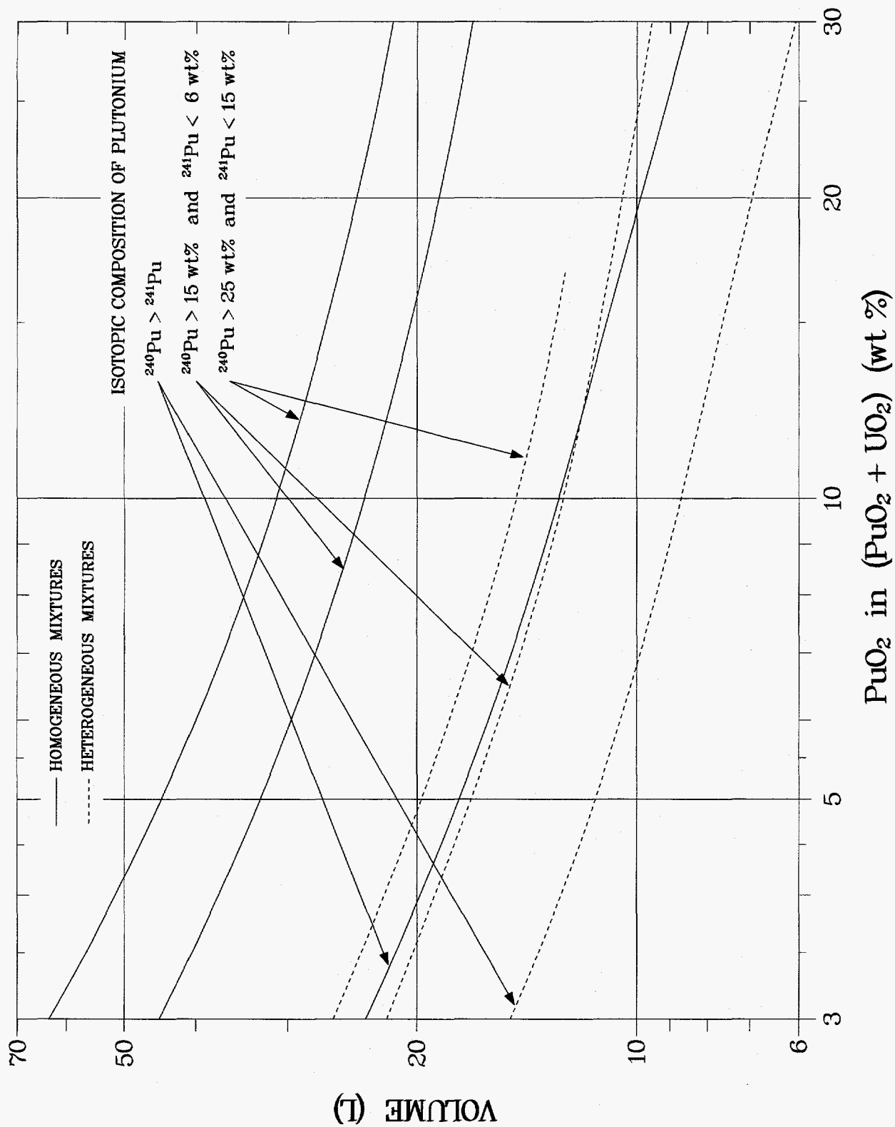
Fig. 15. Subcritical volume limits for water-reflected spheres of aqueous mixtures of PuO 2 and U(0.7)O 2 .
