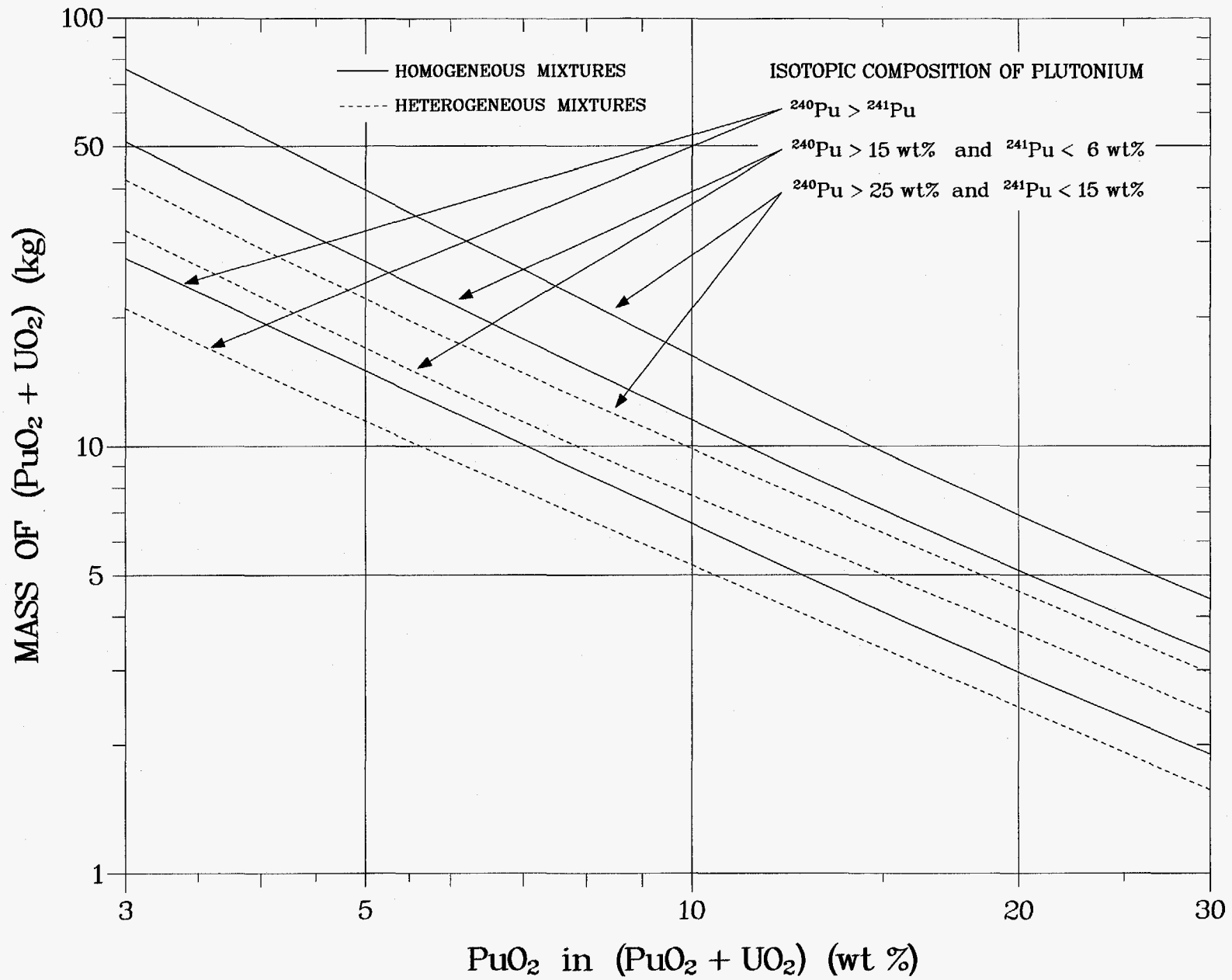
Fig. 14. Subcritical mass limits for water-reflected spheres of aqueous mixtures of \text{PuO}_2 and \text{U}(0.7)\text{O}_2 .
