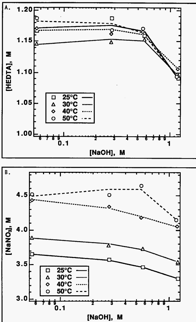
Figure 3-11. Solubility of sodium HEDTA in \text{NaNO}_3 - \text{NaNO}_2 solutions saturated with crystalline \text{NaNO}_3 at 25 °C, 30 °C, 40 °C, and 50 °C for various sodium hydroxide concentrations (A), and measured sodium nitrate concentrations in the same solutions (B).
