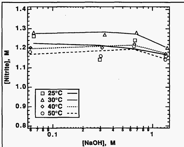
Figure 3-8. Measured sodium nitrite concentrations in solutions where the solubility of sodium butyrate was determined. These solutions were saturated with crystalline \text{NaNO}_3 at 25 °C, 30 °C, 40 °C, and 50 °C, the initial sodium nitrite concentration was 2.0 M, and initial sodium hydroxide concentrations varied from 0.1 M to 2.0 M.
