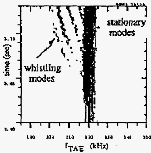
Figure 3 Frequency spectrum versus time showing the frequency-decreasing modes (“whistling”) and the “stationary” modes. (same conditions as in Figure 2, with P_{it}=6.5 MW)
