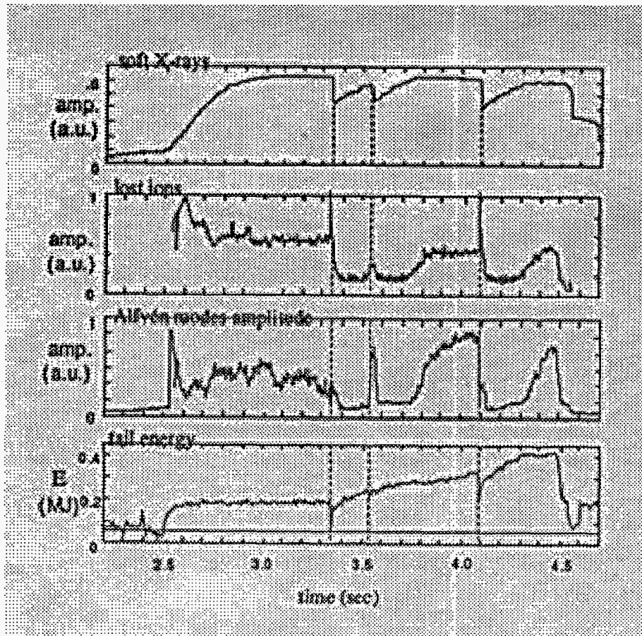
Figure 4 Correlation between soft X-ray, lost particles and TAE modes intensities and tail energy in a TFTR discharge similar to the one in Figure 2, with P_{\text{rf}}=4.8 MW.
