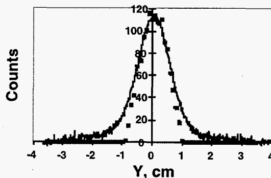
Fig. 2. Hydrogen beam profile 42.9 cm from the source measured with a video camera (line) and predicted by SCHAR (squares).
