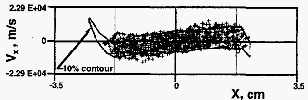
Fig. 1. The SCHAR-calculated phase space (crosses) at the EMU for the LEDA prototype LEBT. The solid line is the 10% phase-space contour measured with the EMU.
