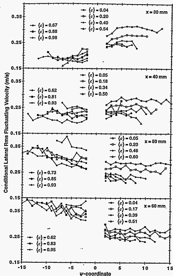
Figure 13: Profiles of the lateral rms fluctuating velocity conditional on \psi . Statistics computed for regions within the flamelet thermal thickness, \psi = -1, 0, \text{ and } 1 , are not shown.
