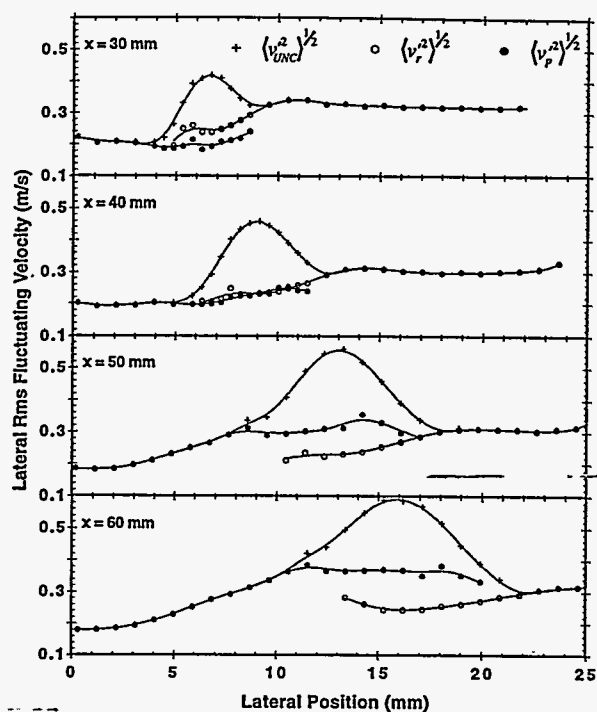
Figure 8: Lateral rms turbulence levels— unconditional and zone conditional lateral (y) coordinate profiles.
