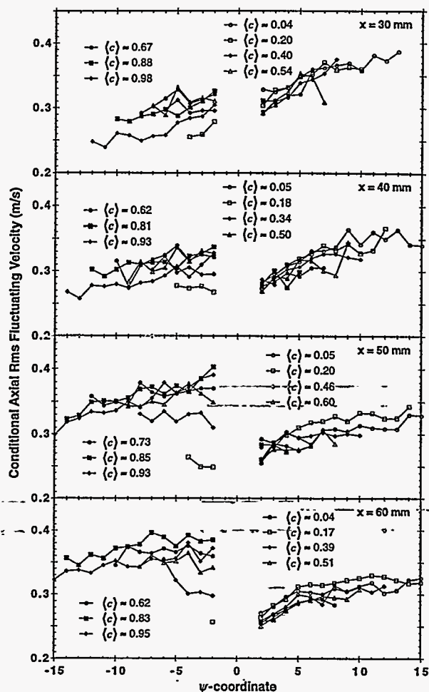
Figure 14: Profiles of the axial rms fluctuating velocity conditional on \psi .
