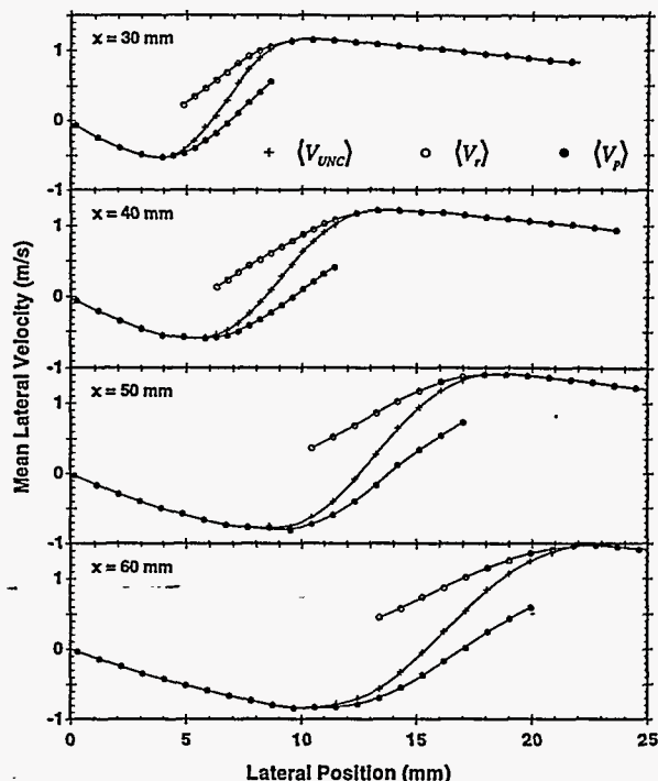
Figure 6: Mean lateral velocity— unconditional and zone conditional (products or reactants) lateral coordinate profiles
