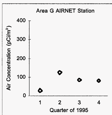
c. Americium-241
