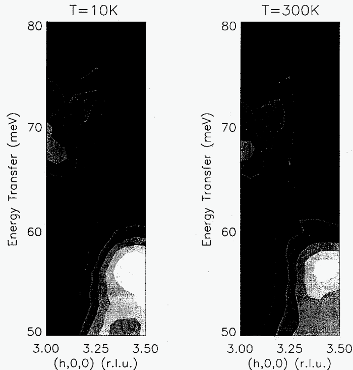
FIGURE 2. Intensity contour plot for the LO phonon branches of \text{YBa}_2\text{Cu}_3\text{O}_{6.93} at T = 10 \text{ K} (left) and at room temperature (right).
