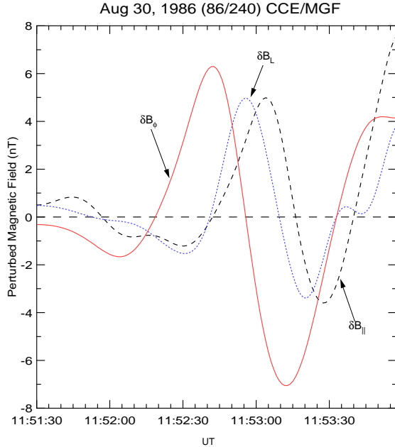
Figure 1. Three components of the low frequency perturbed magnetic field.
