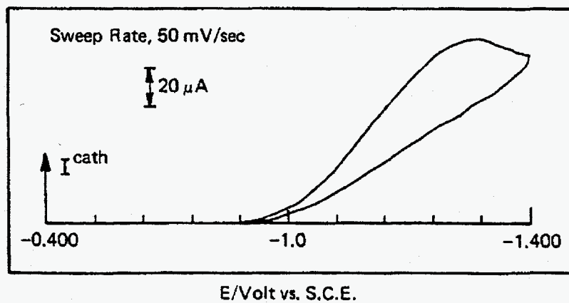
FIGURE 8. Cyclic Voltammogram of 0.59M NaNO 3 in 3M NaOH, 0.25M Na 2 CO 3 at 80°C
