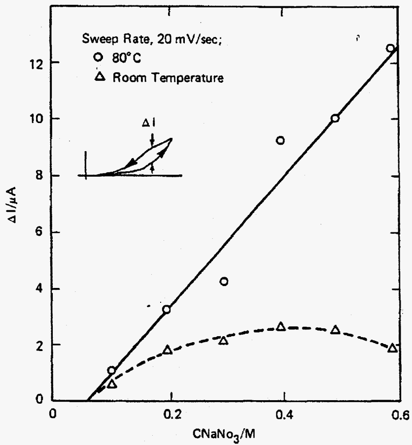
FIGURE 10. Variation of I at Nickel Electrode with Concentration of \text{NaNO}_3 in \text{NaOH} at 80^\circ\text{C}
