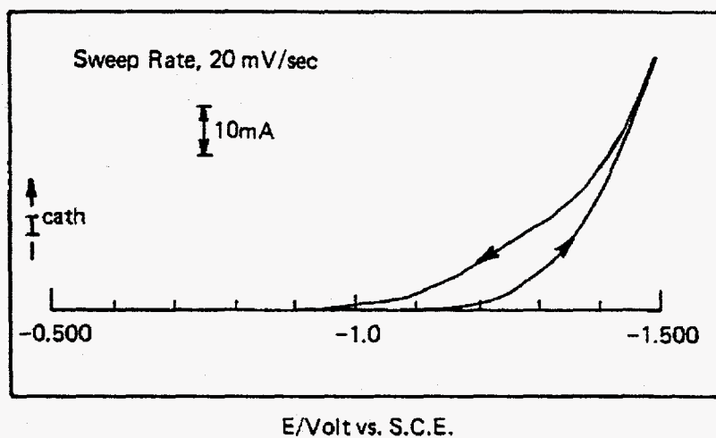
FIGURE 9. Cyclic Voltammogram of 0.39M \text{NaNO}_3 in 3M \text{NaOH} , 0.25M \text{Na}_2\text{CO}_3 at 80°C; Nickel Electrode
