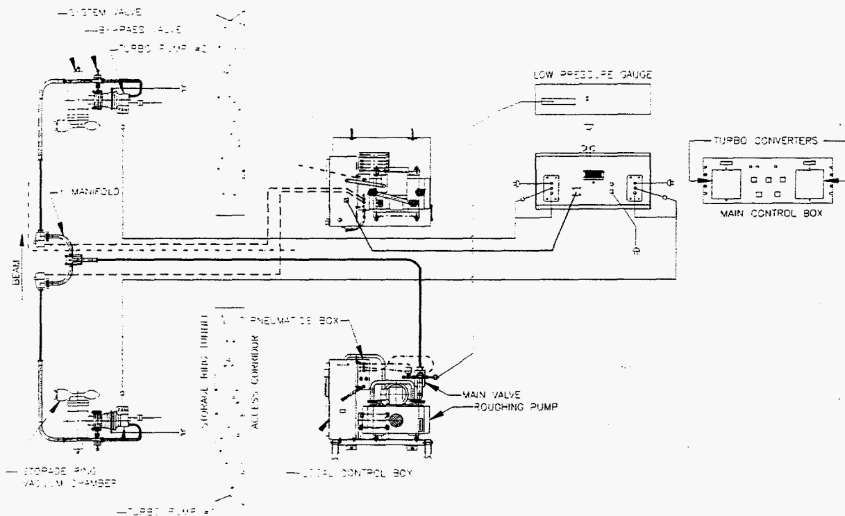
Figure 2: Ancillary pumping system.
