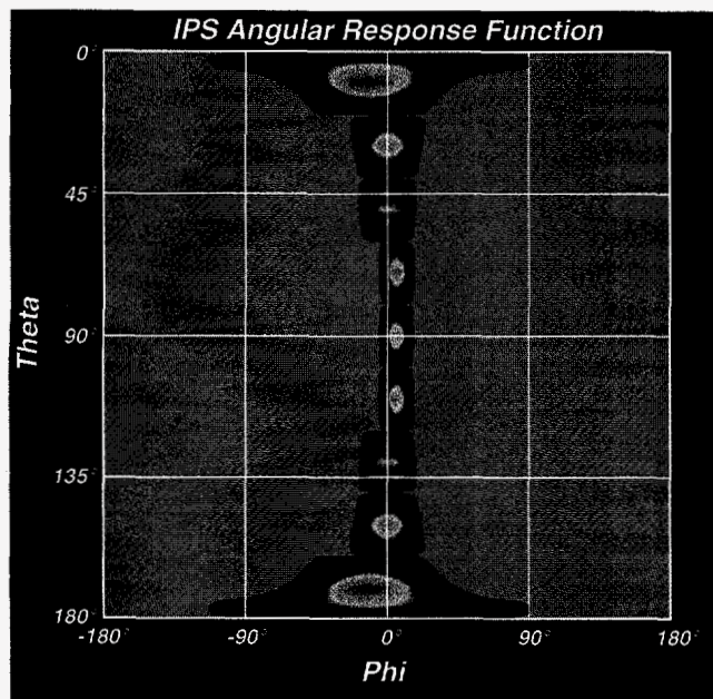
Fig. 2. Effective Angular response of the IPS instrument.
