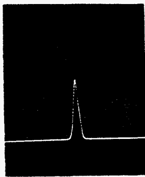
Figure 9.4-2. ^{16}\text{O}_2^- .
