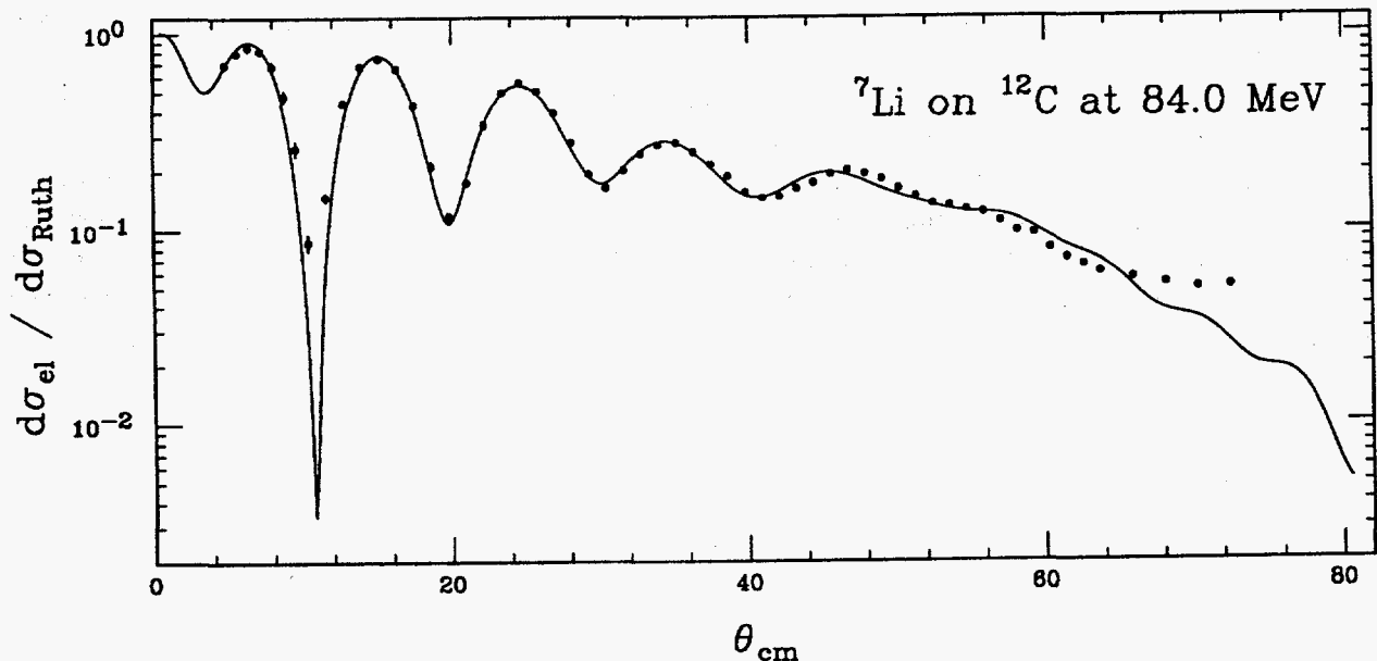
Figure 3.7-1. Elastic scattering angular distribution and optical model fit with Woods-Saxon potentials.
