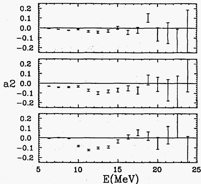
Figure 2.2-1. a_2(E_\gamma) Legendre coefficients of the CM \gamma -ray angular distributions from the reactions ^{18}\text{O} + ^{72}\text{Ge} \rightarrow ^{90}\text{Zr}^* at E_{proj} = 50 (top) and 74 MeV (middle) ^{28}\text{Si} + ^{64}\text{Ni} \rightarrow ^{92}\text{Mo}^* at E_{proj} = 137 MeV (bottom).
