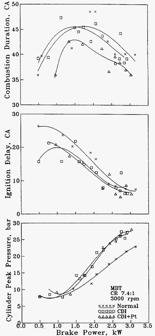
Fig. 7 Combustion characteristics of the high-energy ignition system at the normal compression ratio and 3000 rpm.
