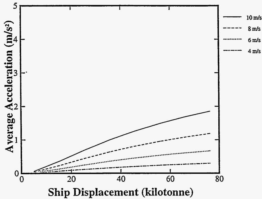
Figure 13. Average Accelerations for the Heavy Cargo Case ( f = 0.5 , \sigma = 1500 MPa)
