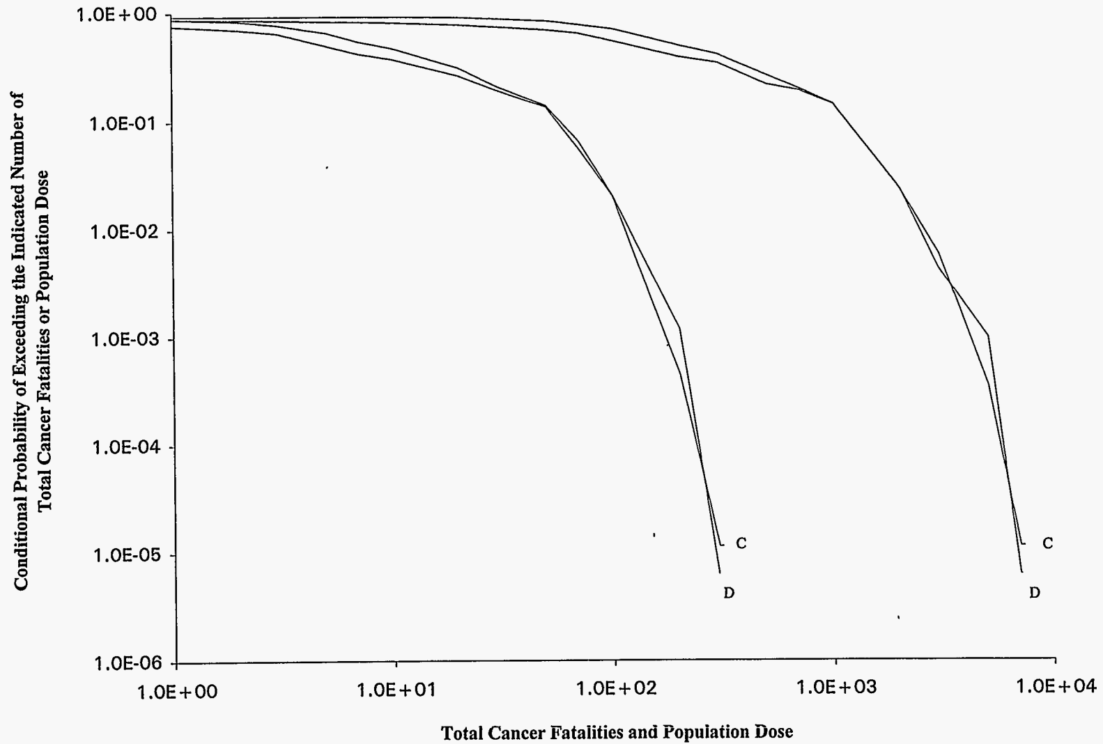
Figure 51. Total Cancer Fatalities and EDE Whole Body Population Dose (Sv), 0-80 km, Savannah Dock (D) and Channel (C) Locations, BR-2 Inventory, EIS6B Release Fractions, Variable Meteorology
