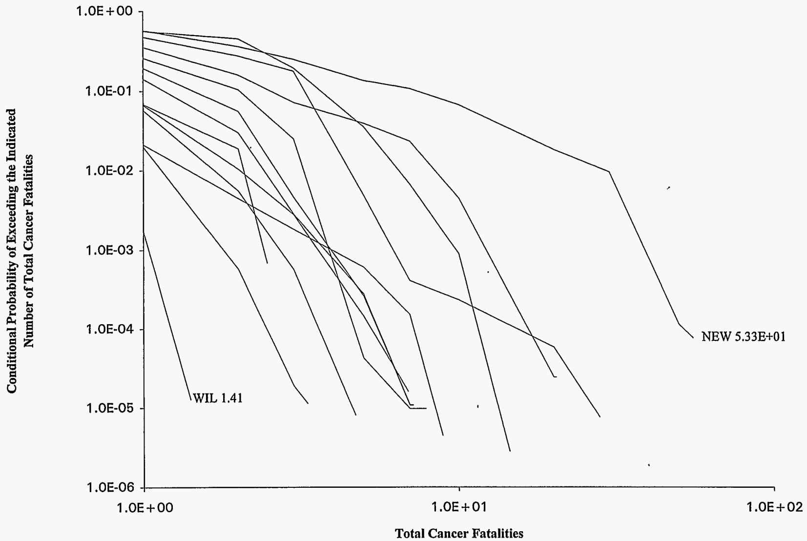
Figure 27. Total Cancer Fatalities, 0-80 km, All Channel Locations, BR-2 Inventory, EA5 Release Fractions, Variable Meteorology
