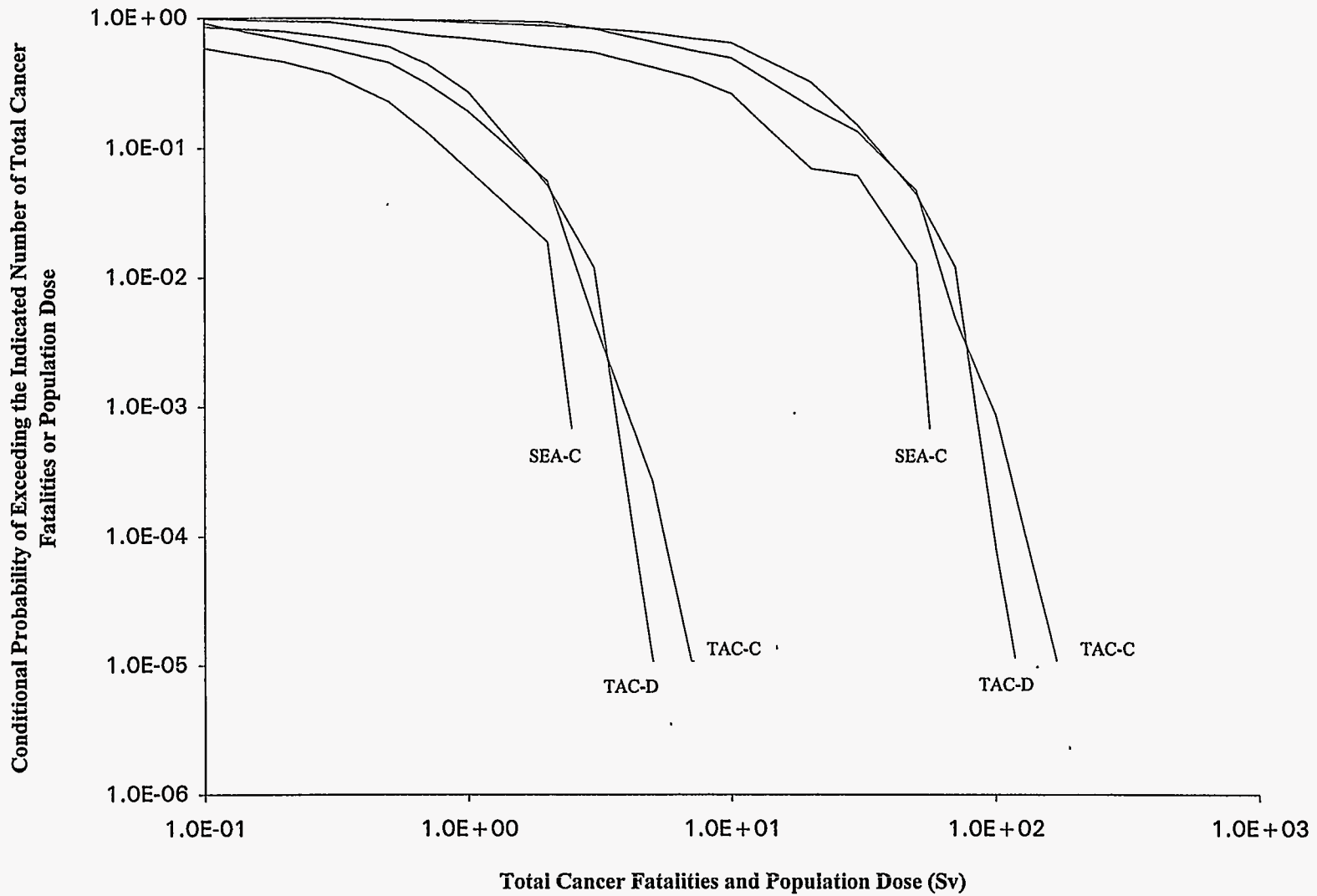
Figure 38. Total Cancer Fatalities and EDE Whole Body Population Dose (Sv), 0-80 km, Tacoma Dock (D) and Channel (C) and Seattle Channel (C) Locations, BR-2 Inventory, EA5 Release Fractions, Variable Meteorology
