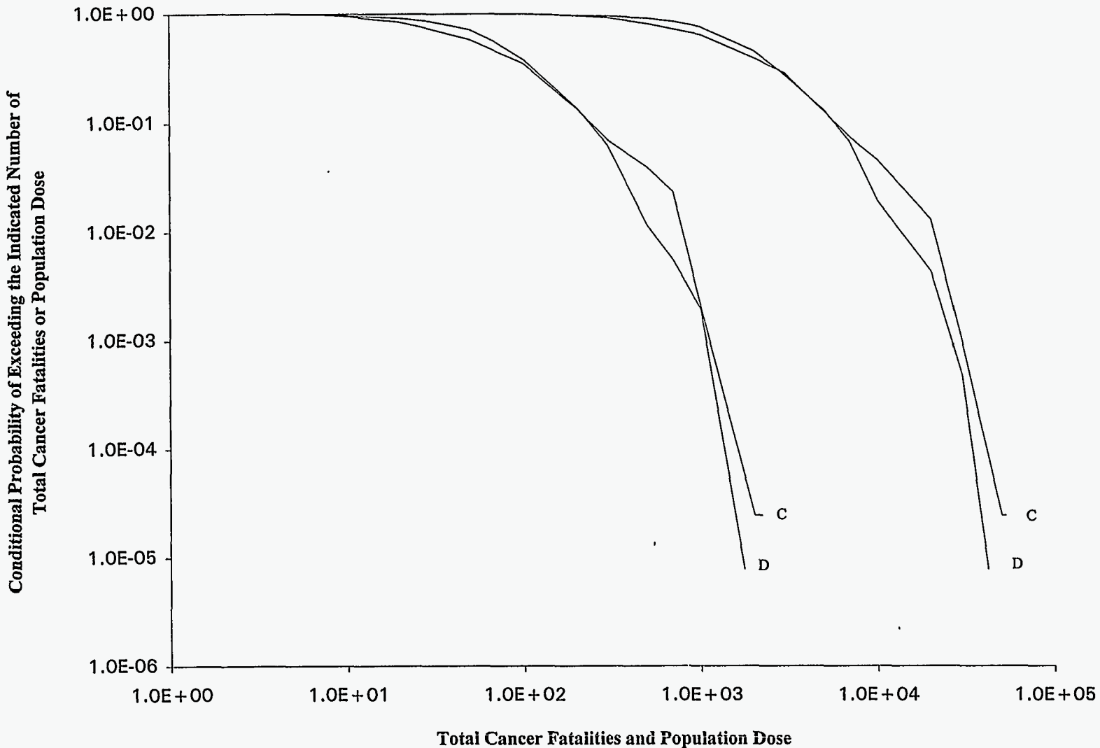
Figure 49. Total Cancer Fatalities and EDE Whole Body Population Dose (Sv), 0-80 km, Philadelphia Dock (D) and Channel (C) Locations, BR-2 Inventory, EIS6B Release Fractions, Variable Meteorology
