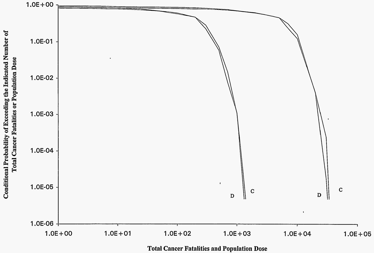
Figure 46. Total Cancer Fatalities and EDE Whole Body Population Dose (Sv), 0-80 km, Los Angeles Dock (D) and Channel (C) Locations, BR-2 Inventory, EIS6B Release Fractions, Variable Meteorology
