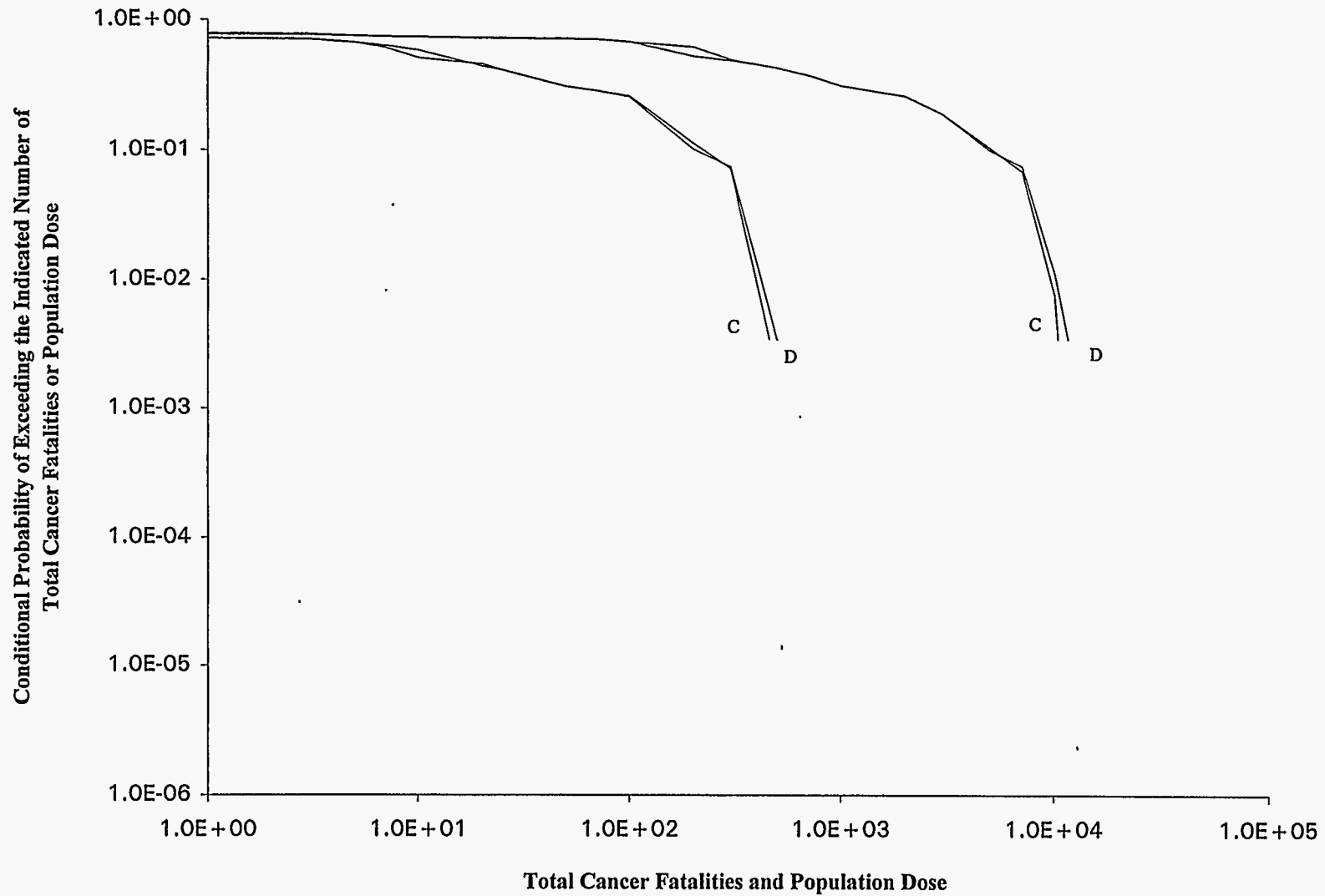
Figure 44. Total Cancer Fatalities and EDE Whole Body Population Dose (Sv), 0-80 km, Galveston Dock (D) and Channel (C) Locations, BR-2 Inventory, EIS6B Release Fractions, Variable Meteorology
