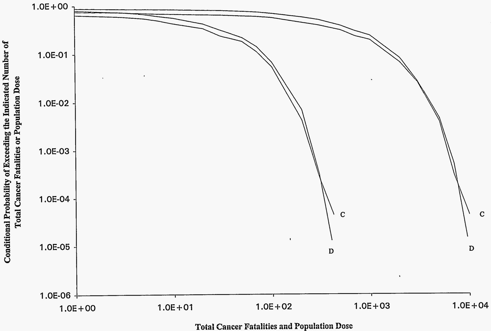
Figure 45. Total Cancer Fatalities and EDE Whole Body Population Dose (Sv), 0-80 km, Jacksonville Dock (D) and Channel (C) Locations, BR-2 Inventory, EIS6B Release Fractions, Variable Meteorology
