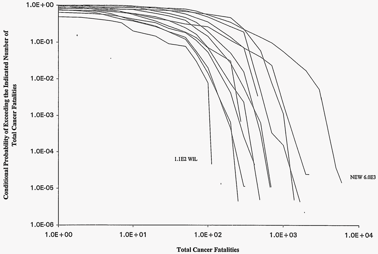
Figure 41. Total Cancer Fatalities, 0-80 km, All Channel Locations, BR-2 Inventory, EIS6B Release Fractions, Variable Meteorology
