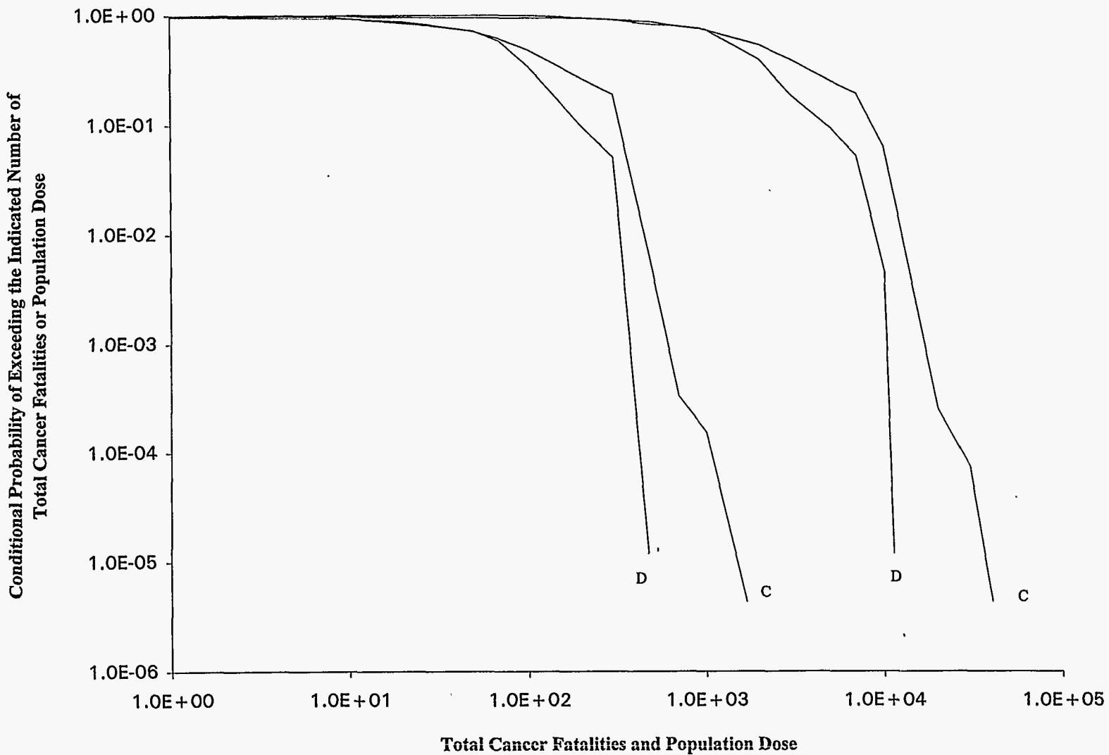
Figure 43. Total Cancer Fatalities and EDE Whole Body Population Dose (Sv), 0-80 km, Concord Dock (D) and (C) Channel Locations, BR-2 Inventory, EIS6B Release Fractions, Variable Meteorology
