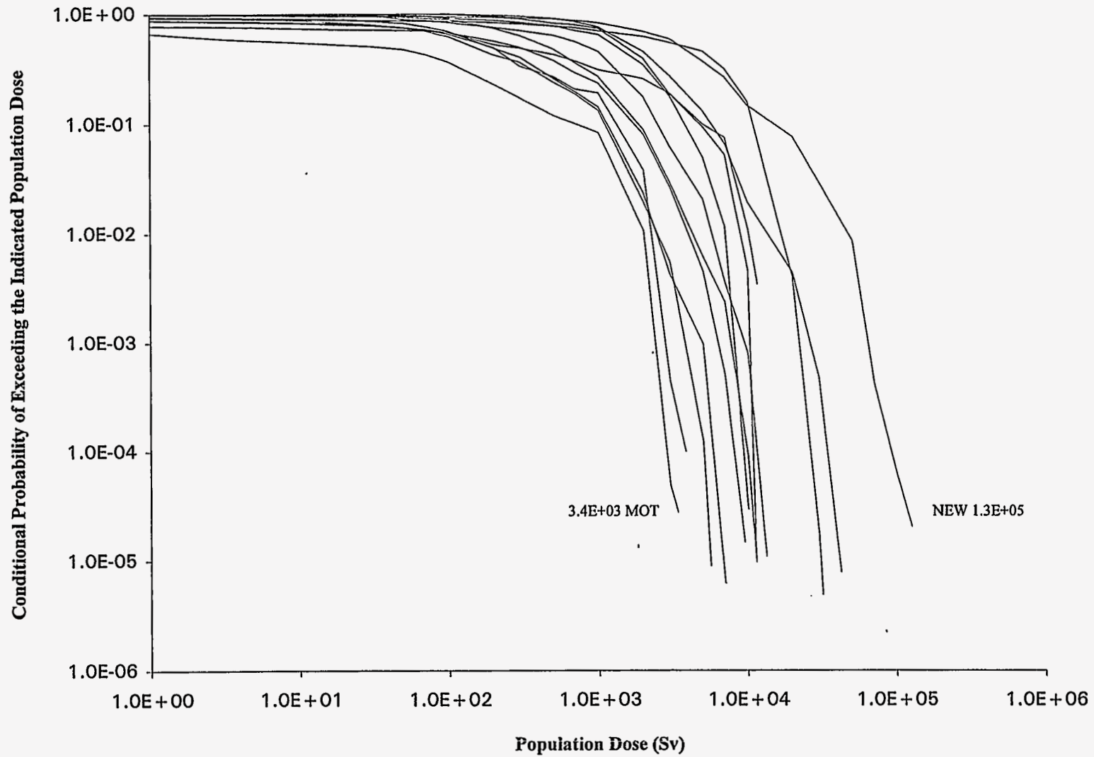
Figure 40. EDE Whole Body Population Dose, 0-80 km, All Dock Locations, BR-2 Inventory, EIS6B Release Fractions, Variable Meteorology
