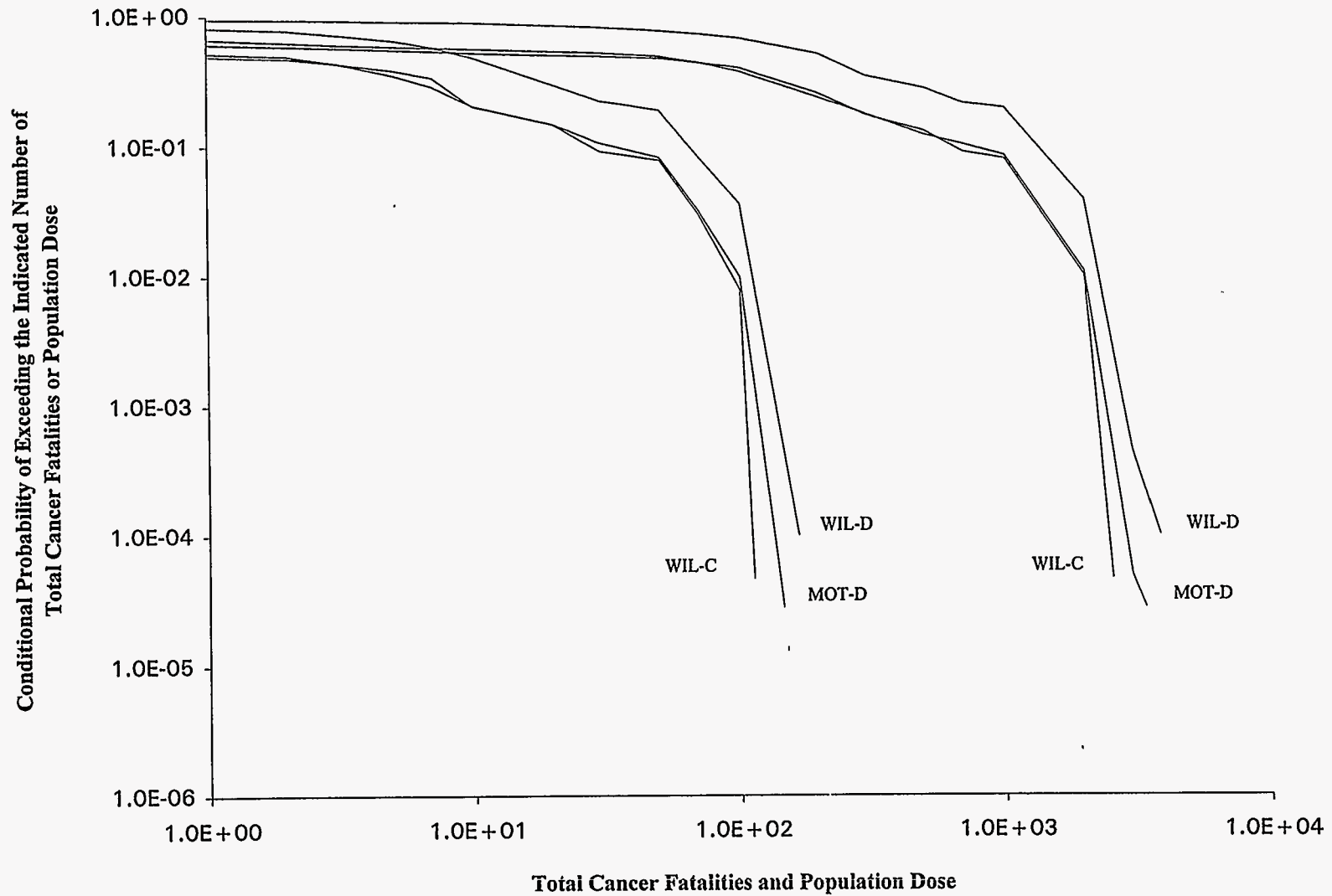
Figure 53. Total Cancer Fatalities and EDE Whole Body Population Dose (Sv), 0-80 km, Wilmington Dock (D) and Channel (C) and MOTSU Dock (D) Locations, BR-2 Inventory, EIS6B Release Fractions, Variable Meteorology
