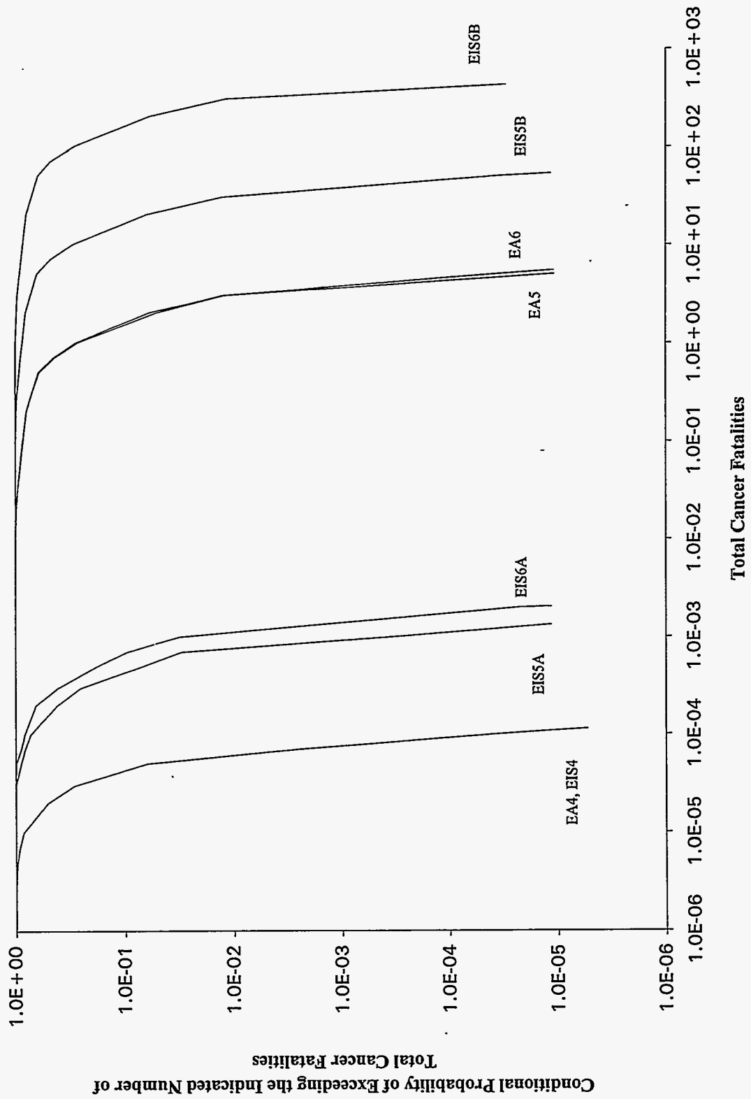
Figure 65. Total Cancer Fatalities, 0-80 km, Tacoma Dock, BR-2 Inventory, All EA and EIS Source Terms, Variable Meteorology
