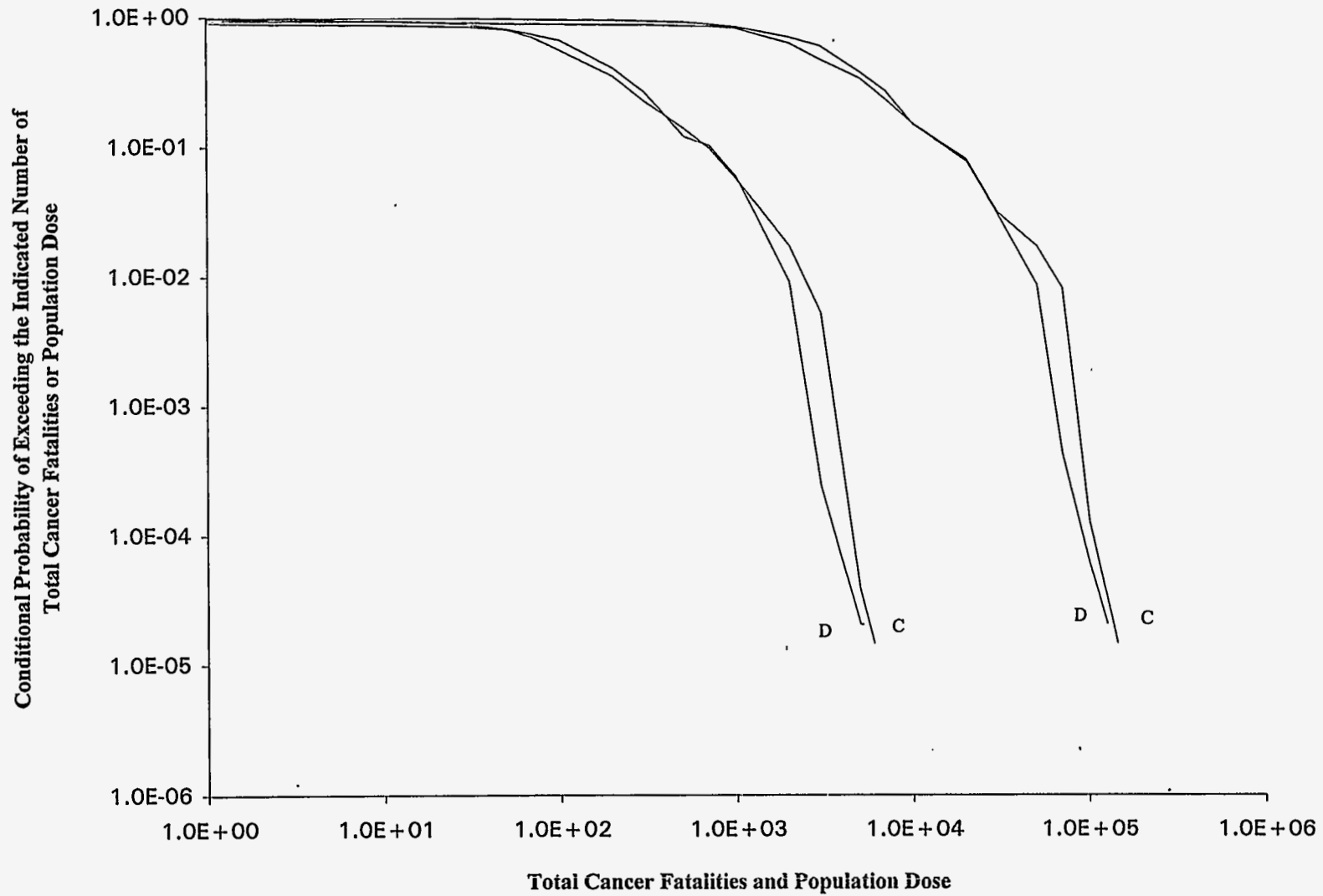
Figure 47. Total Cancer Fatalities and EDE Whole Body Population Dose (Sv), 0-80 km, Newark Dock (D) and Channel (C) Locations, BR-2 Inventory, EIS6B Release Fractions, Variable Meteorology
