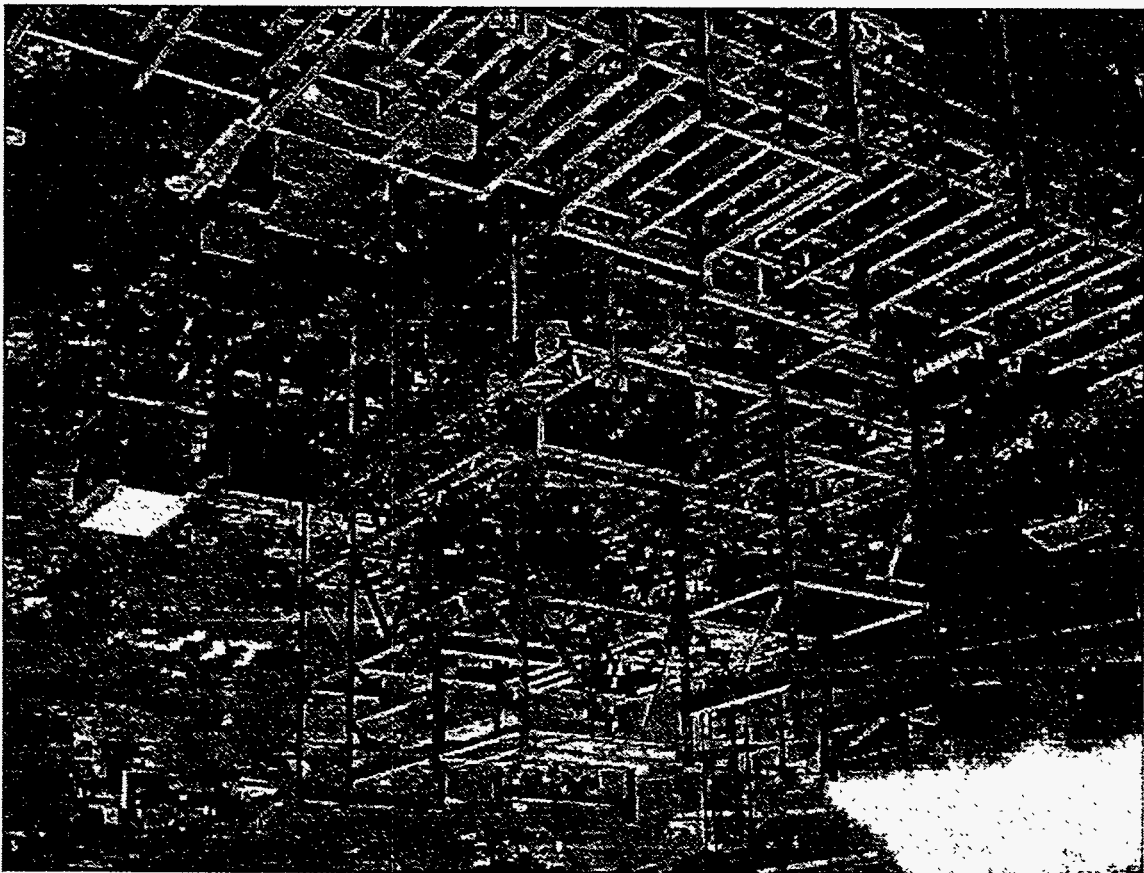
Gasifier Structure to 153' Elevation. Foreground: Pipetack. Top Right: Stacker/Reclaimer Foundation.
