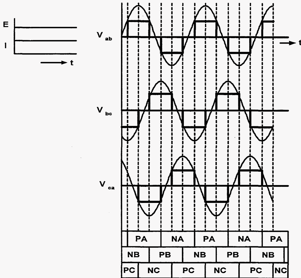
Figure B-15. Waveform and switching sequence for a three-phase, voltage-source inverter.
