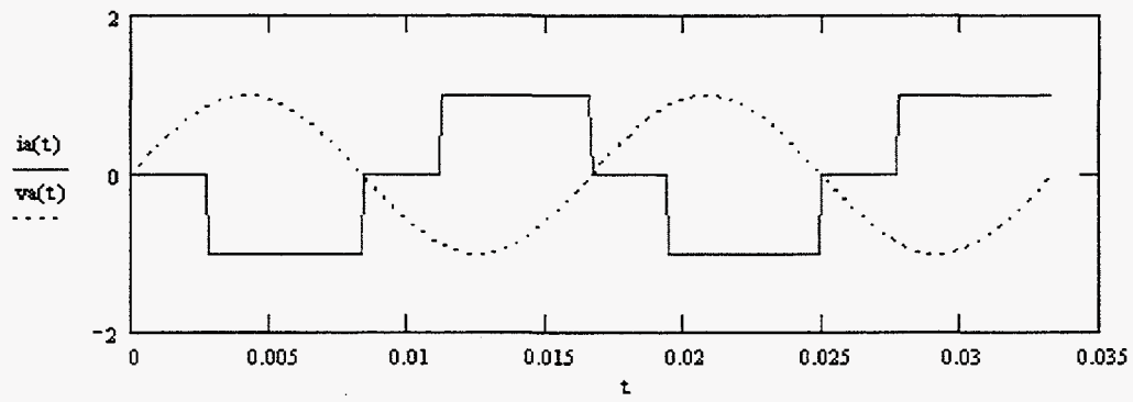
Figure B-19. Waveforms for a three-phase, six-pulse bridge rectifier.
