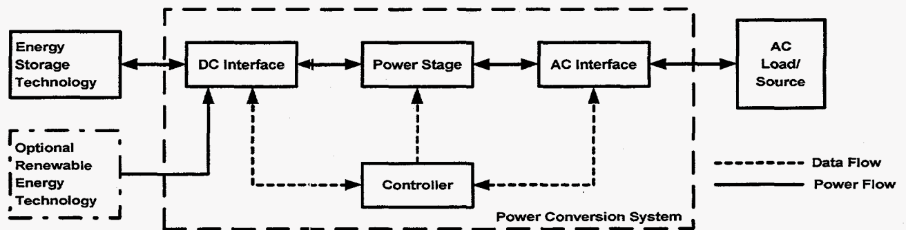
Figure 3. PCS connected to a storage device and an AC load/source.
