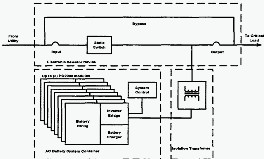
Figure 14. AC Battery PQ2000 configuration.
