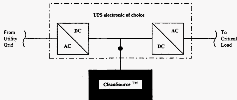
Figure D-2. Power quality glitch protection configuration.
