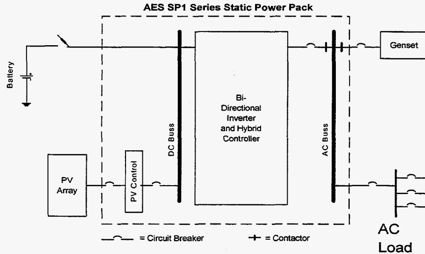
Figure 11. Advanced Energy Systems hybrid inverter design.
