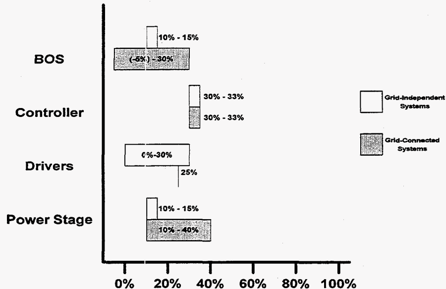
Figure 34. Near-term (within approximately two years) cost reduction potential.
