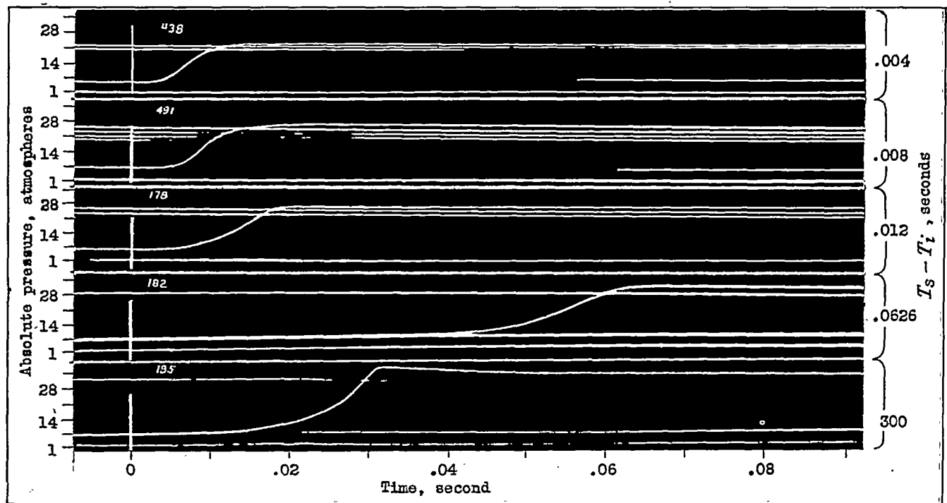
FIGURE 5.—Effect of time interval ( T_s - T_1 ) between injection and spark. Initial air temperature, 200° C.; initial air pressure, 6.3 atmospheres, absolute; air-fuel ratio, 15.
