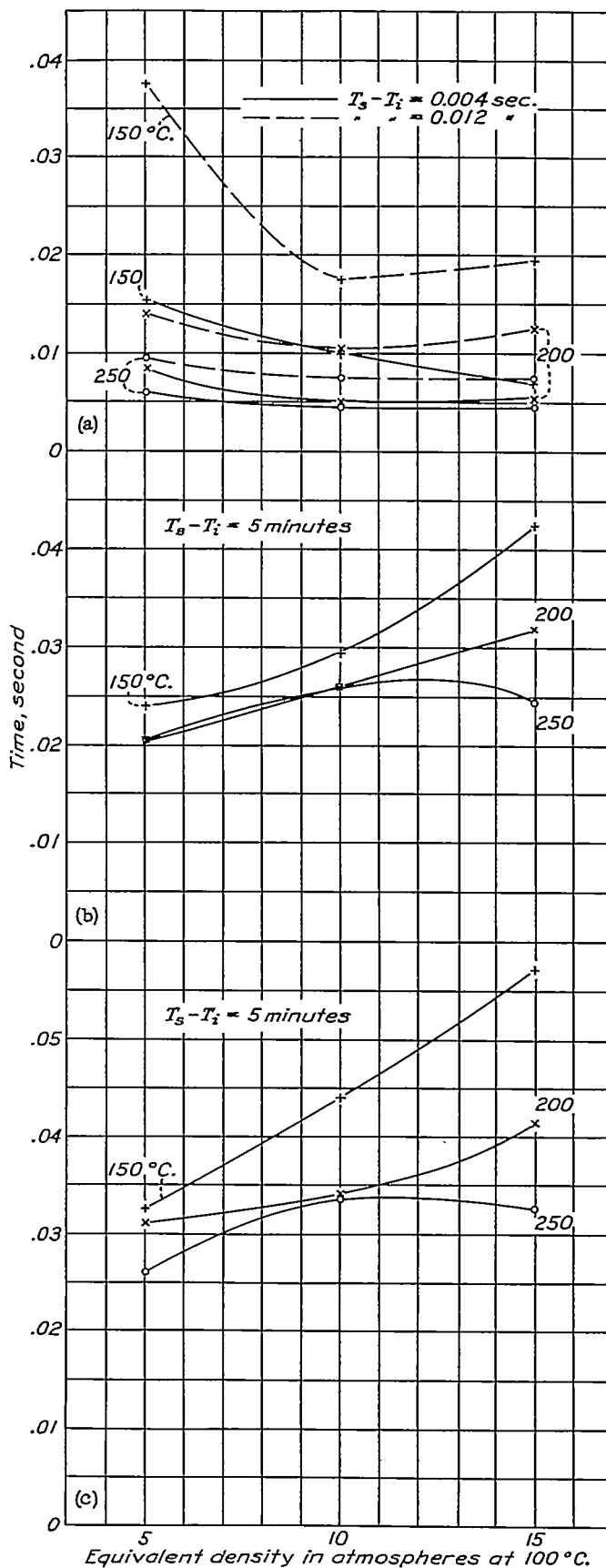
FIGURE 8.—Effect of air density on time of reaction. Air-fuel ratio, 16. (a) Time required for pressure to reach 2.5 P_i . T_s - T_i , 0.004 and 0.012 second. (b) Time required for pressure to reach 2.5 P_i . T_s - T_i , 5 minutes. (c) Time required for pressure to reach maximum. T_s - T_i , 5 minutes.
