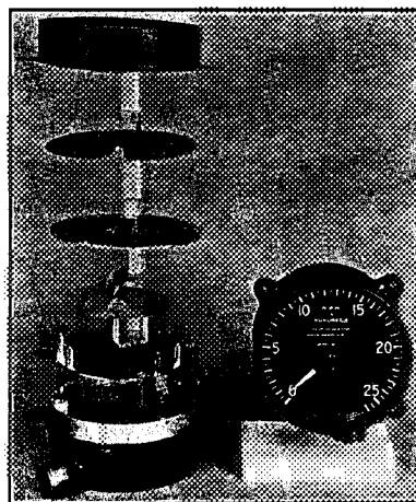
FIG. 47.—Warner magnetic tachometer, airplane type.
