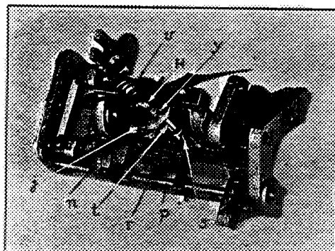
FIG. 20.—Indicating system.
