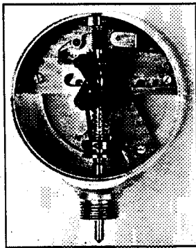
FIG. 39.—Olhovsky mechanism.
