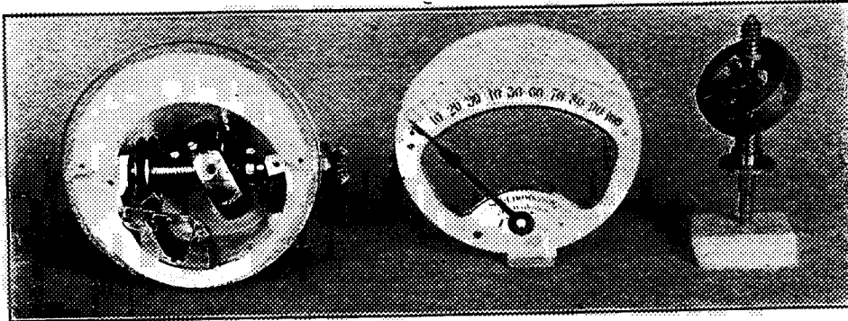
FIG. 34.—Jones Centrifugal Tachometer.
