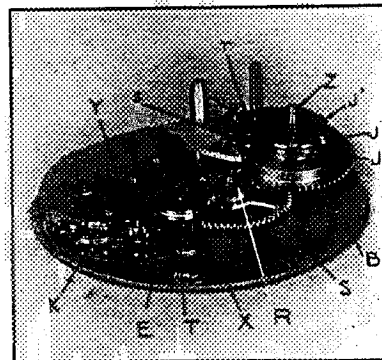
FIG. 10.—Escapement—Cam System.
