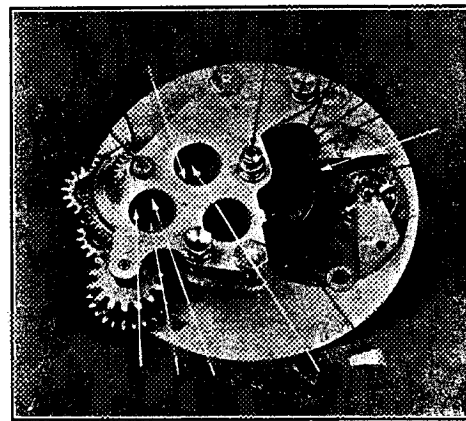
FIG. 8.—Mechanism—Perspective.
