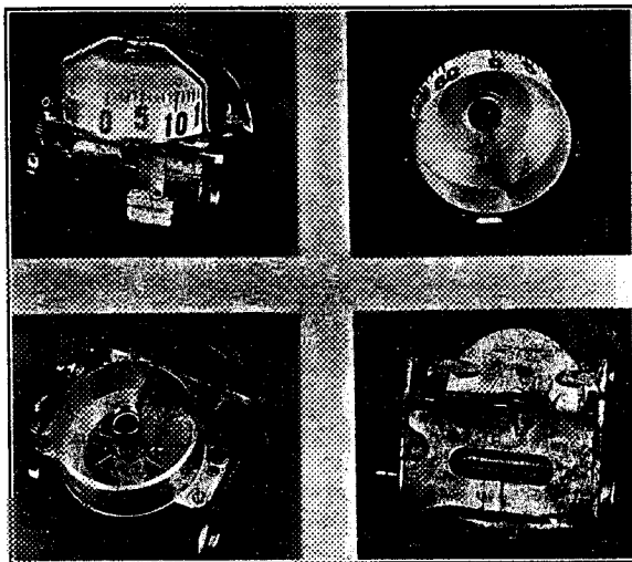
FIG. 44.—Van Sicklen air pump speedometer.
