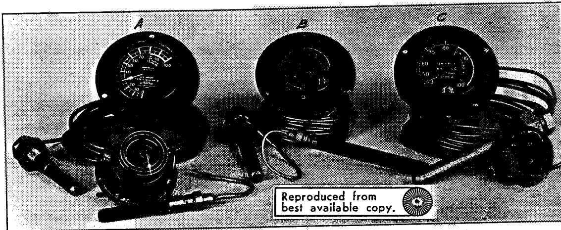
FIG. 1.—Types of thermometers. A. Liquid filled thermometer with long Bourdon tube.
