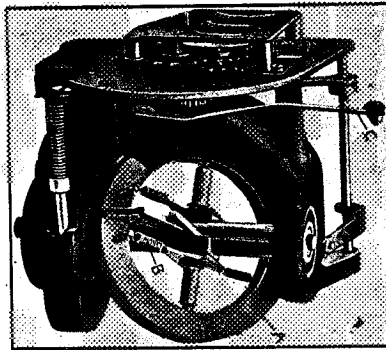
FIG. 38.—Oliver centrifugal mechanism.
