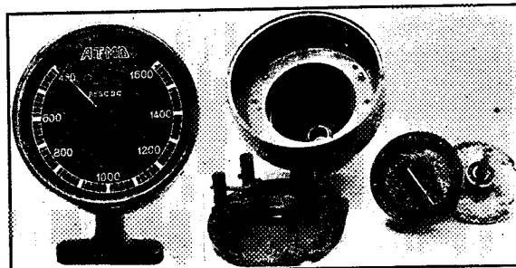
FIG. 49.—Atmo mercury viscosity tachometer.
