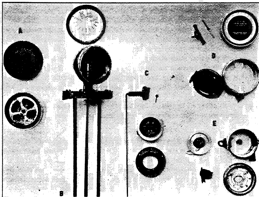
FIG. 2.—Float Type Gasoline Depth Gages—Disassembled.
