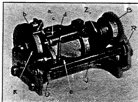
FIG. 18.—Escapement system.
