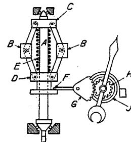
FIG. 28.—Governor type.
