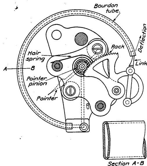
FIG. 1.—Pressure gage.
