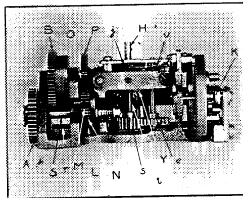
FIG. 14.—Side View.
