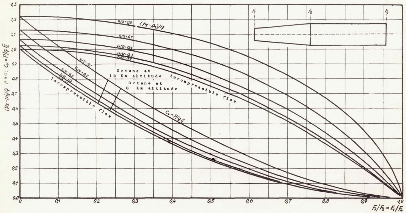
Figure 8.- Jet tube without discharge nozzle; pressure wire in diffuser and coefficient of propulsion c_v .
