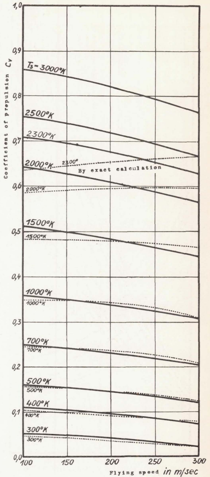
Figure 5.- Propulsive efficiency of jet tube at T_1 = 216.5 K (stratosphere) by approximation (solid line) and by exact calculation (dotted lines).
