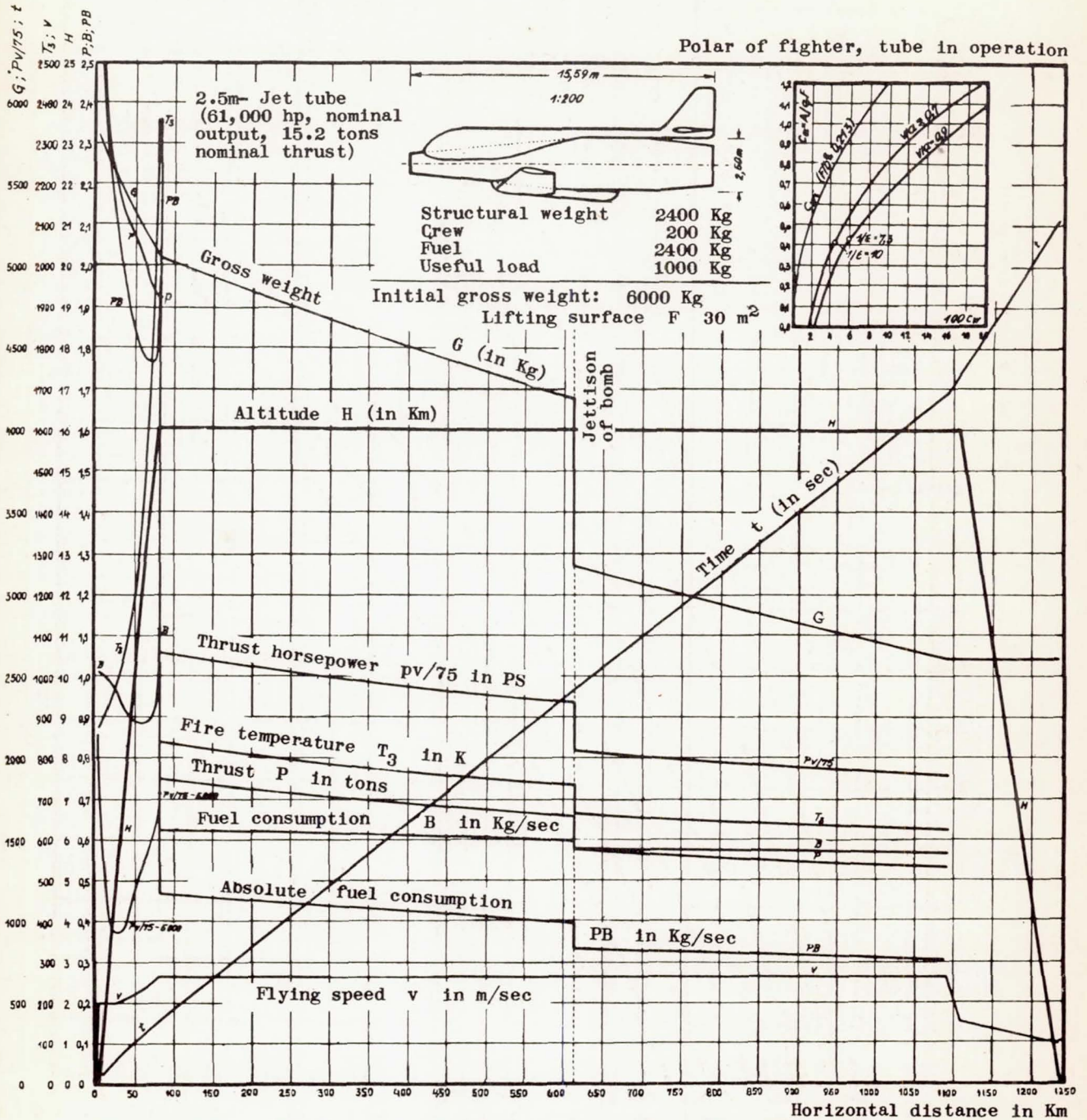
Figure 34.- Flight path of jet fighter used as level bomber gives at 1000 Kg useful load and 16 Km altitude about 430 Km depth of penetration.
