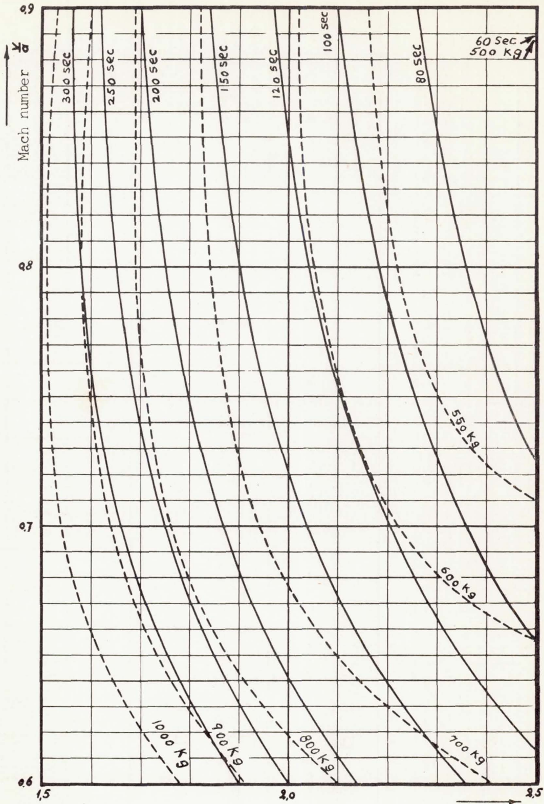
Figure 32a.- Actual time of ascent of jet fighter to 12,000 m altitude and relative fuel consumption plotted against flying speed v and tube diameter d_2 .
