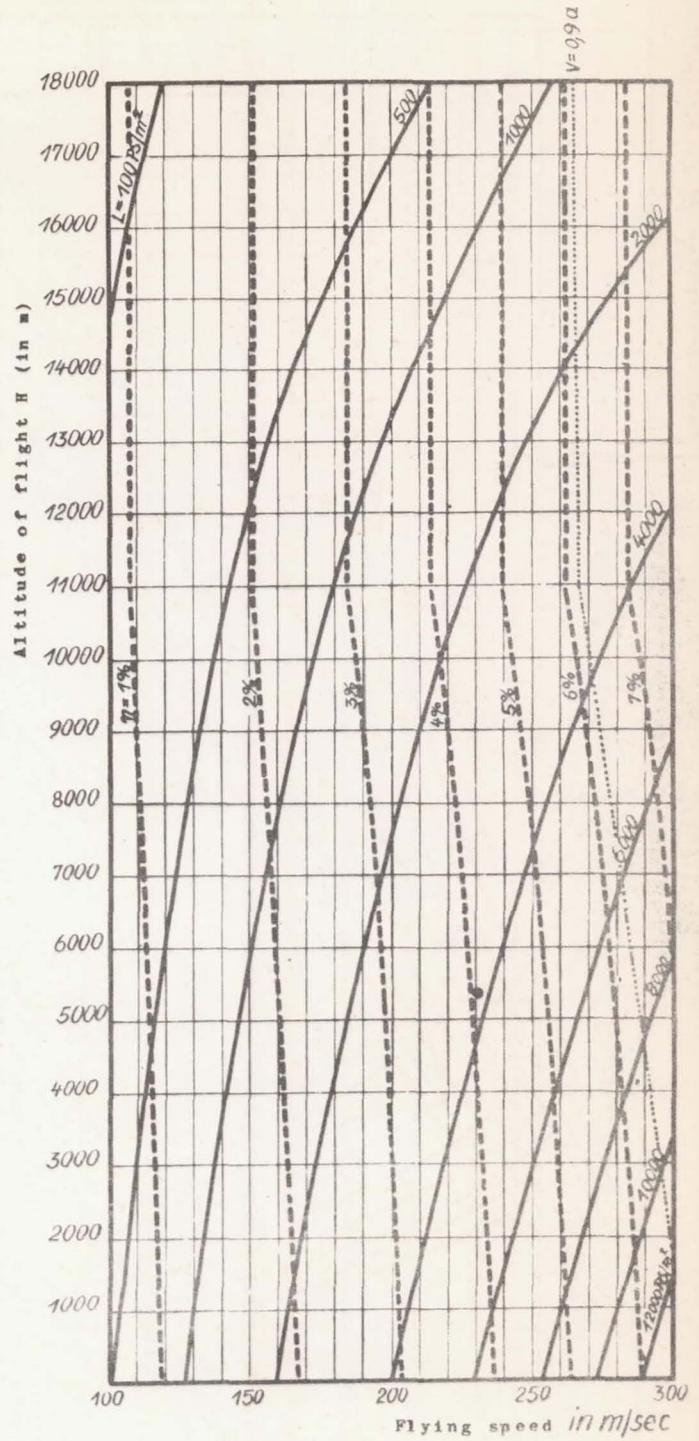
Figure 7.- Maximum thrust horsepower per m^2 of maximum cross-sectional area L/F_2 ( HP/m^2 ) and the respective efficiency \eta for stoichiometric hydrocarbon combustion.
