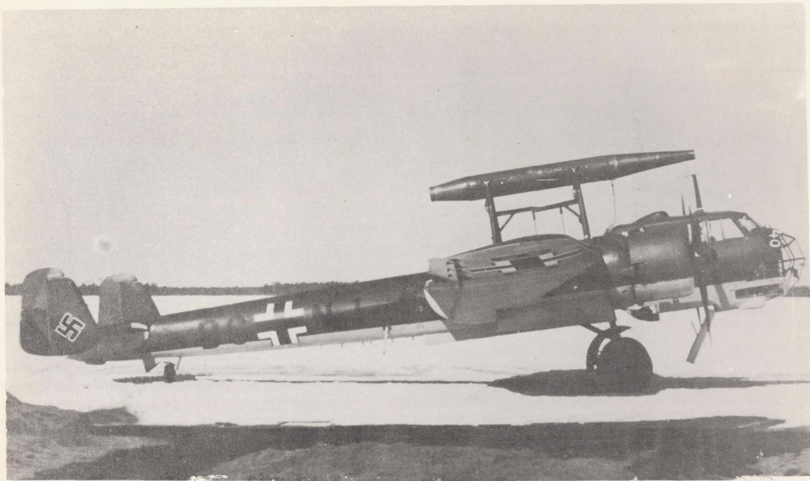
Figure 21.- 2400-hp jet tube on the Do 17Z as experimental carrier.
