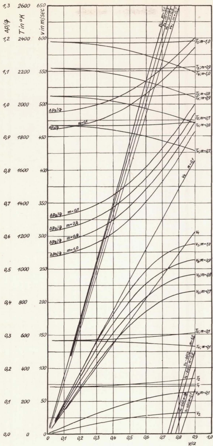
Figure 11.- Phase quantities \Delta p/q , T and v in the four maximum cross sections F_1, F_2, F_3 , and F_4 of a jet tube with the dimensions F_1/F_2 = 0.16 plotted against the flying speed v/a at 0 Km flight level and with respect to the fuel volume factor m .
