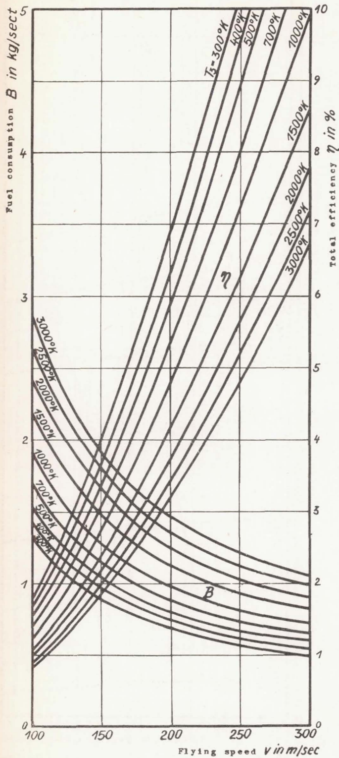
Figure 4.- Efficiency and fuel consumption of jet tube at T_1 = 216.5 K (stratosphere) by approximate method.
