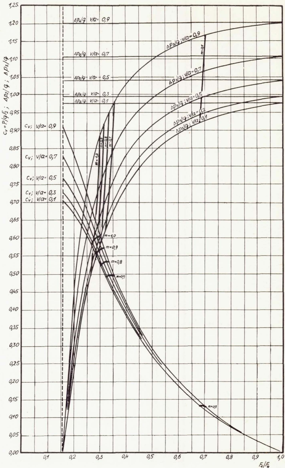
Figure 14.- Coefficients c_v , excess pressures \Delta p_2/q and \Delta p_3/q at 4 Km flight altitude for a jet tube with the dimensions F_1/F_2 = 0.16 for different hydrocarbon-air mixtures plotted against cross section ratio F_1/F_4 .
