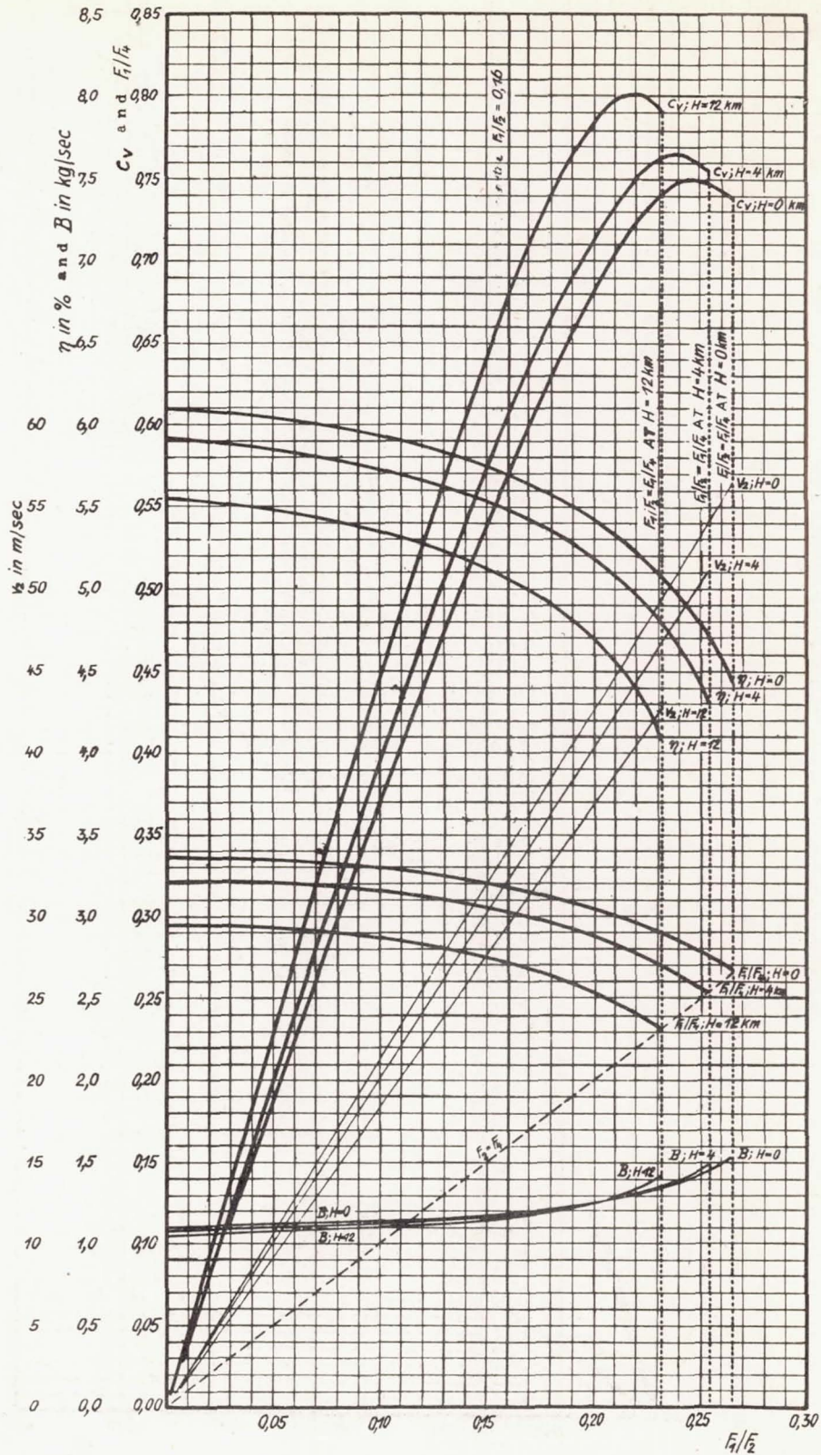
Figure 10.- Coefficient of propulsion c_v (-), efficiency (%), cross-section ratio F_1/F_4 (-) and fuel consumption B (Kg/sec) plotted against ratio F_1/F_2 for v/a = 0.9 and stoichiometric octane-air combustion at 0.4 and 12 Km altitude.
