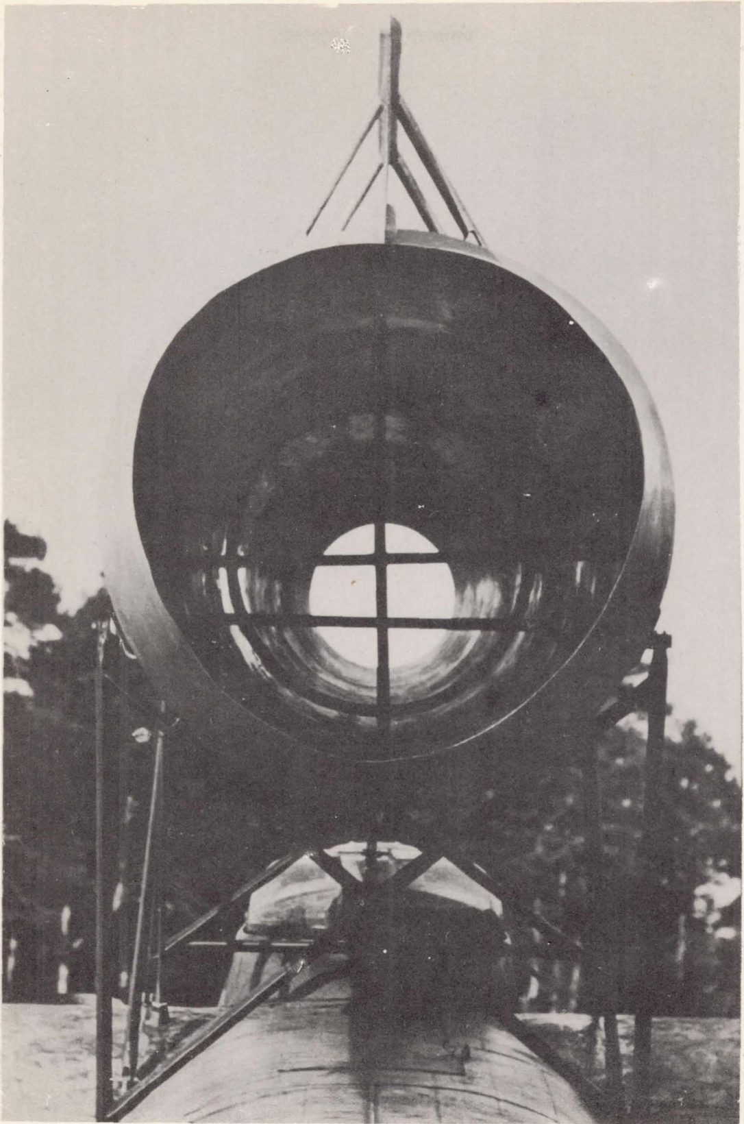
Figure 26.- Interior view showing injection cross from rear. 20,000-hp jet tube mounted on Do. 217E2.
