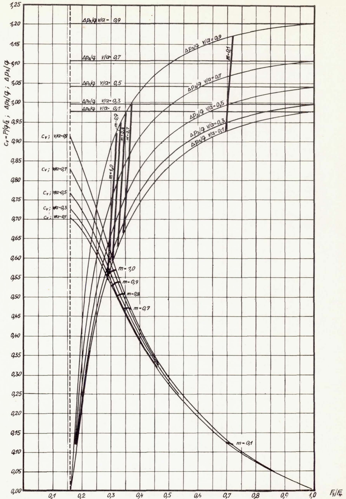
Figure 12. Coefficients c_v , excess pressures \Delta p_2^2/q and \Delta p_3/q at 0 Km height for a jet tube with the dimensions F_1/F_2 = 0.16 for various hydrocarbon-air mixtures plotted against the cross section ratio F_1/F_4 .
