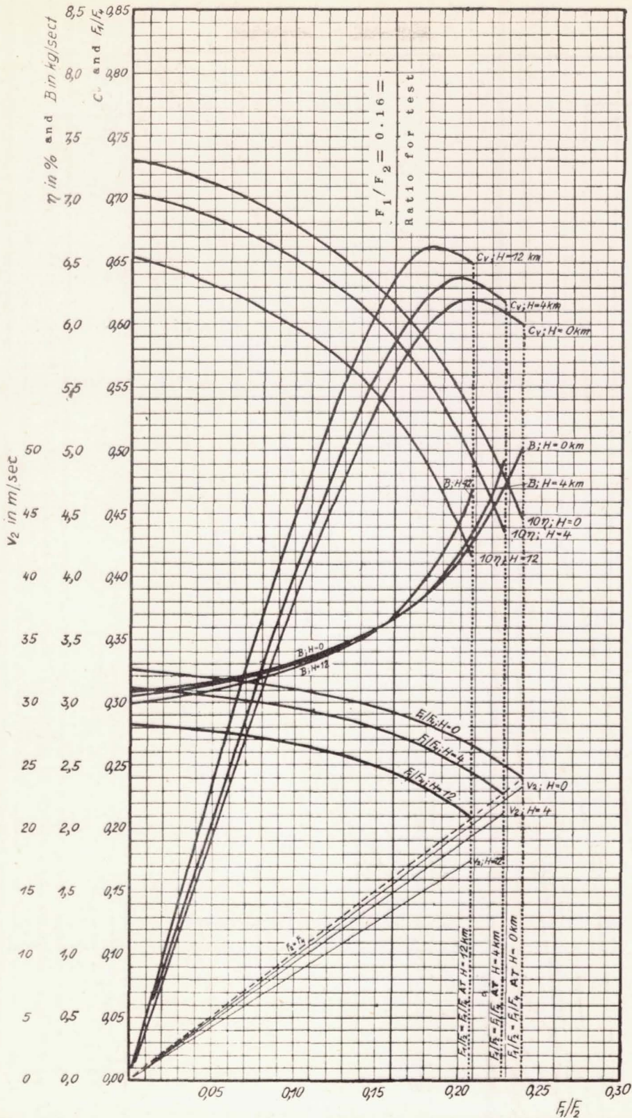
Figure 9.- Coefficient of propulsion c_v (-), efficiency (%), cross-section ratio F_1/F_4 (-) and fuel consumption B (Kg/sec) plotted against ratio F_1/F_2 for v/a = 0.3 and stoichiometric octane-air combustion at 0.4 and 12 Km altitude.
