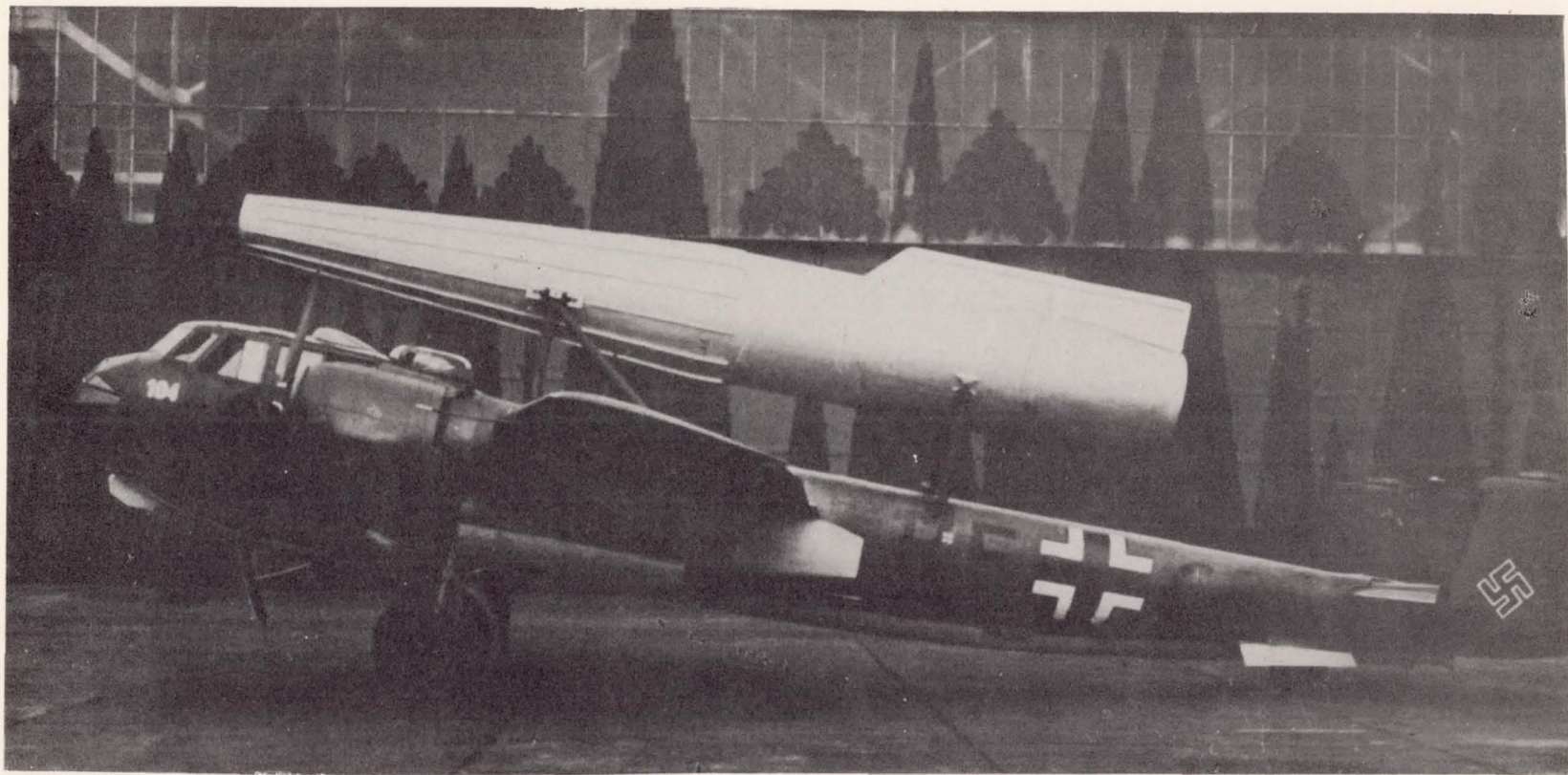
Figure 25.- Side view of 20,000-hp jet tube mounted on the Do. 217E2 as test carrier.
