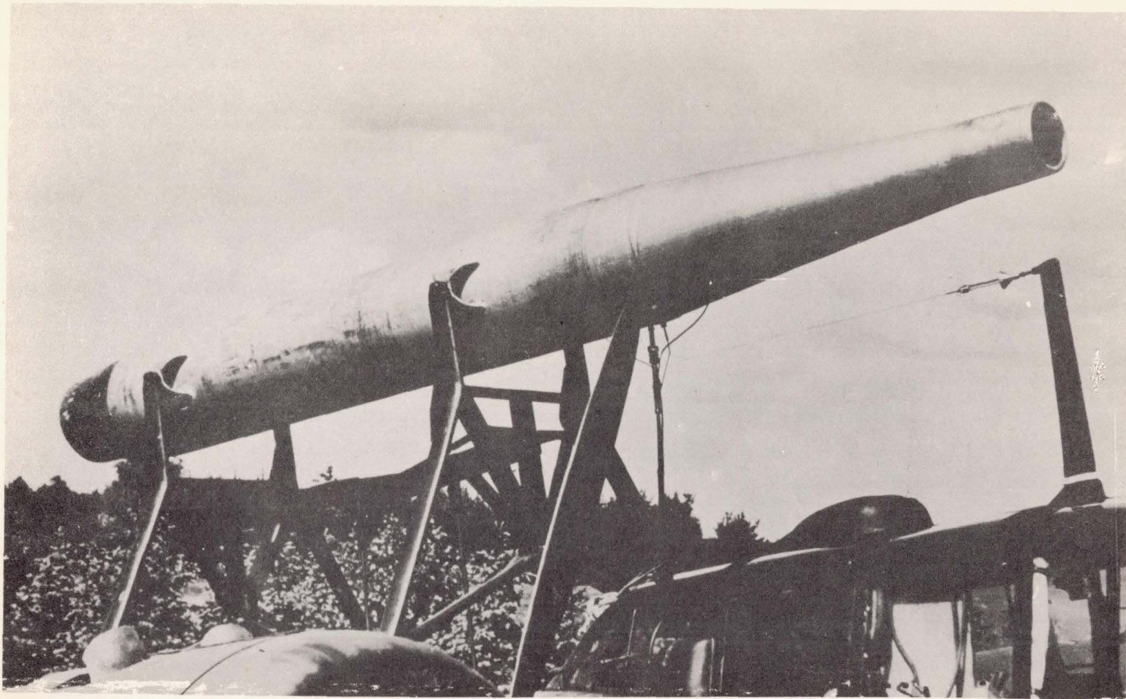
Figure 22.- 2400-hp jet tube and thrust recording setup on the Do. 17Z.
