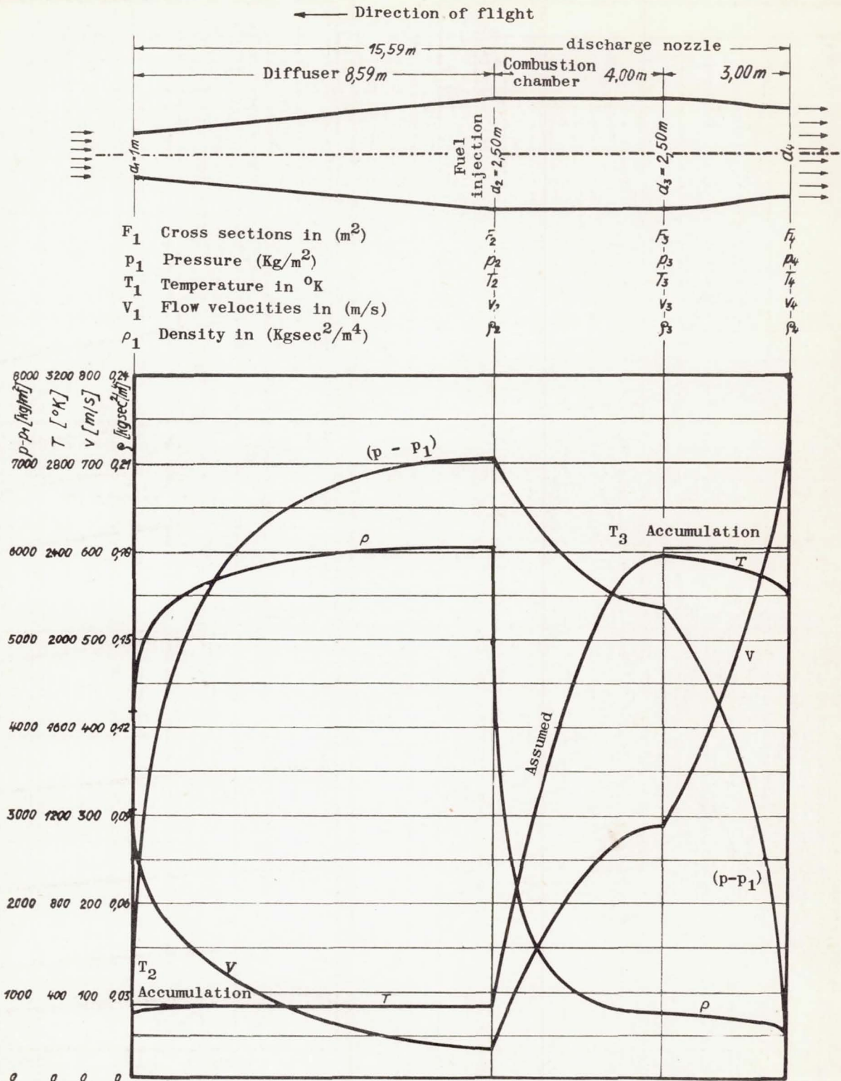
Figure 1.- Jet tube of 2.5m diameter at flight near sea level with stoichiometric gasoline consumption and 1100 Km/h ( v/a = 0.9 ) flying speed. (Thrust: 16.4 tons, thrust coefficient: c_v = 0.57 ; gasoline consumption: 1.19 Kg/sec t; efficiency: 5.7%; thrust horsepower: 67,000 hp.)
