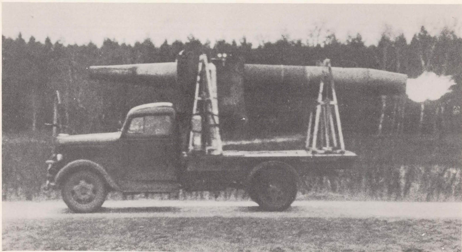
Figure 20.- Road towing test with high-temperature jet tube for measuring the diffuser efficiencies.
