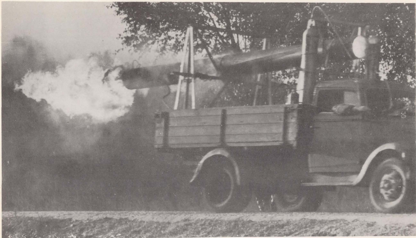
Figure 18.- Road towing test with Lorin combustion chamber for studying the injection and combustion processes.
