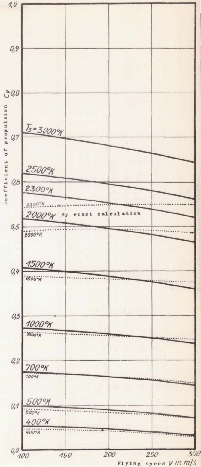
Figure 3.- Propulsive efficiency of jet tube at T_1 = 288^\circ\text{K} (sea level) by approximate method (solid curve) and by exact calculation (dotted line).
