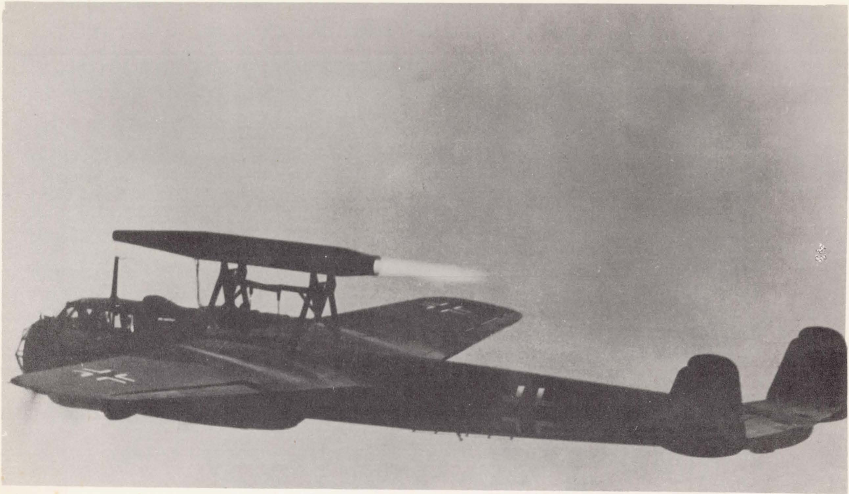
Figure 24. 2400hp jet tube with v=85\text{m/sec.} in operation.
