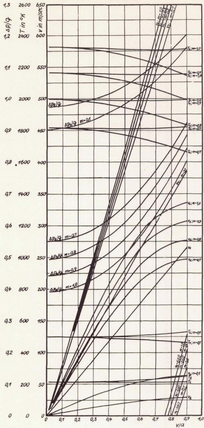
Figure 15.- Quantities \Delta p/q, T and v in four maximum cross sections F_1, F_2, F_3, F_4 , of a jet tube with the dimensions F_1/F_2 = 0.16 plotted against the flying speed v/a at 12 Km altitude and fuel volume factor m .
