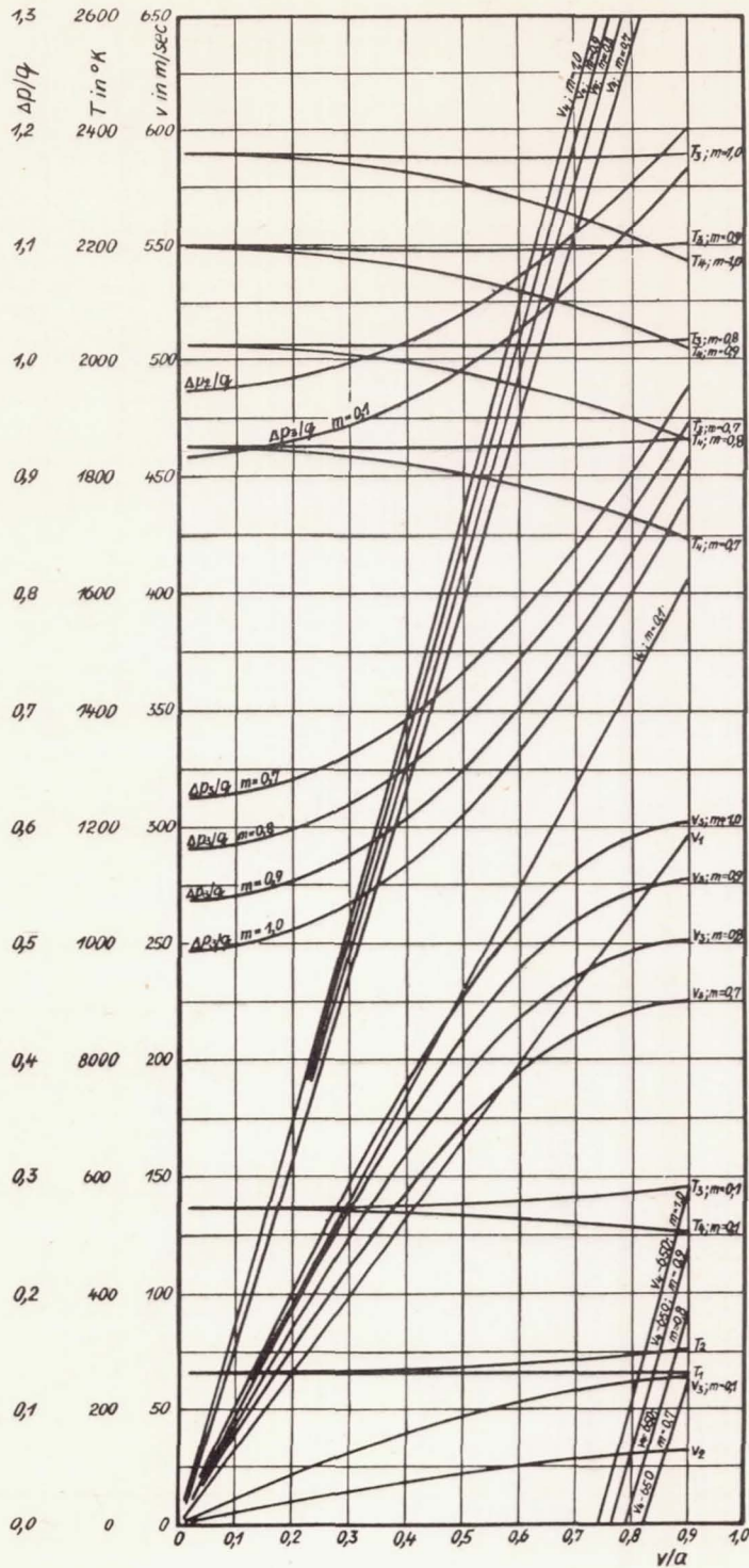
Figure 13.- Phase quantities \Delta p/g , T and v in the four maximum cross sections F_1, F_2, F_3, F_4 , of a jet tube with the dimensions F_1/F_2 = 0.16 plotted against fly-ing speed v/a at 4 Km flight altitude and fuel-volume factor m .
