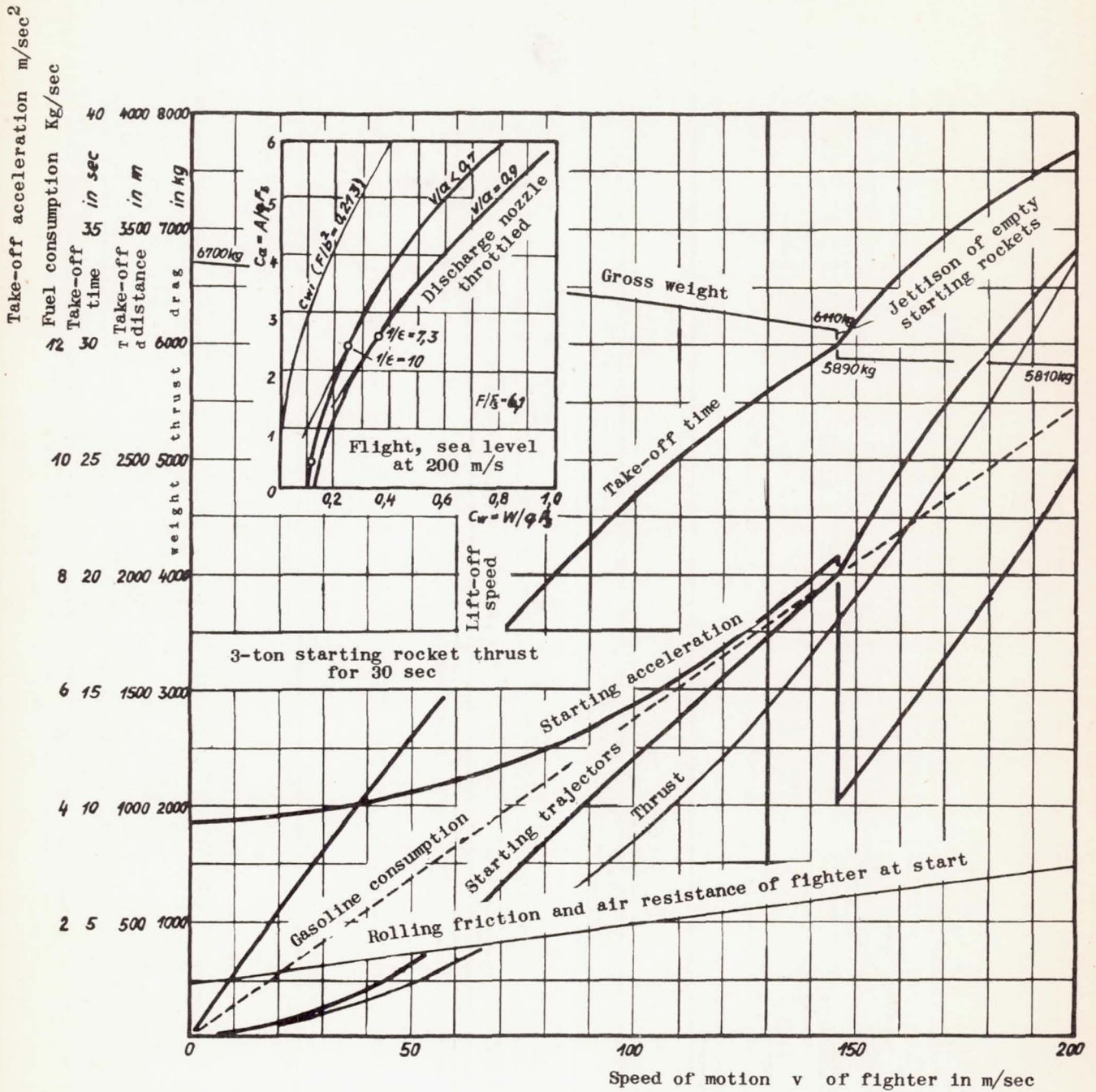
Figure 31.- Estimated polars and take-off conditions of jet fighter.
