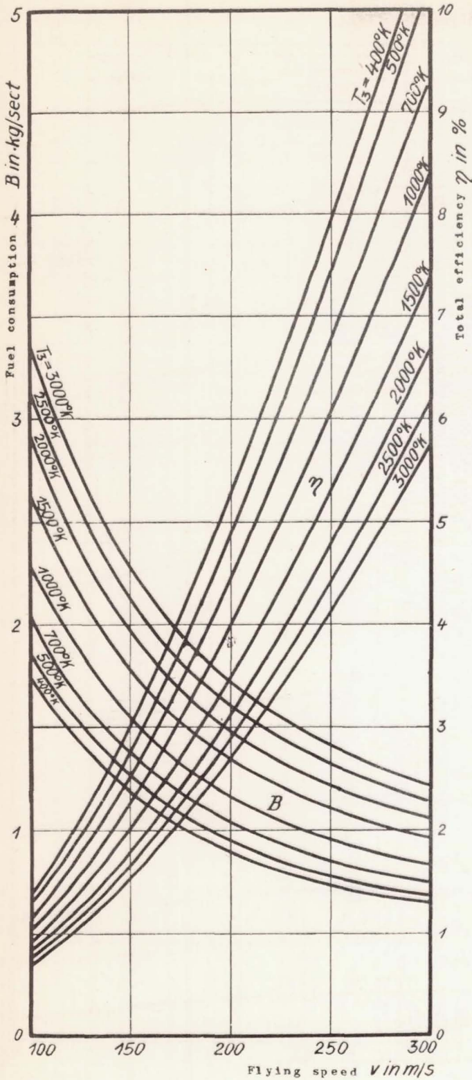
Figure 2.- Efficiency and fuel consumption of jet tube at T_1 = 288^\circ\text{K} (near sea level) by approximation.
