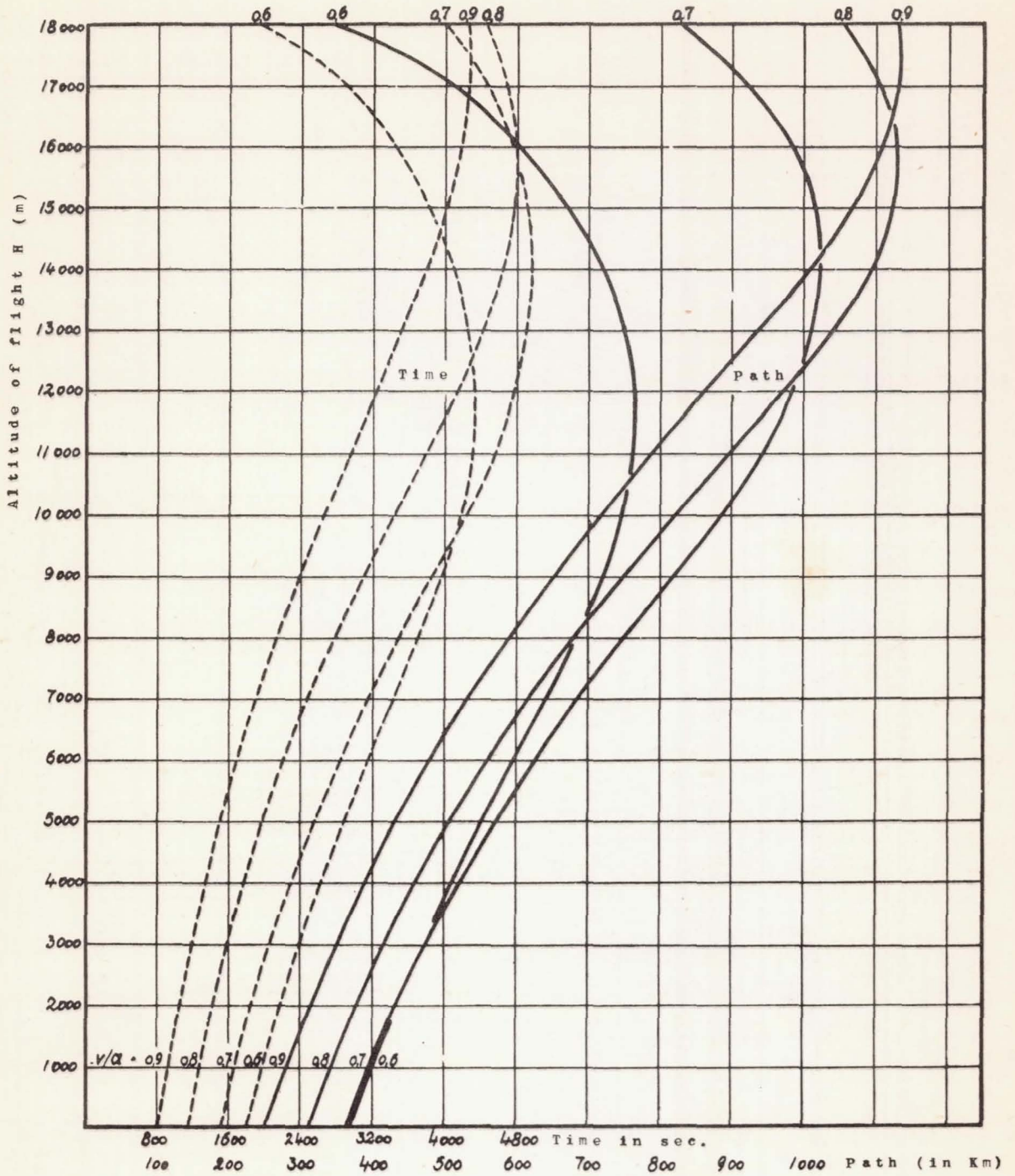
Figure 33. Conditions of horizontal flight.
