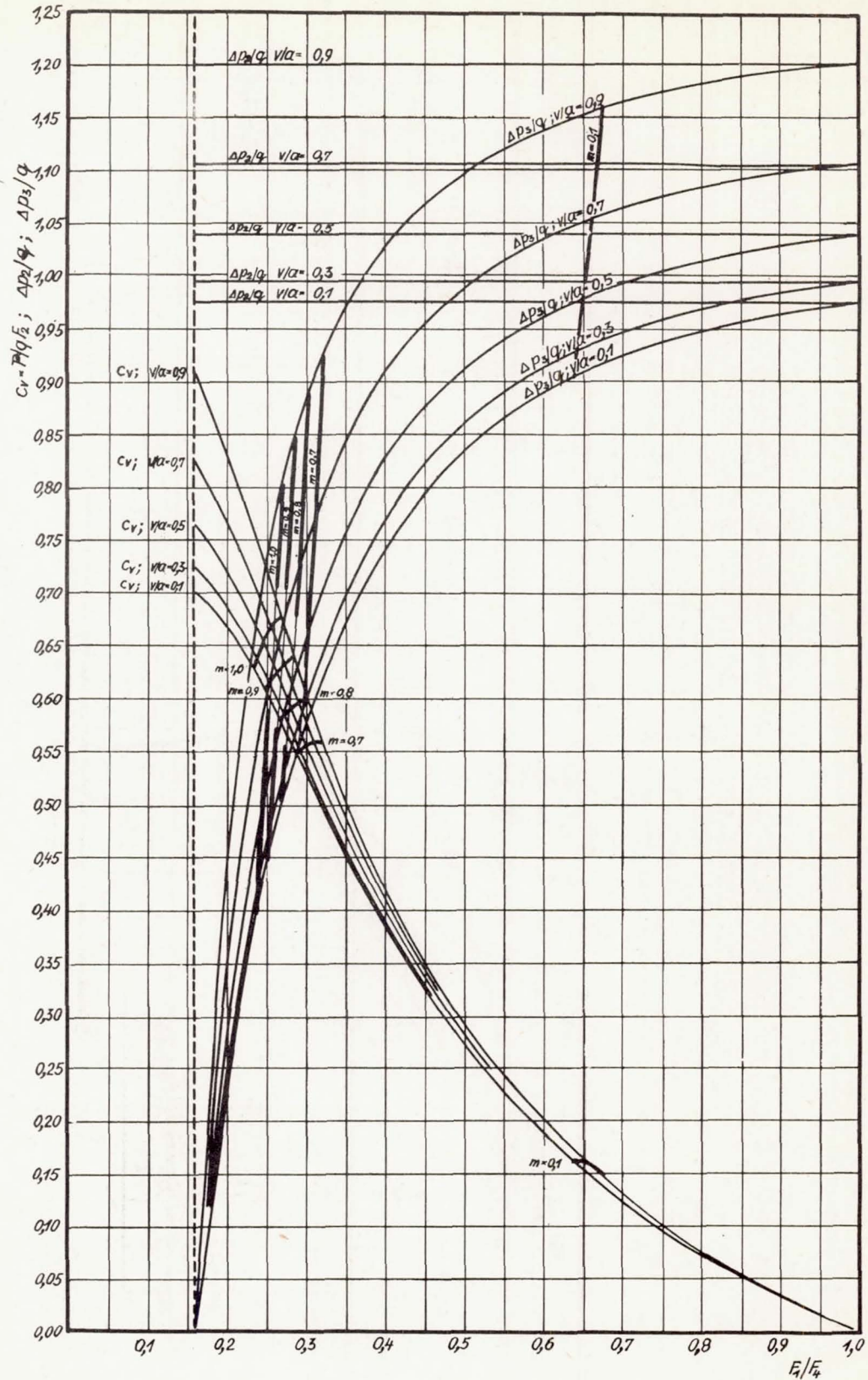
Figure 16. Coefficients c_v , excess pressures \Delta p_2/q and \Delta p_3/q at 12 Km altitude for a jet tube with the dimensions F_1/F_2=0.16 for various hydrocarbon-air mixtures plotted against the cross-section ratio F_1/F_4 .
