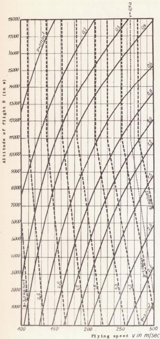
Figure 6.- Maximum thrust per m^2 of maximum cross-sectional area P/F_2 ( t/m^2 ) and the respective fuel consumption B ( Kg/sect ) for stoichiometric hydrocarbon combustion.
