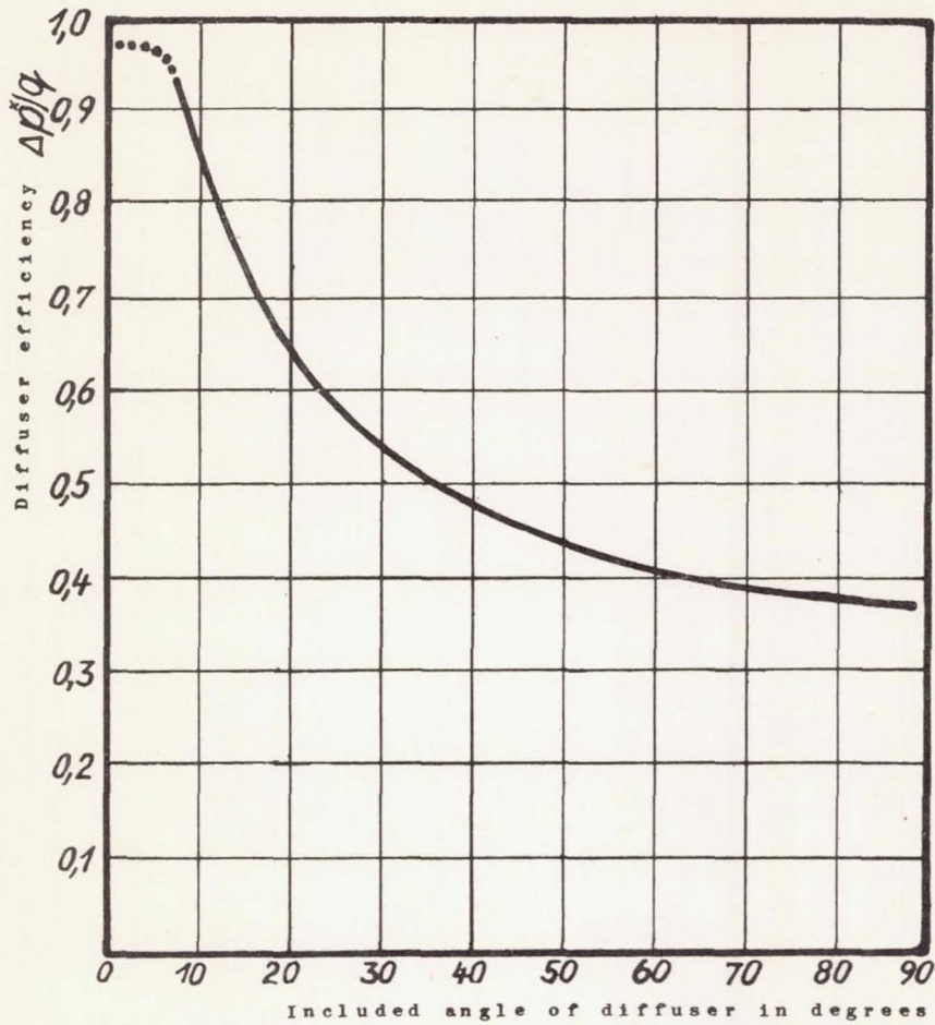
Figure 17. Diffuser efficiency \Delta p_2^x/q plotted against included angle according to towing tests with high-temperature jet tubes at v_1=20 m/sec and F_2/F_1 = 6.25 .
