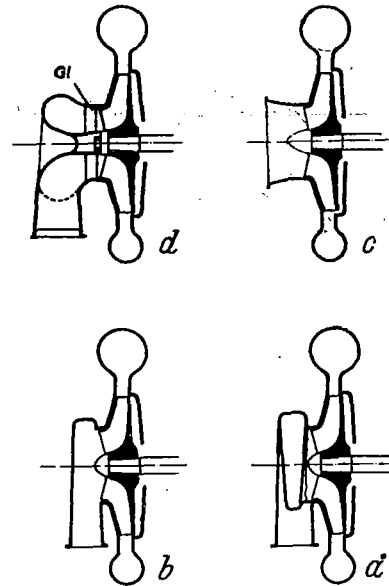
Figure 15.- Common forms of inlet housings.
