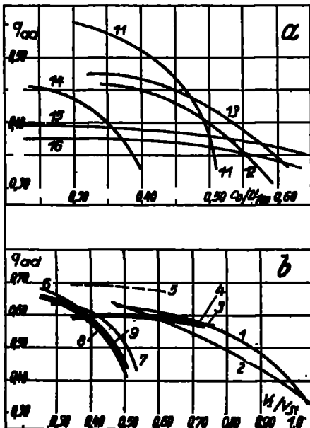
Figure 21.- Values of q_{ad} found for a large number of superchargers investigated.
