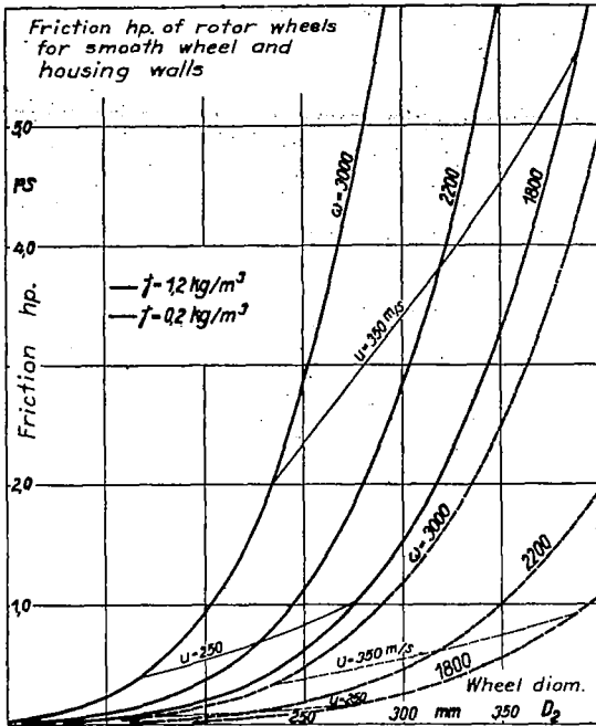
Figure 13.- Friction hp. of impellers for different air densities in the casing and different values of w .
