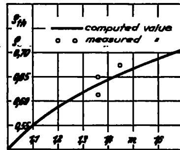
Figure 23.-Computed and measured values for \rho .
