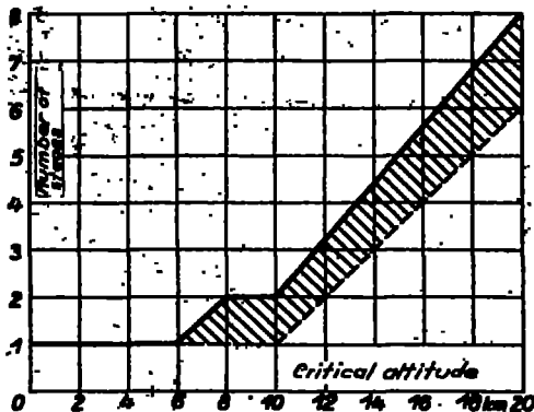
Figure 19.- Number of stages of multi-stage superchargers for critical altitudes up to 20 km. (12.4 mi.) ----- Lower limit for present state of development.
