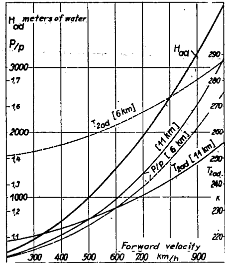
Figure 3.-Variation of delivery heads, pressure ratios, and temperatures with velocity of flight for zero losses, adiabatic compression.
