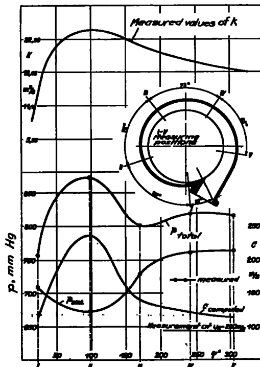
Figure 24. Computed values of k and measured pressures and velocities in a supercharger spiral.
