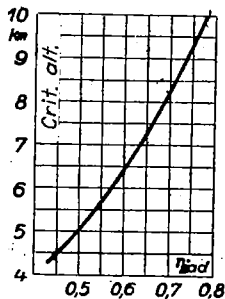
Figure 2.-Critical altitude attainable without intercooling as a function of the internal adiabatic supercharger efficiency \eta_{ad} (Admissible assumed supercharger temperature 80^\circ ).
