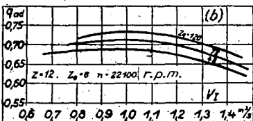
Figure 11b.- Figures of merit for different numbers of intermediate radial blades z_a at rotor wheel exit.
