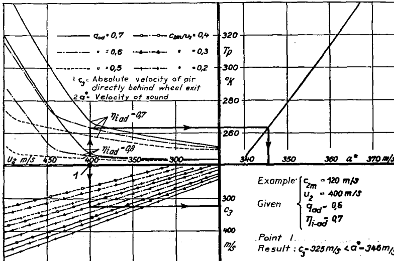
Figure 14.- Computed relations between the peripheral velocity of wheel, absolute velocity of air at rotor wheel exit and velocity of sound for various air temperatures at exit. (The computation is based on measured values of temperatures and pressures. The inlet temperatures correspond to the peripheral velocity and figure of merit of corresponding critical altitude).
