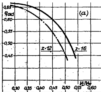
Figure 11a.- Figures of merit for different numbers of blades for same supercharger dimensions.
