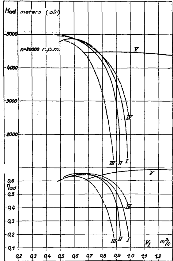
Figure 10.- Effect of form of exit on characteristics of superchargers. Curves I-IV correspond to four different forms of guide vanes. Curve V was obtained with vanes removed. i.e. with smooth guide ring.
