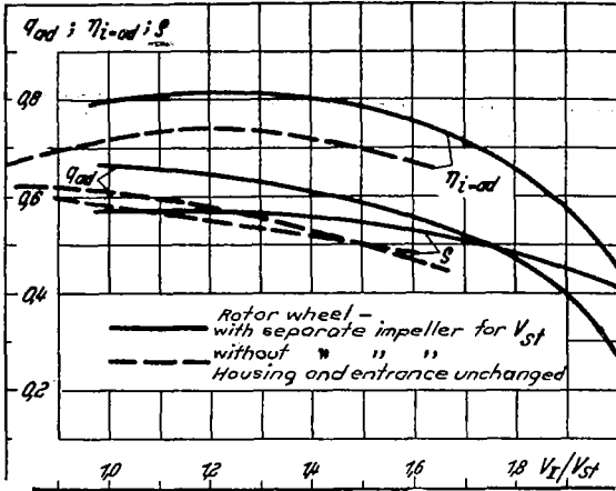
Figure 9.- Improvement in characteristics of a wheel with radial blades by separately added impeller (fig.6).
