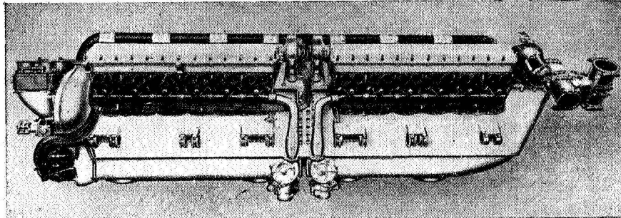
Figure 7.- Flat AS 6 engine.
