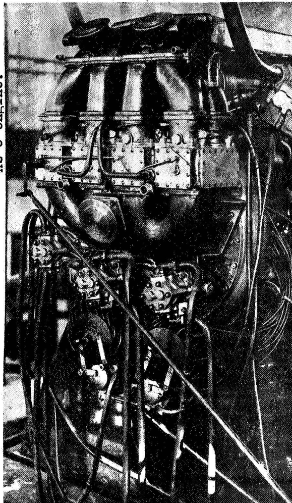
Figure 12.- Carburetors and fuel pumps. AS 6 engine.
