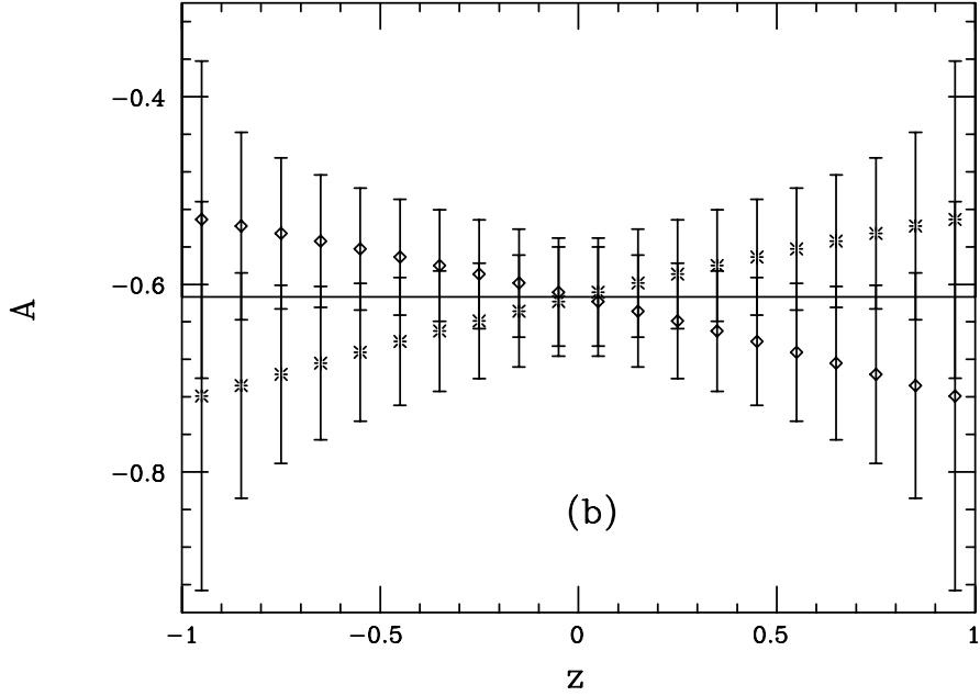
Figure 3: Same as the previous figure but now for a \tilde{\mu}_R .
