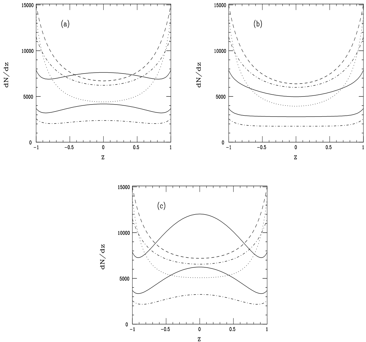
Figure 7: Un-binned angular distribution as in the previous figure but now broken down into the various helicity contributions. A stop mass of 250 GeV has been assumed along with an integrated luminosity of 200 \text{ fb}^{-1} and a collider center of mass energy of 1 TeV. (a) is the MSSM while (b) and (c) are the results including graviton exchange with \lambda = \pm 1 with M_s = 2 TeV. In all panels, the helicities are as follows: (++++) is the upper dash-dotted curve, (+++-) is the dashed curve, (+ + - -) is the lower dash-dotted curve, (+ - + -) is the dotted curve, (- + + -) is the upper solid curve and (+ - - -) is the lower solid curve.
