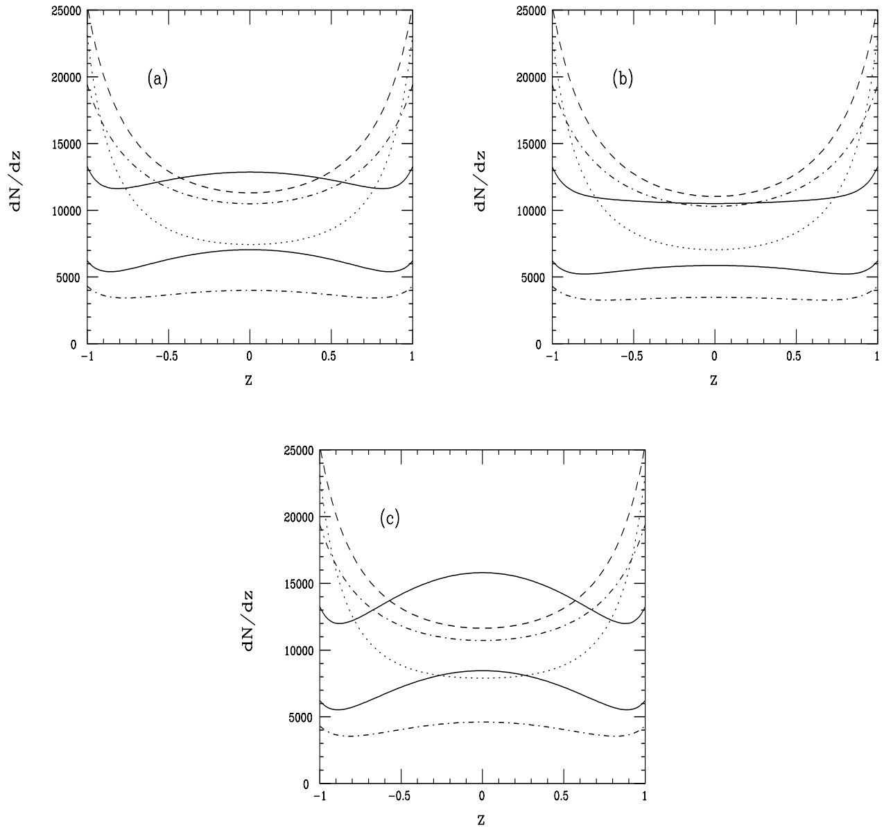
Figure 9: Same as Fig.7 but now for either H^- or \tilde{\ell} pair production by polarized photons.
