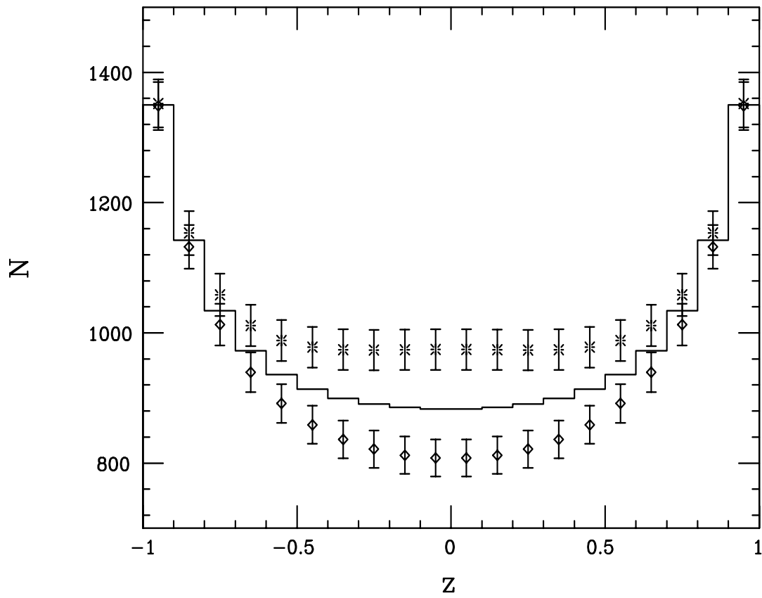
Figure 8: Same as Fig.6 but now for either H^- or \tilde{\ell} pair production by unpolarized photons.
