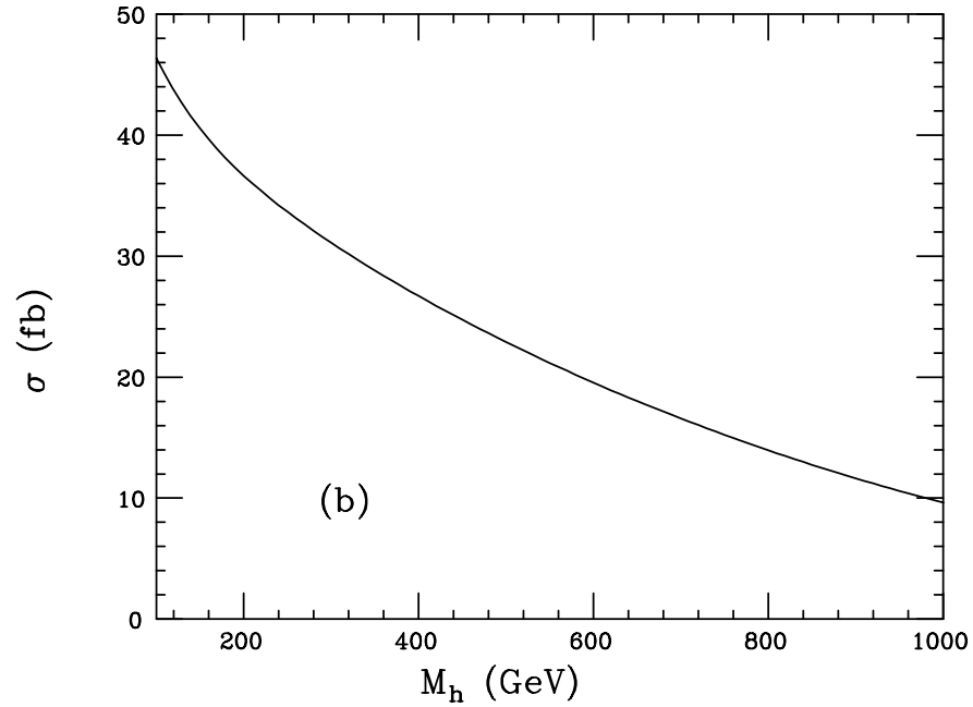
Figure 12: Leading order production cross sections for Higgs boson pairs at (a) TeV II or (b) the LHC as a function of the Higgs boson mass at the tree level due to the exchange of a Kaluza-Klein tower of gravitons. We assume that M_s = 1(3) TeV for the case of the Tevatron(LHC).
