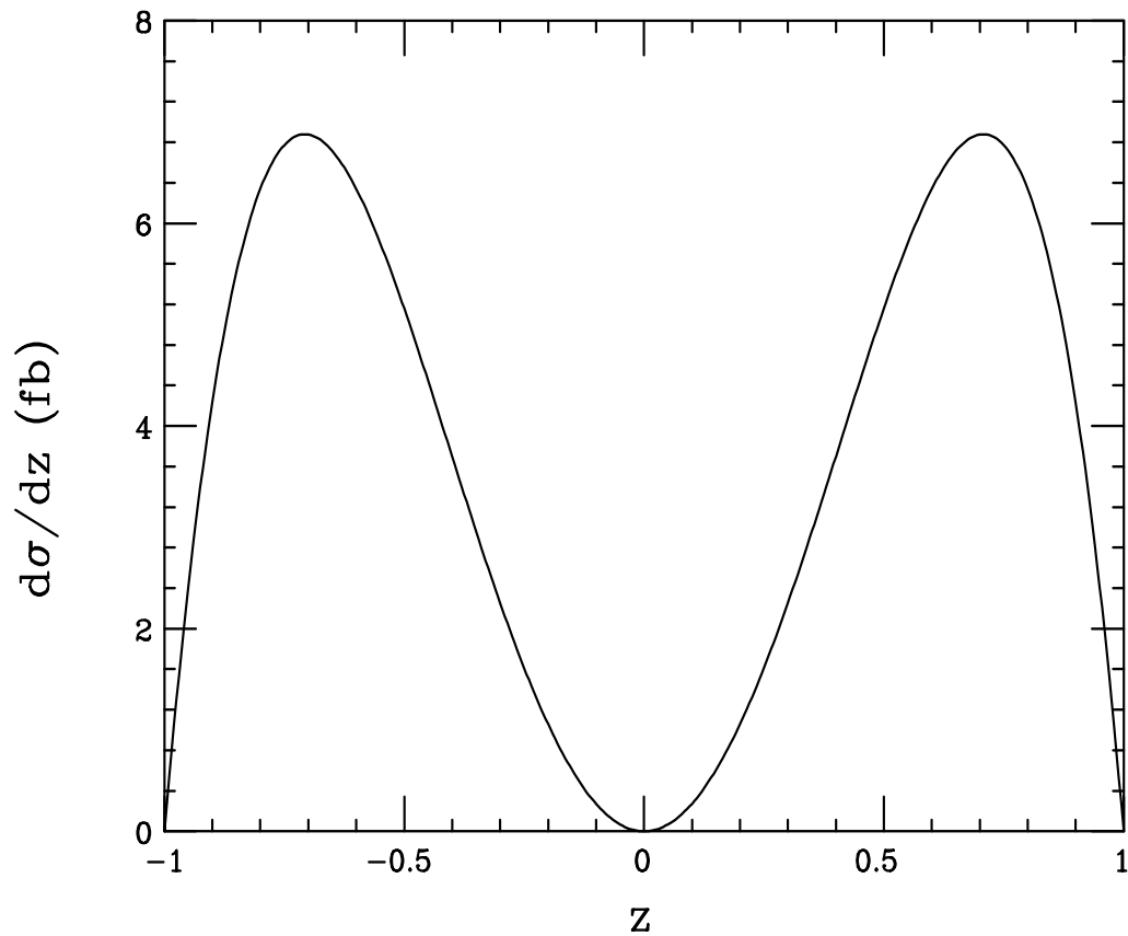
Figure 5: The tree level unpolarized differential cross section for e^+e^- \rightarrow 2h^0 at a 500 GeV e^+e^- linear collider due to the exchange of a Kaluza-Klein tower of gravitons assuming m_h = 130 GeV and M_s = 1 TeV. Note the canonical shape arising from the nature of the spin-2 exchange.
