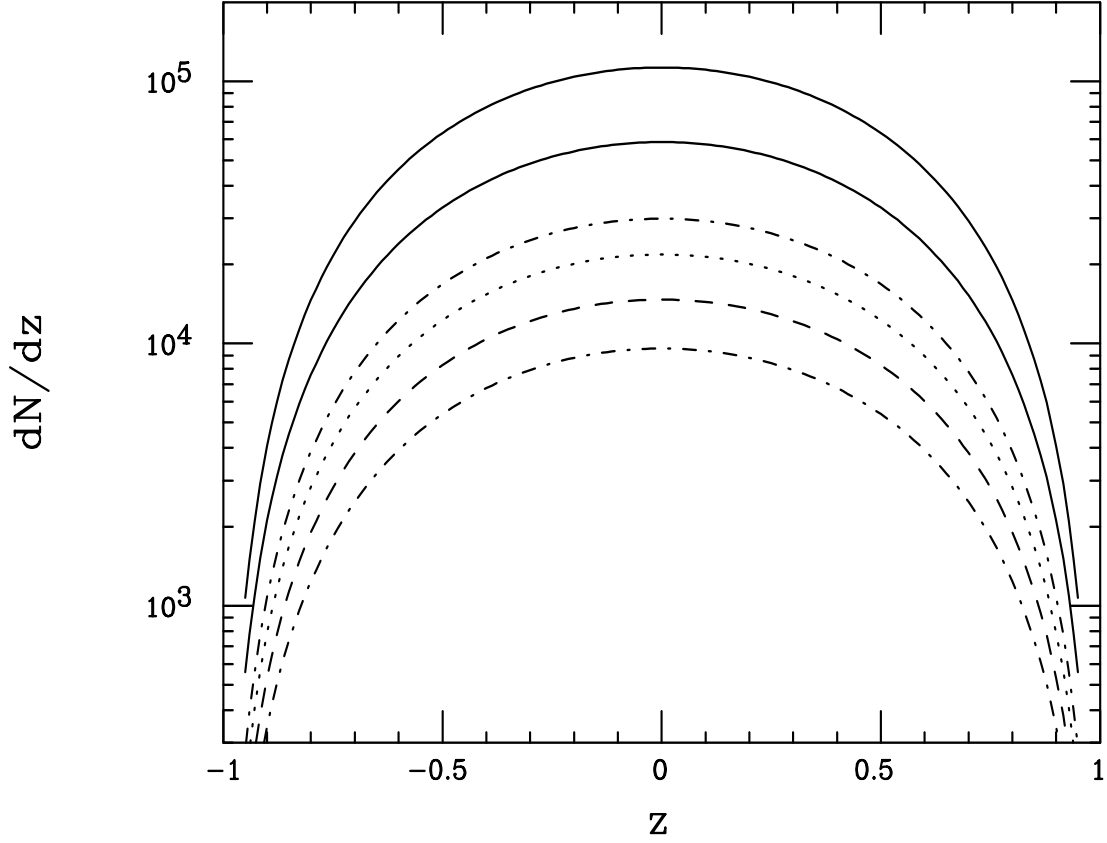
Figure 11: Un-binned angular distribution for the process \gamma\gamma \rightarrow 2h^0 using polarized beams for the same parameter choice as in the previous figure. From top to bottom the polarization parameter choices are given by (- + + -) , (+ - - -) , (+ + - -) , (+ - + -) , (+ + + -) and (+ + + +) , respectively.
