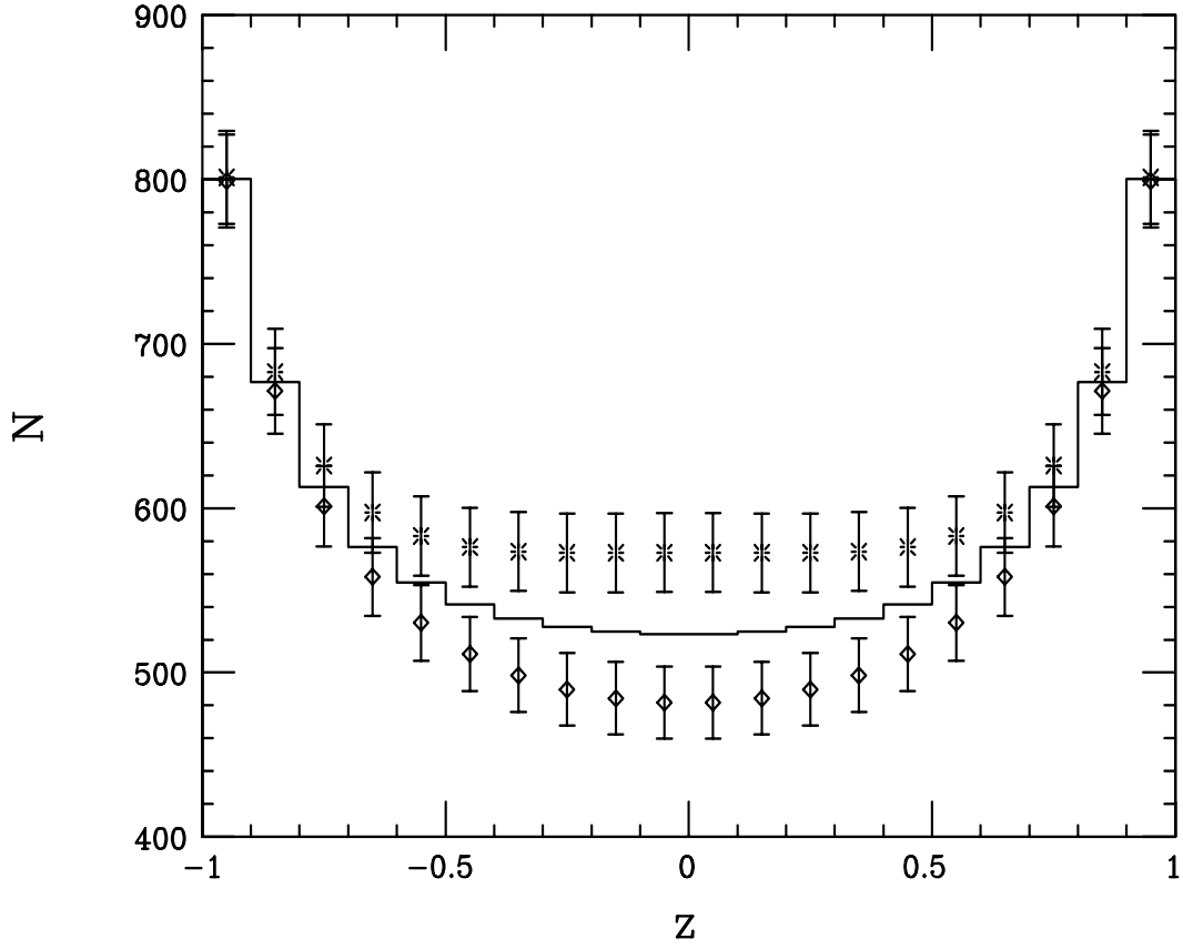
Figure 6: Binned angular distribution for stop pairs produced in unpolarized \gamma\gamma collisions assuming an e^+e^- center of mass energy of 1 TeV for a stop mass of 250 GeV and an integrated luminosity of 200 fb^{-1} . The histogram shows the result in the MSSM while the two sets of ‘data’ are the predictions including the exchange of a tower of K-K gravitons with \lambda = \pm 1 and M_s = 2.5 TeV. The errors shown are statistical only.
