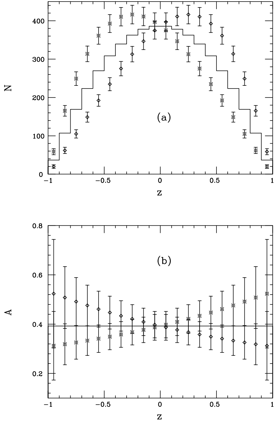
Figure 1: (a) Cross section and (b) A_{LR} for \tilde{t} production at a 500 GeV e^+e^- collider assuming m_{\tilde{t}} = 150 GeV and an integrated luminosity of 100 \text{ fb}^{-1} . The stop is assumed to be maximally mixed, i.e. , \theta_{\tilde{t}} = 45^\circ . The histogram (solid line) shows the MSSM expectations while the two sets of data points include the contributions from a K-K tower of gravitons with M_s = 1.5 TeV and reflect the anticipated measurement errors.
