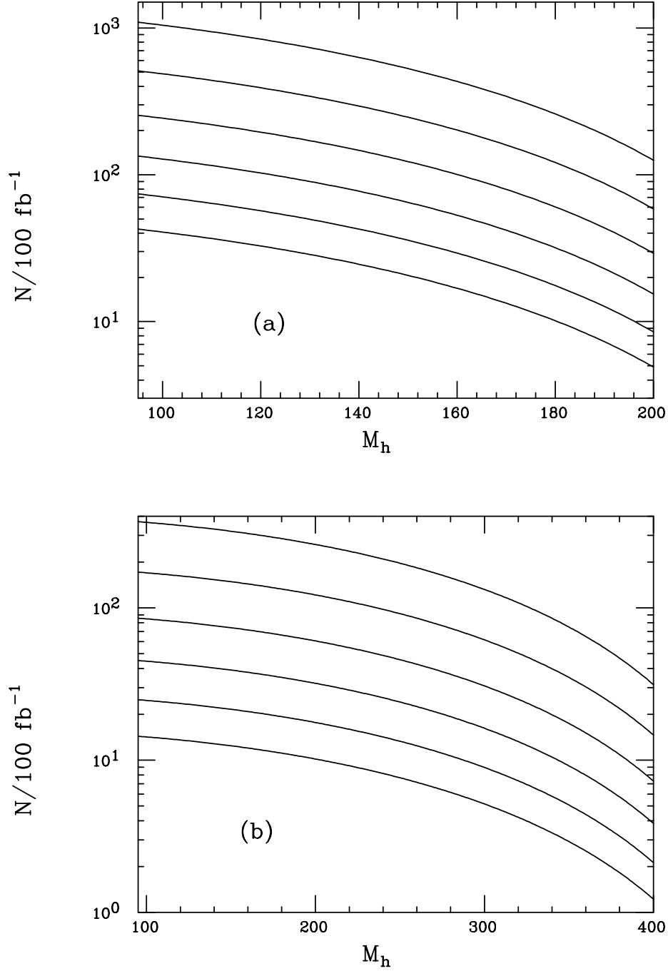
Figure 4: Tree level production rate for Higgs boson pairs due to graviton tower exchange at a (a) 500 GeV or a (b) 1 TeV e^+e^- collider as a function of the Higgs mass scaled to an integrated luminosity of 100 \text{ fb}^{-1} . From top to bottom in (a)[(b)] the curves correspond to the choice M_s = 1[2] TeV increasing in steps of 0.1[0.2] TeV.
