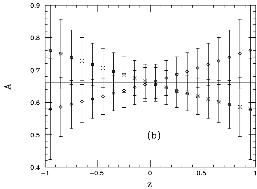
Figure 2: Same as the previous figure but now for either a \tilde{\mu}_L or a charged Higgs boson, H^\pm . Note that the slope of A_{LR} in this case is opposite to that for \tilde{\mu}_L or H^\pm .
