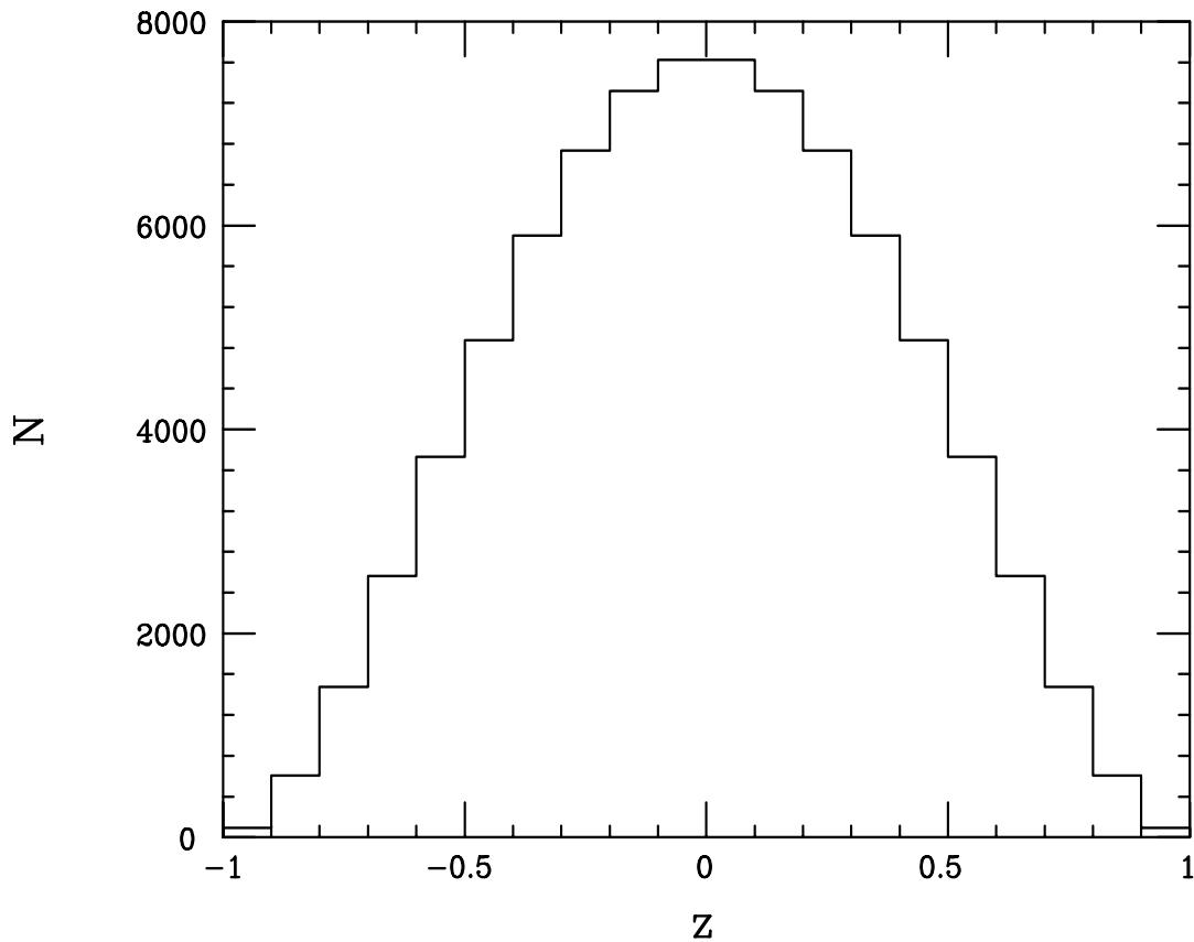
Figure 10: Binned angular distribution for Higgs boson pair production in unpolarized \gamma\gamma collisions at a 1 TeV e^+e^- assuming m_h = 130 GeV, M_s = 1 TeV and an integrated luminosity of 200 \text{ fb}^{-1} .
