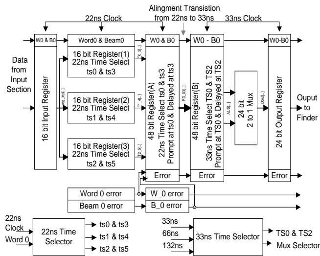
Figure 6: Alignment FPGA Block Diagram.
