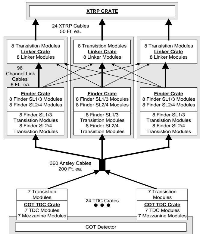
Figure 1: XFT System Diagram.
