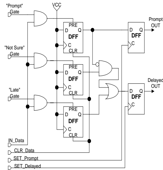
Figure 3: Mezzanine module Prompt & Delayed Logic.
