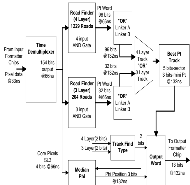
Figure 10: Linker CPLD Block Diagram.
