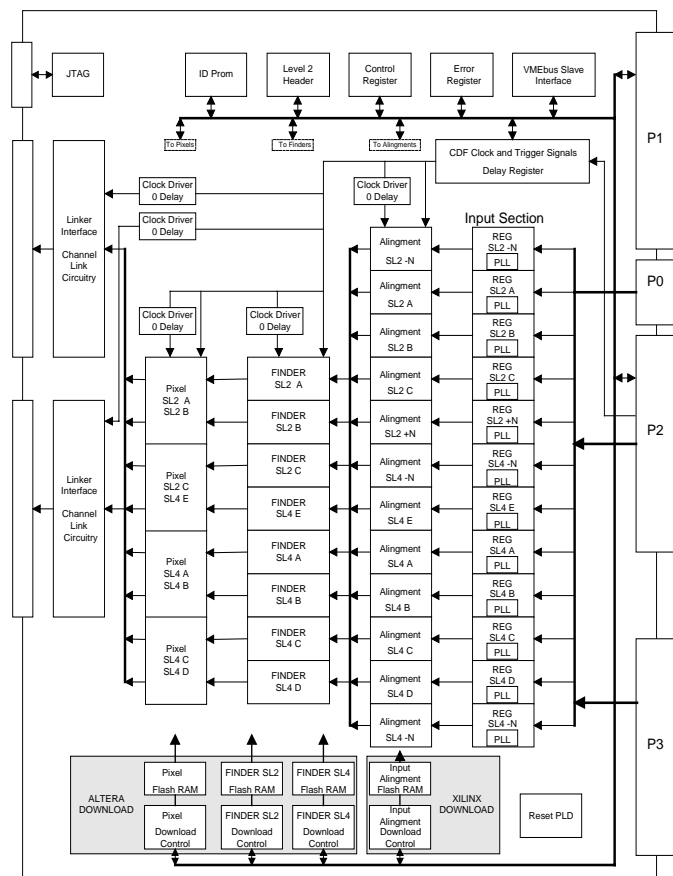
Figure 5: Finder SL24 Module Block Diagram.
