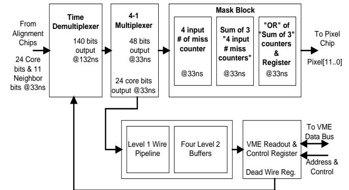
Figure 7: Finder CPLD Block Diagram.
