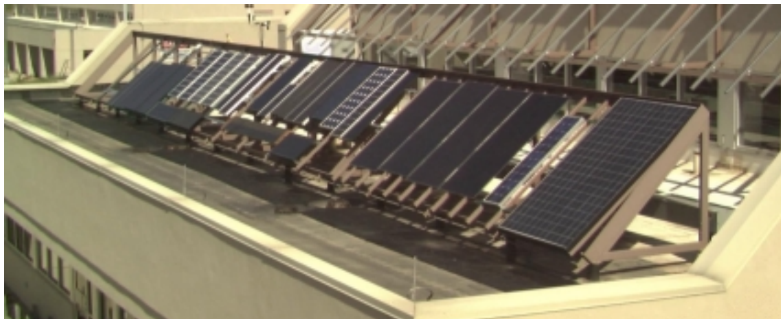
Figure 4-1. PV Modules on the PERT Rack at NREL's Outdoor Test Facility.
