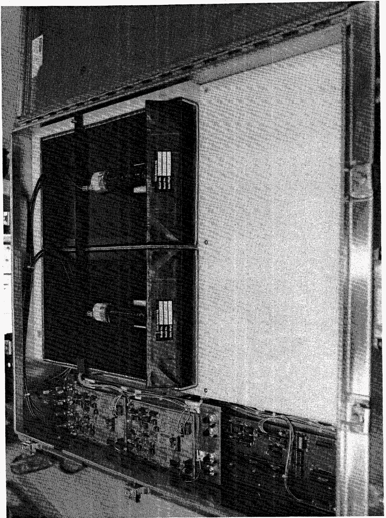
Figure 1. Plastic scintillation detectors inside stainless steel box of GNM.
