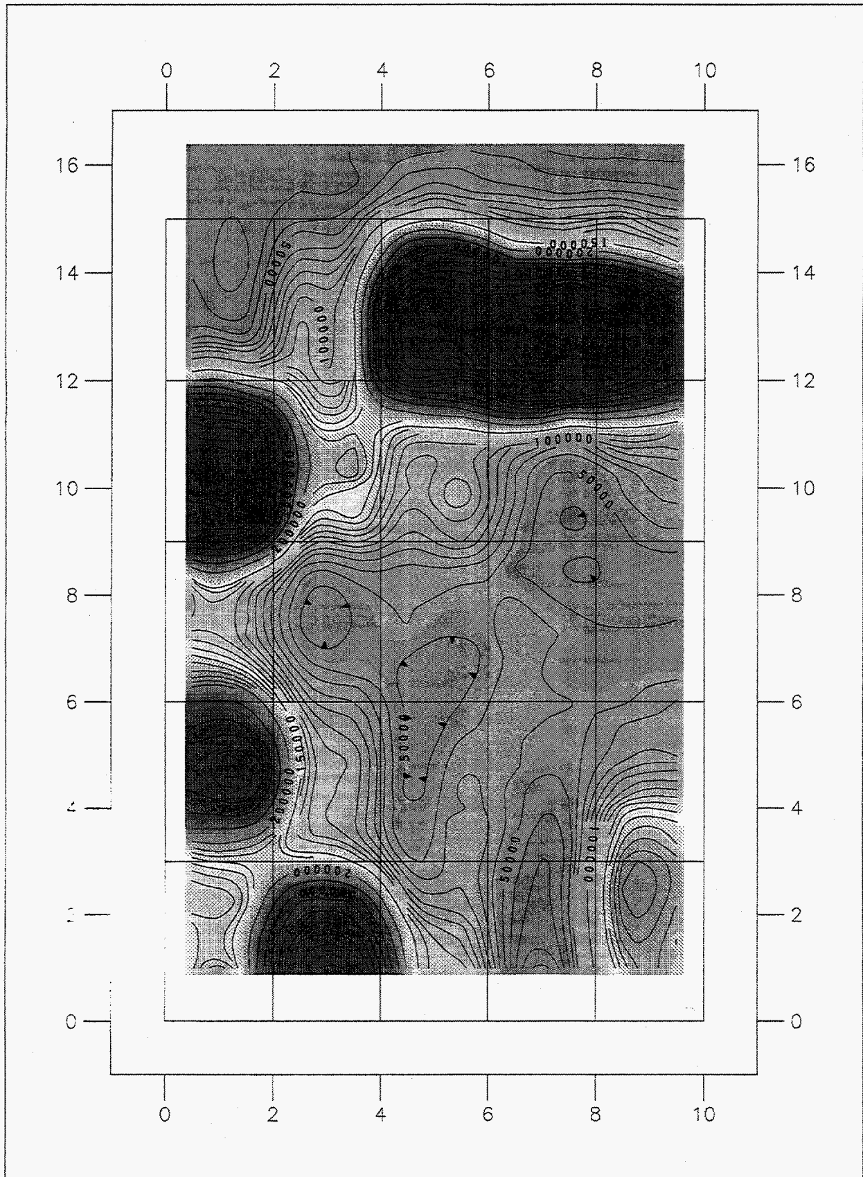
Figure 6. Contour plot of the \gamma -ray count rates from experiment 2 of the 25-drum matrix acquired at a standoff distance of 15.2 cm and a scan speed of 7.5 cm/s.
