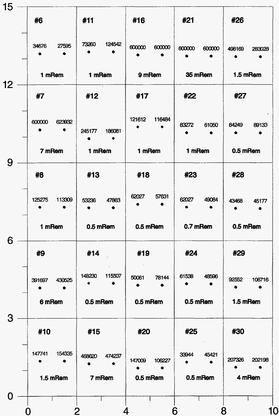
Figure 5. Outline of 25-drum test matrix with static gamma-ray and neutron measurements.
