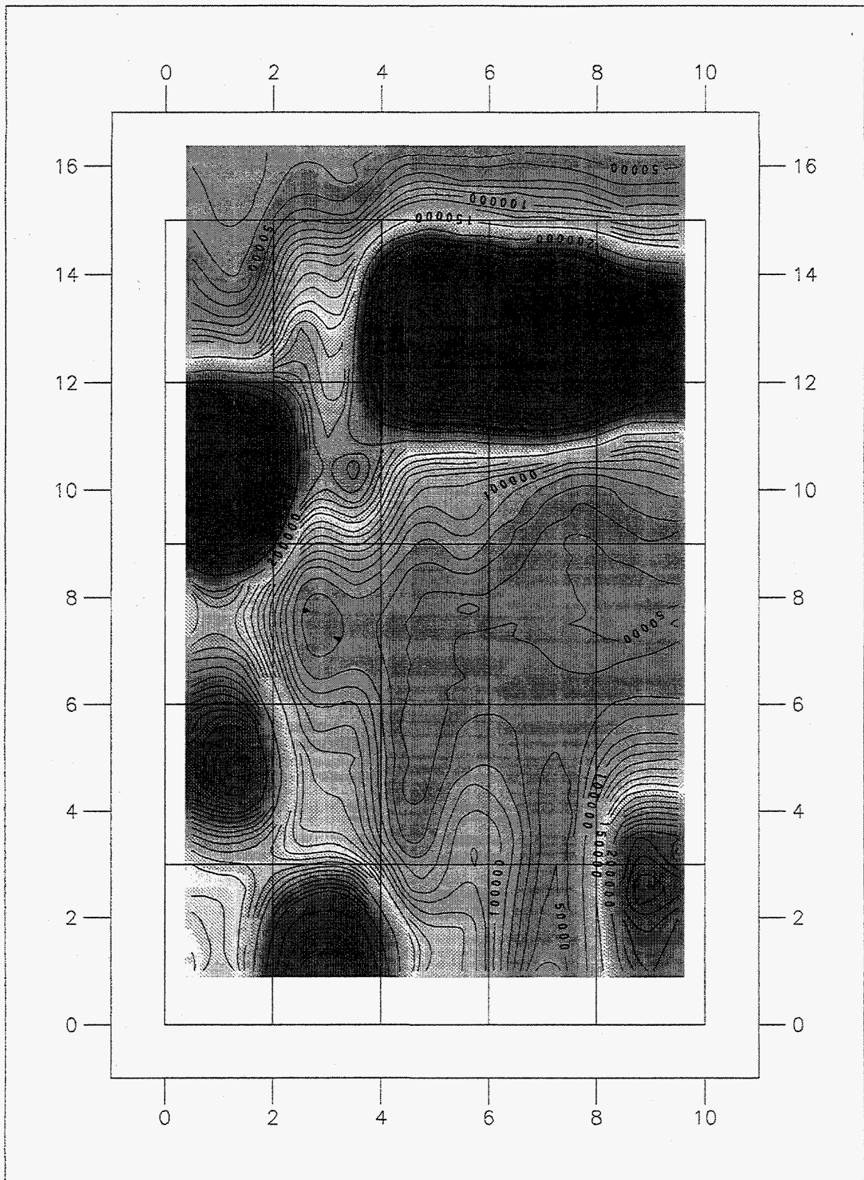
Figure 10. Contour plot of the \gamma -ray count rates from experiment 4 of the 25-drum matrix acquired at a standoff distance of 45.7 cm and a scan speed of 7.5 cm/s.
