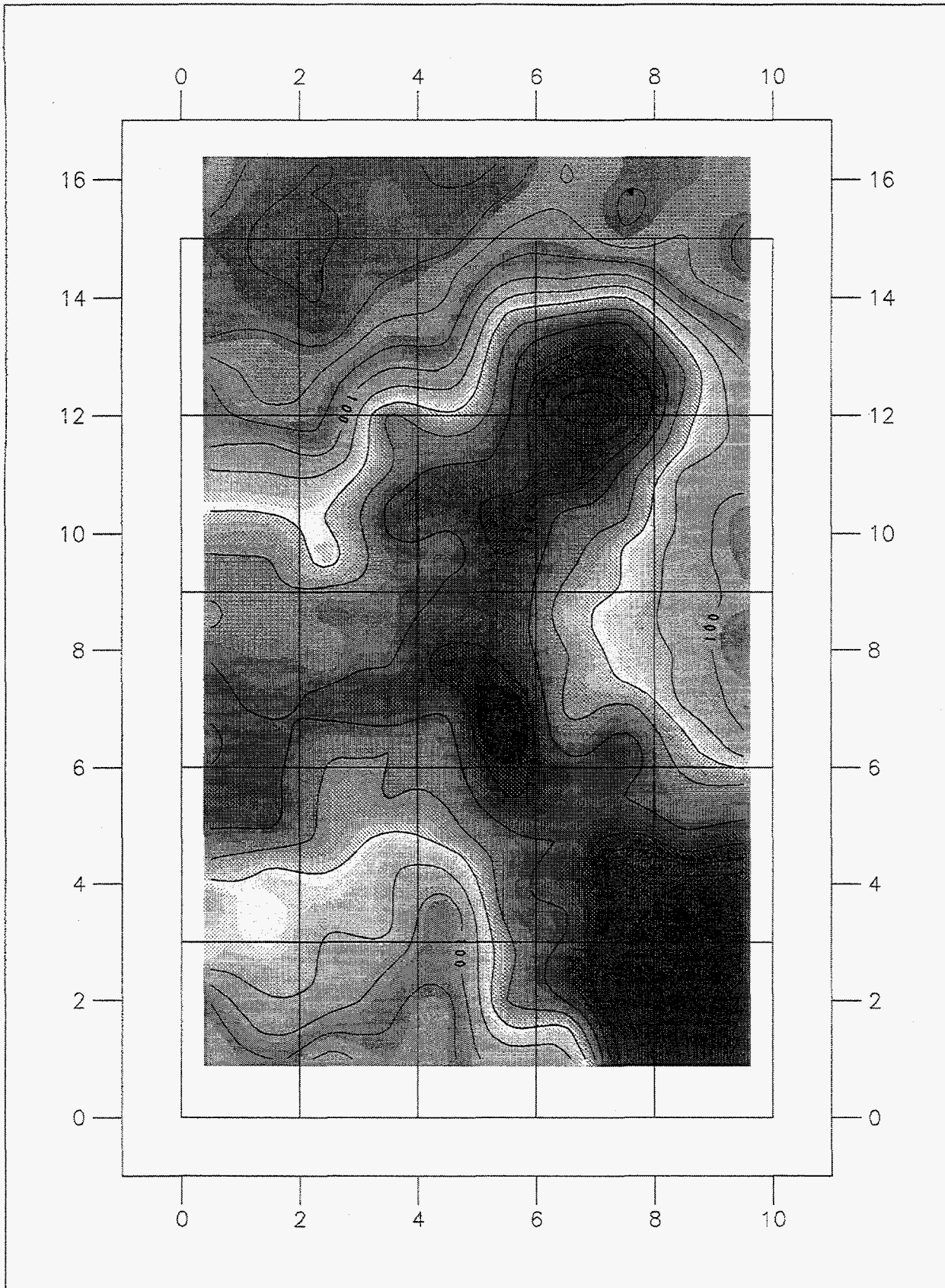
Figure 11. Contour plot of the neutron count rates from experiment 4 of the 25-drum matrix acquired at a standoff distance of 45.7 cm and a scan speed of 7.5 cm/s.
