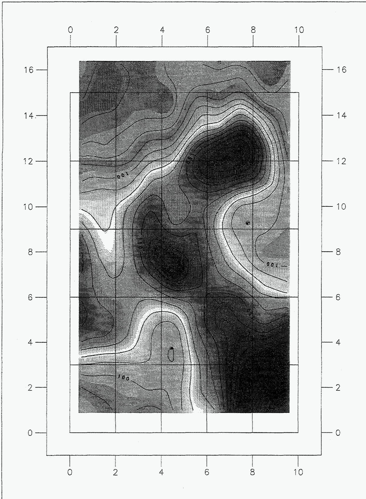
Figure 9. Contour plot of the neutron count rates from experiment 3 of the 25-drum matrix acquired at a standoff distance of 15.2 cm and a scan speed of 15 cm/s.
