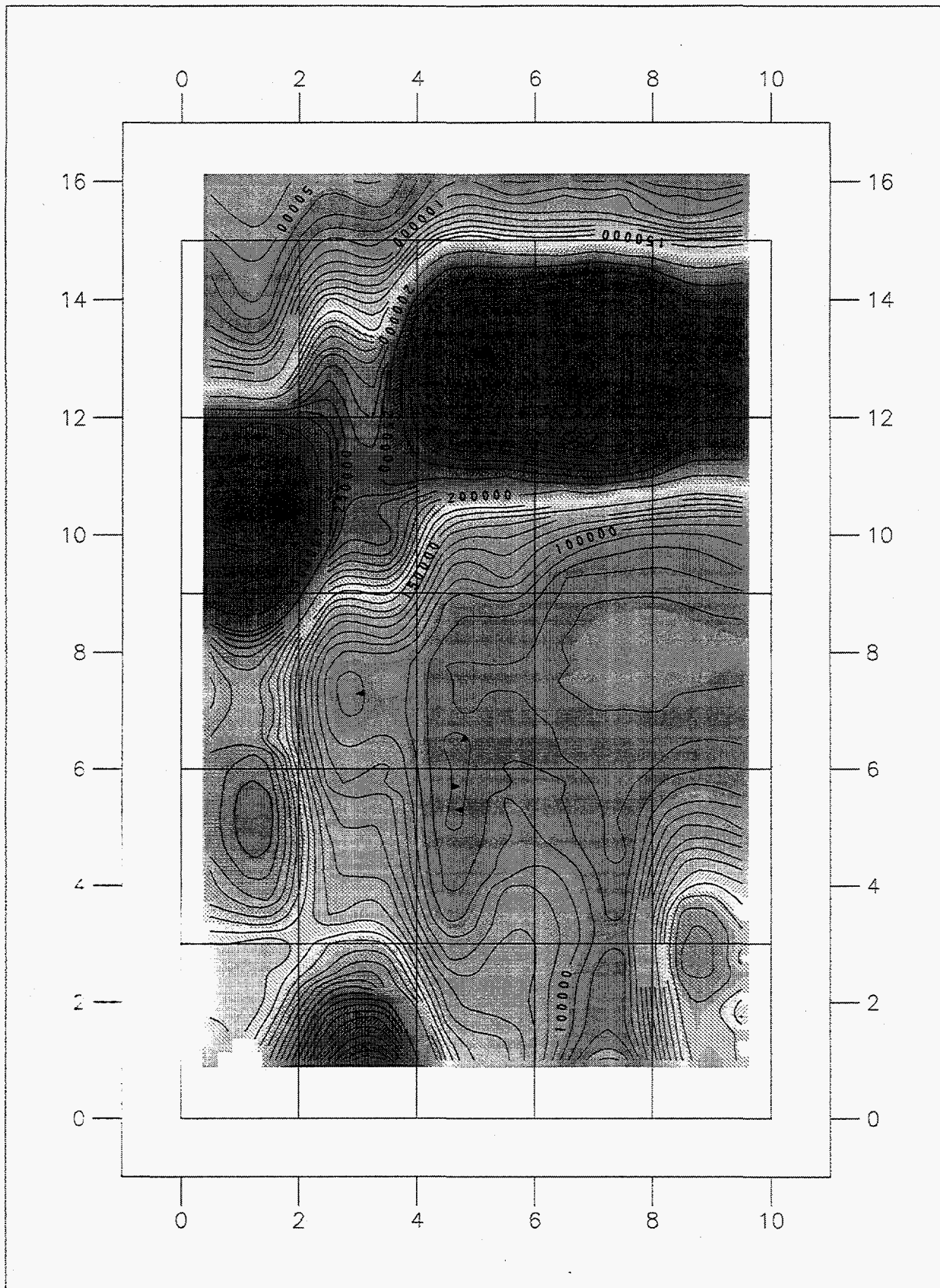
Figure 12. Contour plot of the \gamma -ray count rates from experiment 5 of the 25-drum matrix acquired at a standoff distance of 30.5 cm and a scan speed of 7.5 cm/s.
