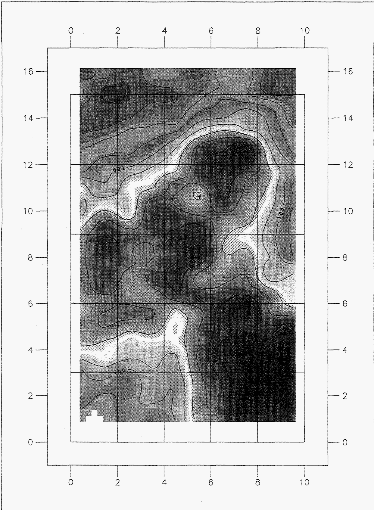
Figure 13. Contour plot of the neutron count rates from experiment 5 of the 25-drum matrix acquired at a standoff distance of 30.5 cm and a scan speed of 7.5 cm/s.
