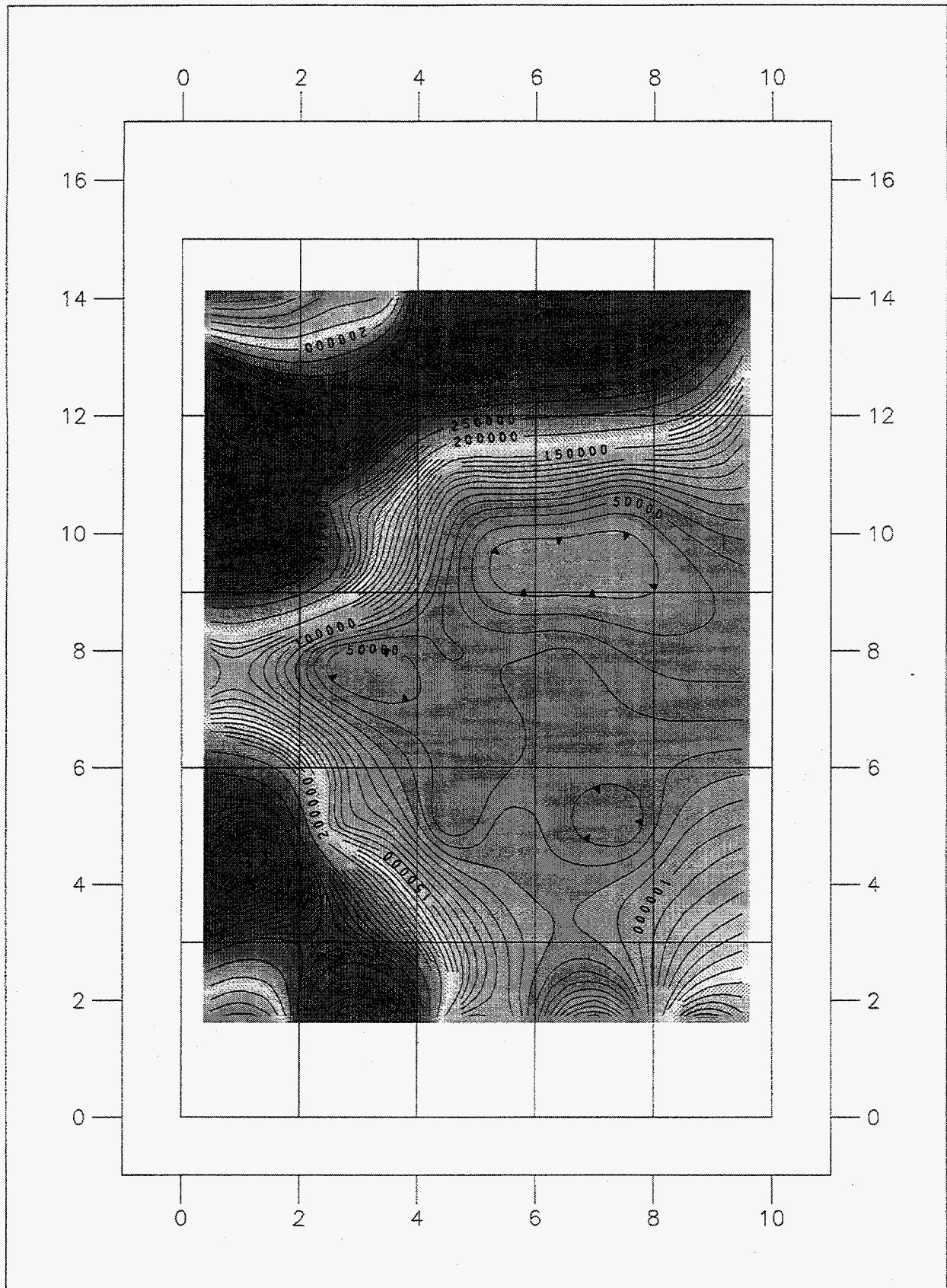
Figure 16. Horizontal scan of \gamma -ray count rates from experiment 7. Scan was across all five stacks at a height of 110 cm (center of second row of drums from the bottom), at a standoff distance of 30.5 cm, and a scan speed of 6.1 cm/s.
