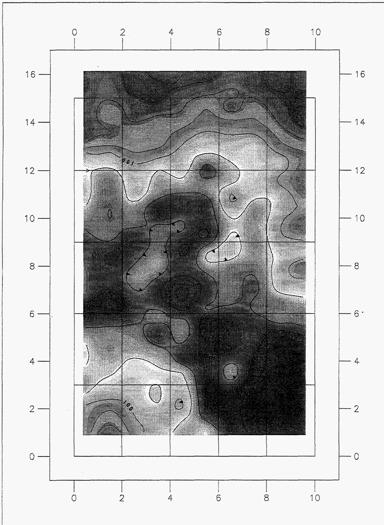
Figure 15. Contour plot of the neutron count rates from experiment 6 of the 25-drum matrix acquired at a standoff distance of 91.4 cm and a scan speed of 7.5 cm/s.
