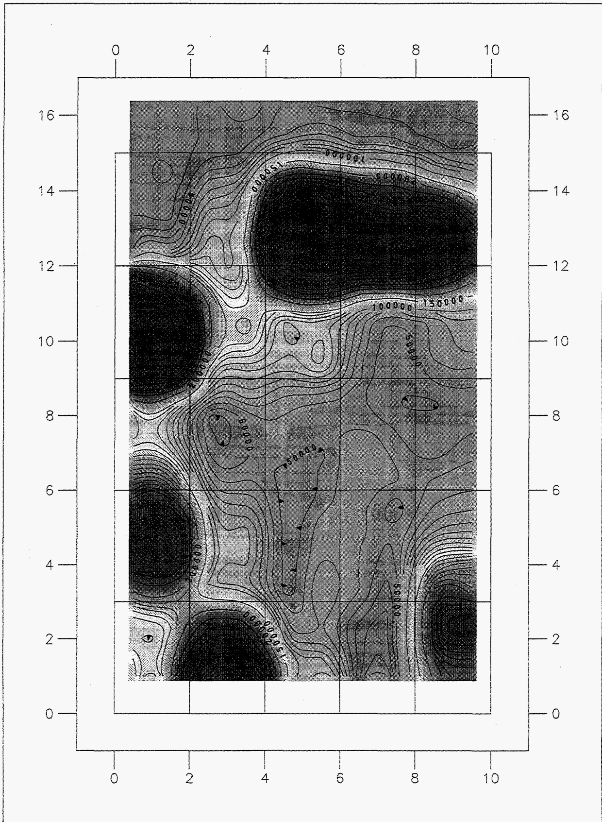
Figure 8. Contour plot of the \gamma -ray count rates from experiment 3 of the 25-drum matrix acquired at a standoff distance of 15.2 cm and a scan speed of 15 cm/s.
