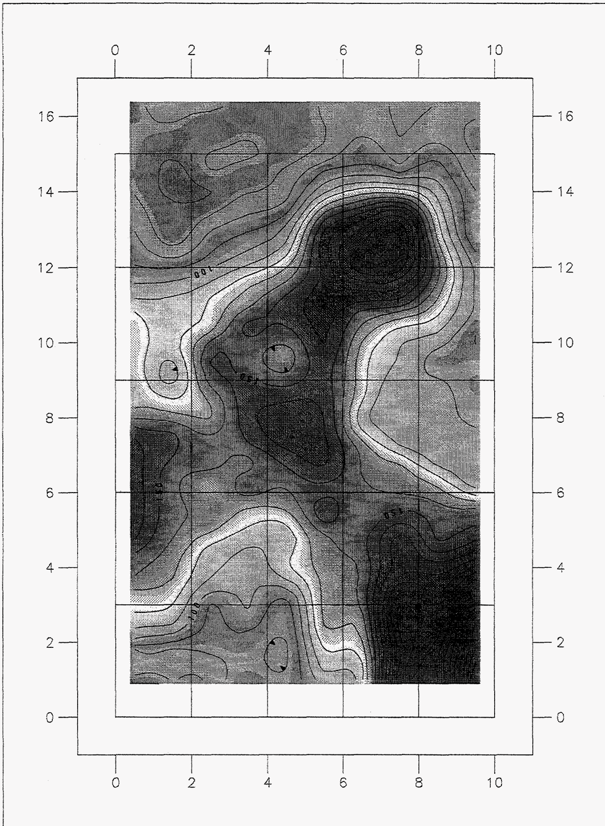
Figure 7. Contour plot of the neutron count rates from experiment 2 of the 25-drum matrix acquired at a standoff distance of 15.2 cm and a scan speed of 7.5 cm/s.
