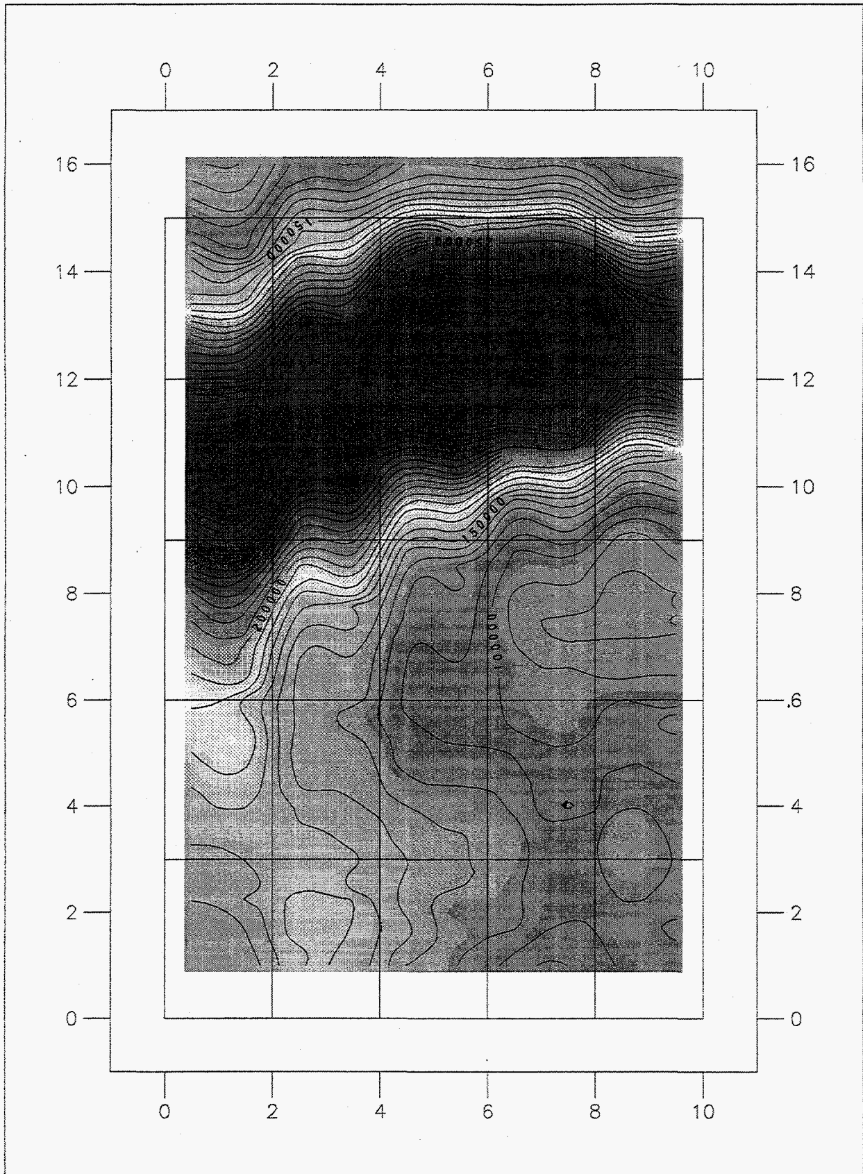
Figure 14. Contour plot of the \gamma -ray count rates from experiment 6 of the 25-drum matrix acquired at a standoff distance of 91.4 cm and a scan speed of 7.5 cm/s.
