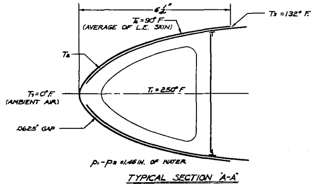
FIGURE 30- RESULTS OF DESIGN ANALYSIS FOR FIN & DORSAL - B-17E AIRPLANE
