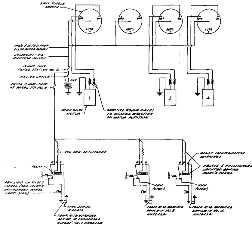
WIRING DIAGRAM
