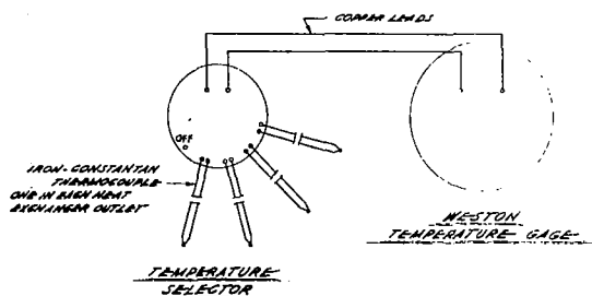
Figure 25.- Instrumentation and control for B-17F thermal ice-prevention system.
