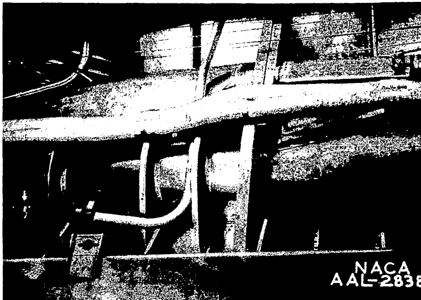
Figure 23.- Heated-air outlet and dump valve for exchanger installed in right inboard nacelle, B-17F airplane.
