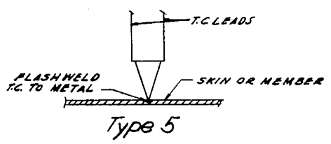
Typical thermocouple mounting details - Not to scale Figure 34.- Thermocouple types employed in tests of B-17F thermal ice-prevention system.
