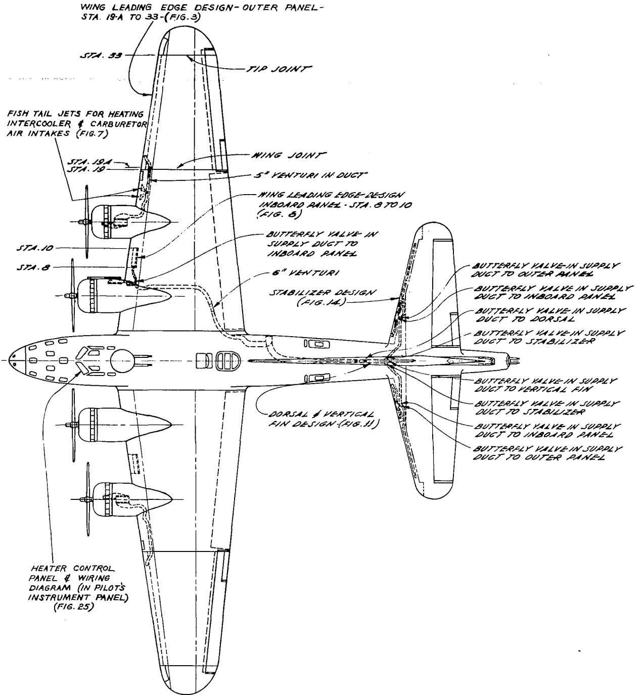
Figure 2.- General view of thermal ice-prevention system, B7F airplane.
