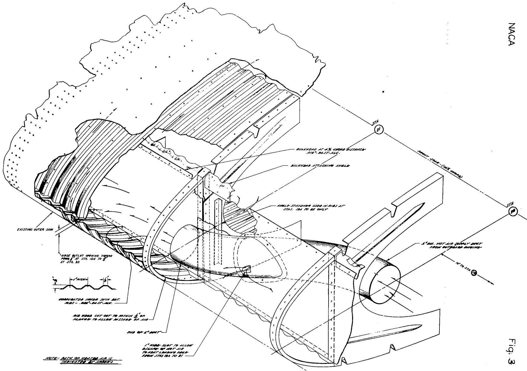
Figure 3.- Details of wing outer-panel leading-edge design for B-17 thermal ice-prevention system.
