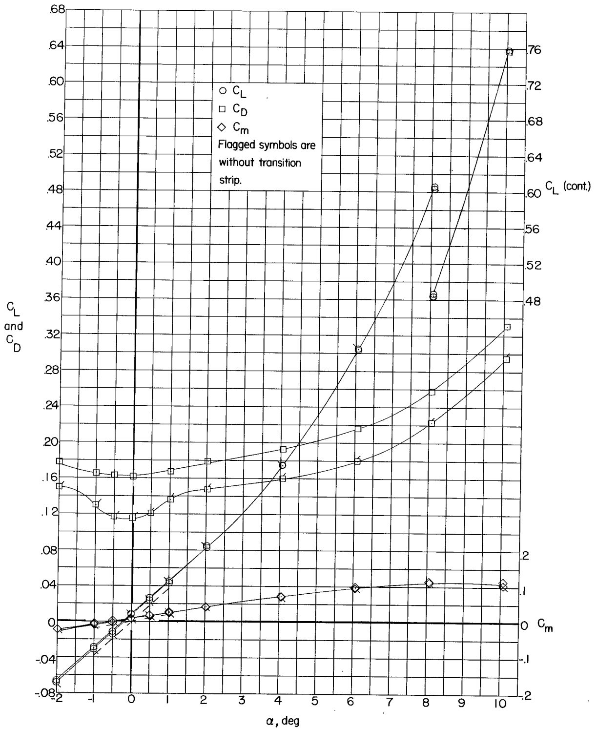
(a) Configuration 1 (basic body).
