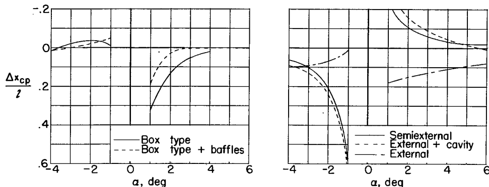
(c) Change in center-of-pressure locations due to addition of bomb to bomb bay.
