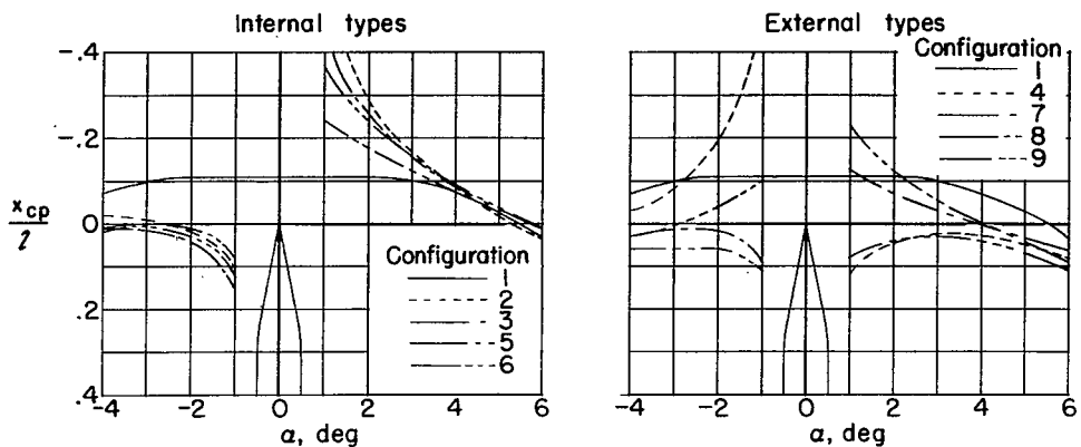
(a) Center-of-pressure locations.
