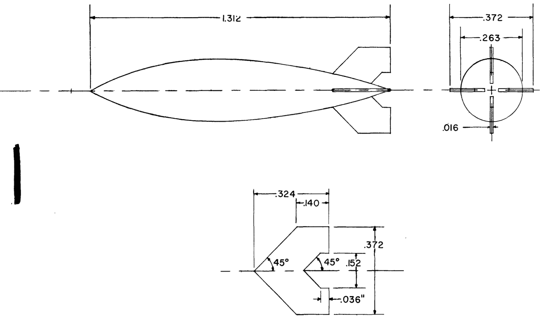
(d) Bomb configuration (maximum diameter at 40 percent length).
