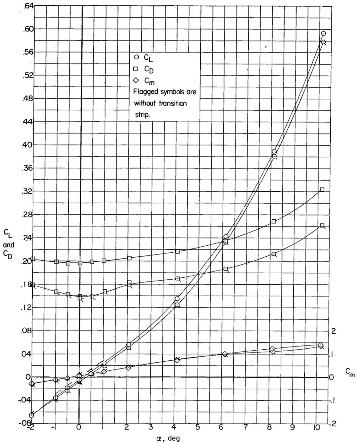
(a) Configuration 1 (basic body).
