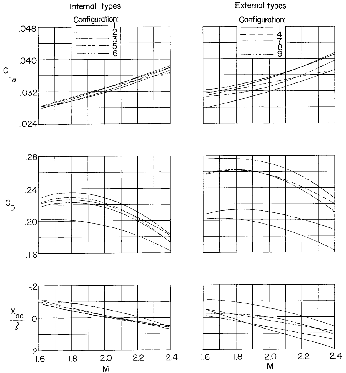
(a) Lift slope, drag, and aerodynamic-center locations.
