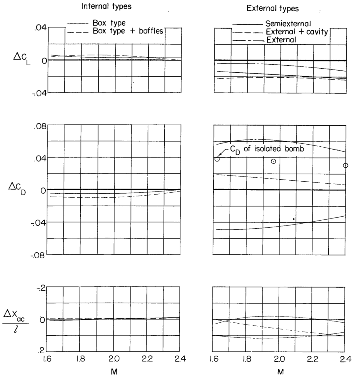
(c) Increments due to addition of bomb to bomb bay.
