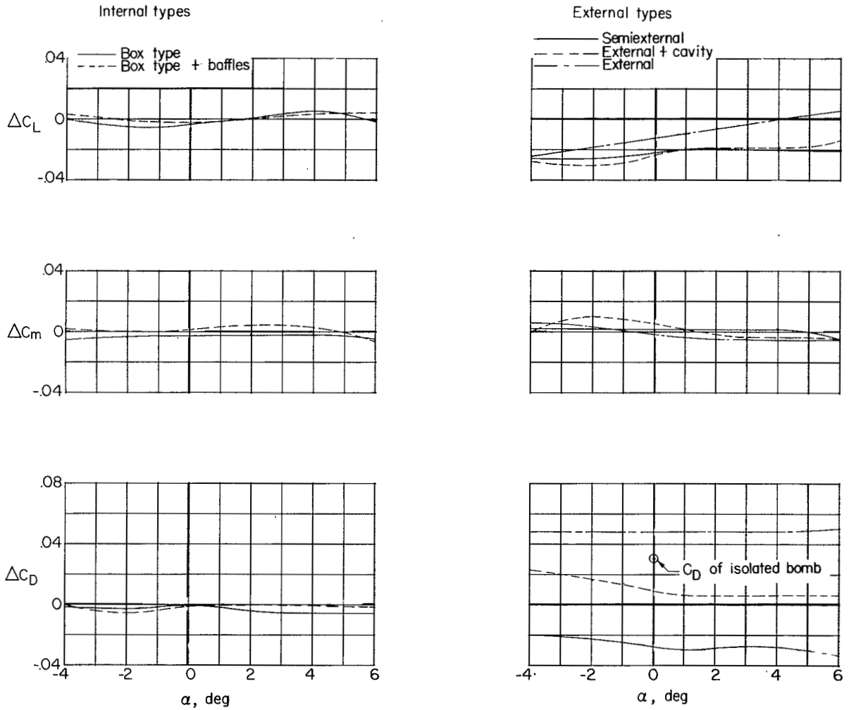
(b) Due to addition of bomb to bomb bay.
