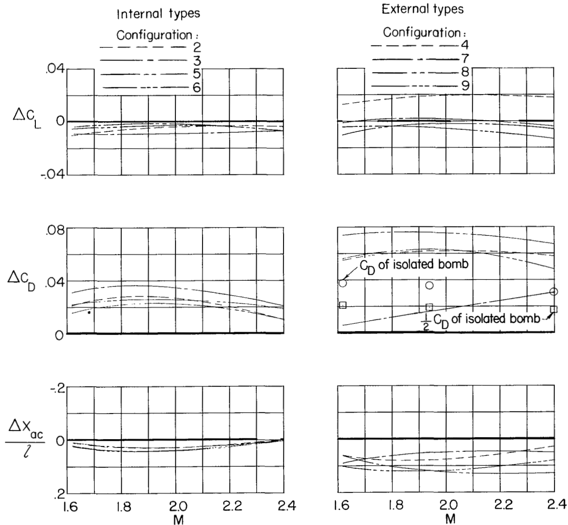
(b) Increments due to installation of bomb bay or bomb plus bomb bay to basic body.
