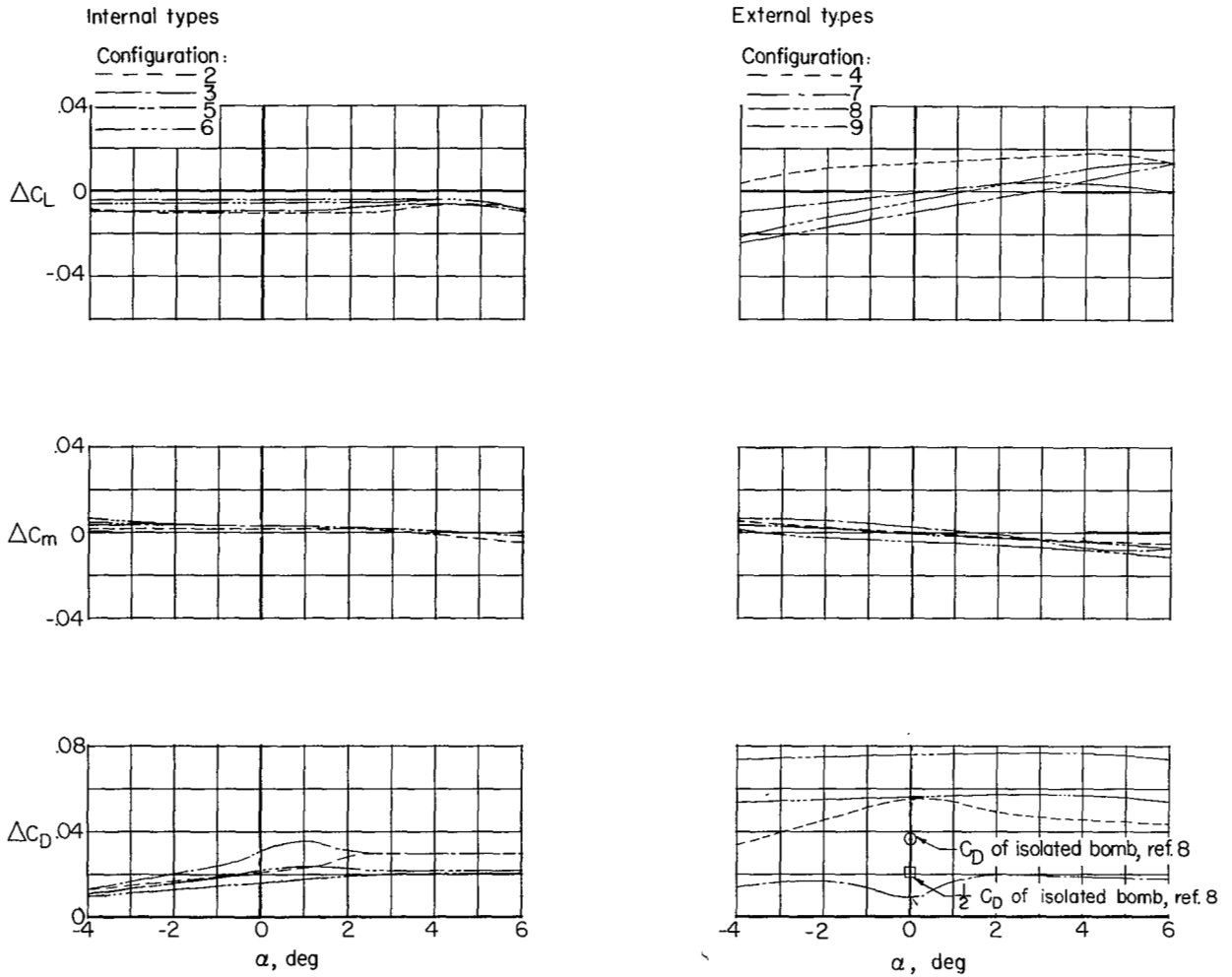
(a) Due to installation of bomb bay or bomb plus bomb bay to basic body.
