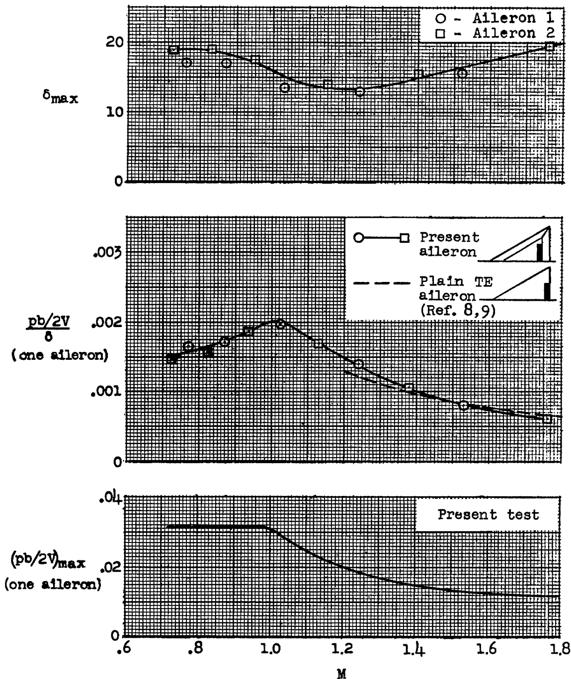
Figure 6.- Variations with Mach number of measured maximum aileron deflection and rolling effectiveness obtained with the bellows-actuated aileron control configuration of the present test, and comparison with other data.
