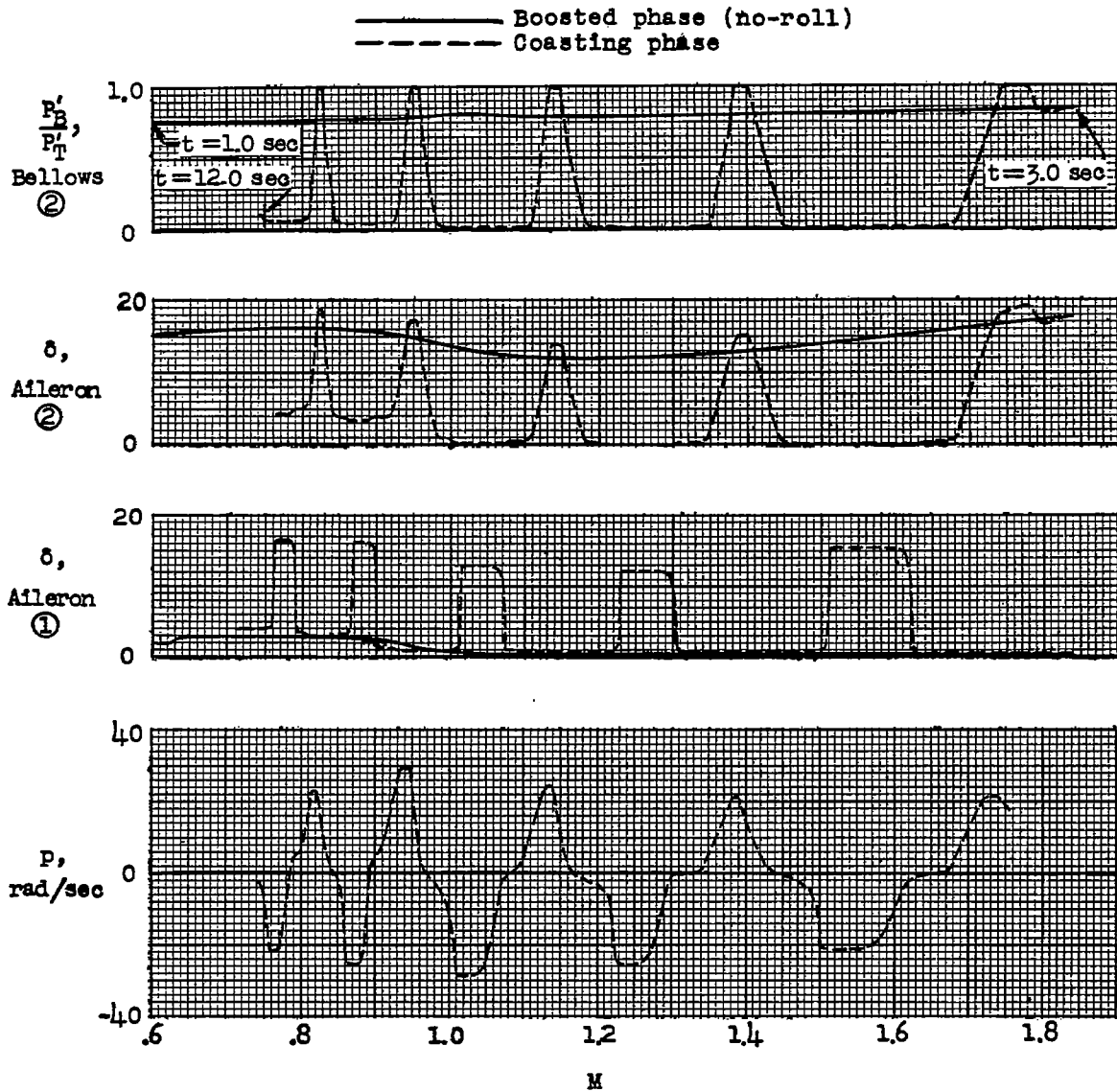
Figure 5.- A flight history, plotted as a function of Mach number, of measured values of bellows pressure in cell (2), aileron deflections, and resulting rolling velocities.
